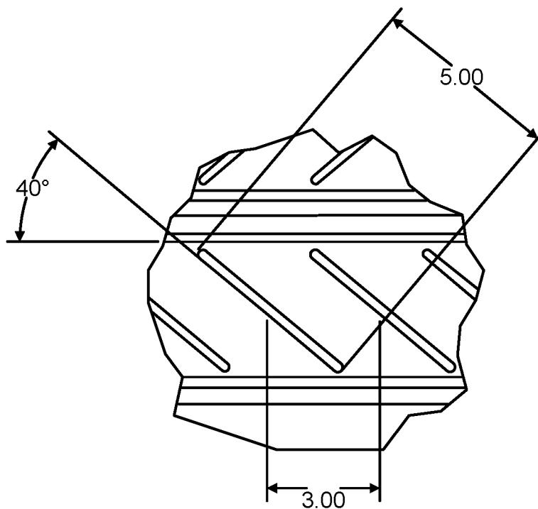
DETAIL A
