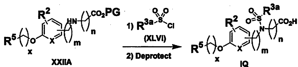
Scheme 16
