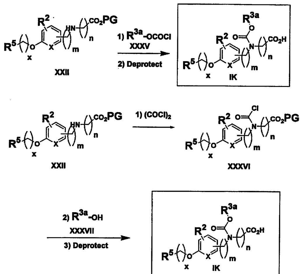
Scheme 11
