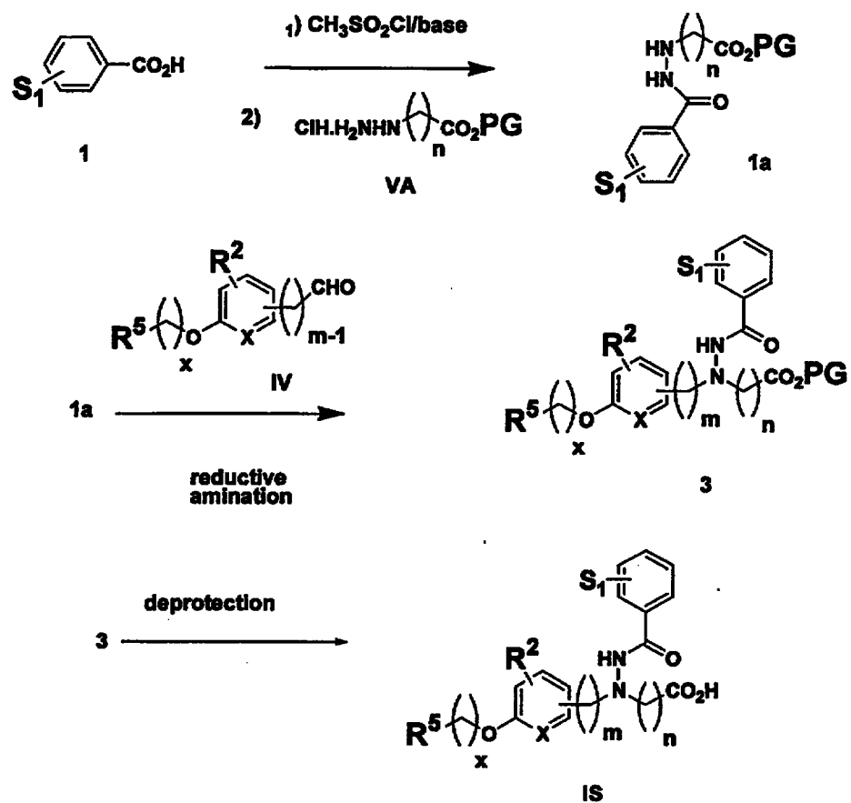
Scheme 18
