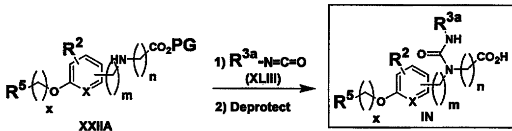
Scheme 13
