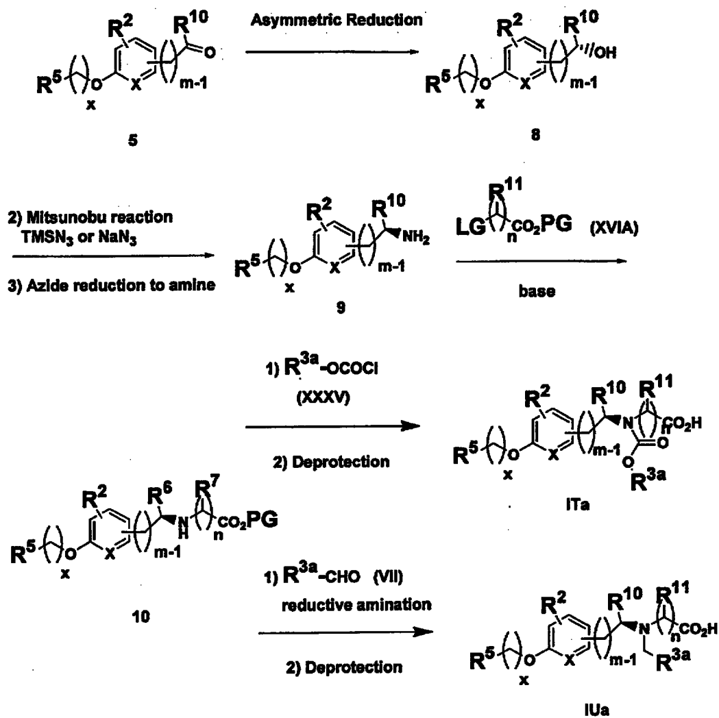
Scheme 21
