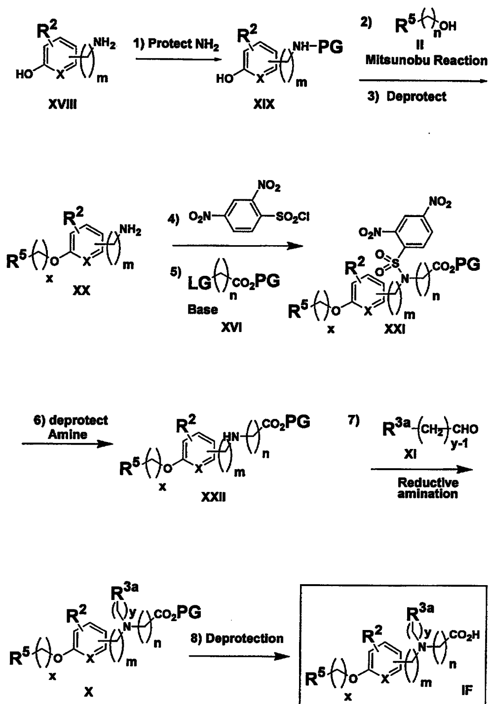
Scheme 6
