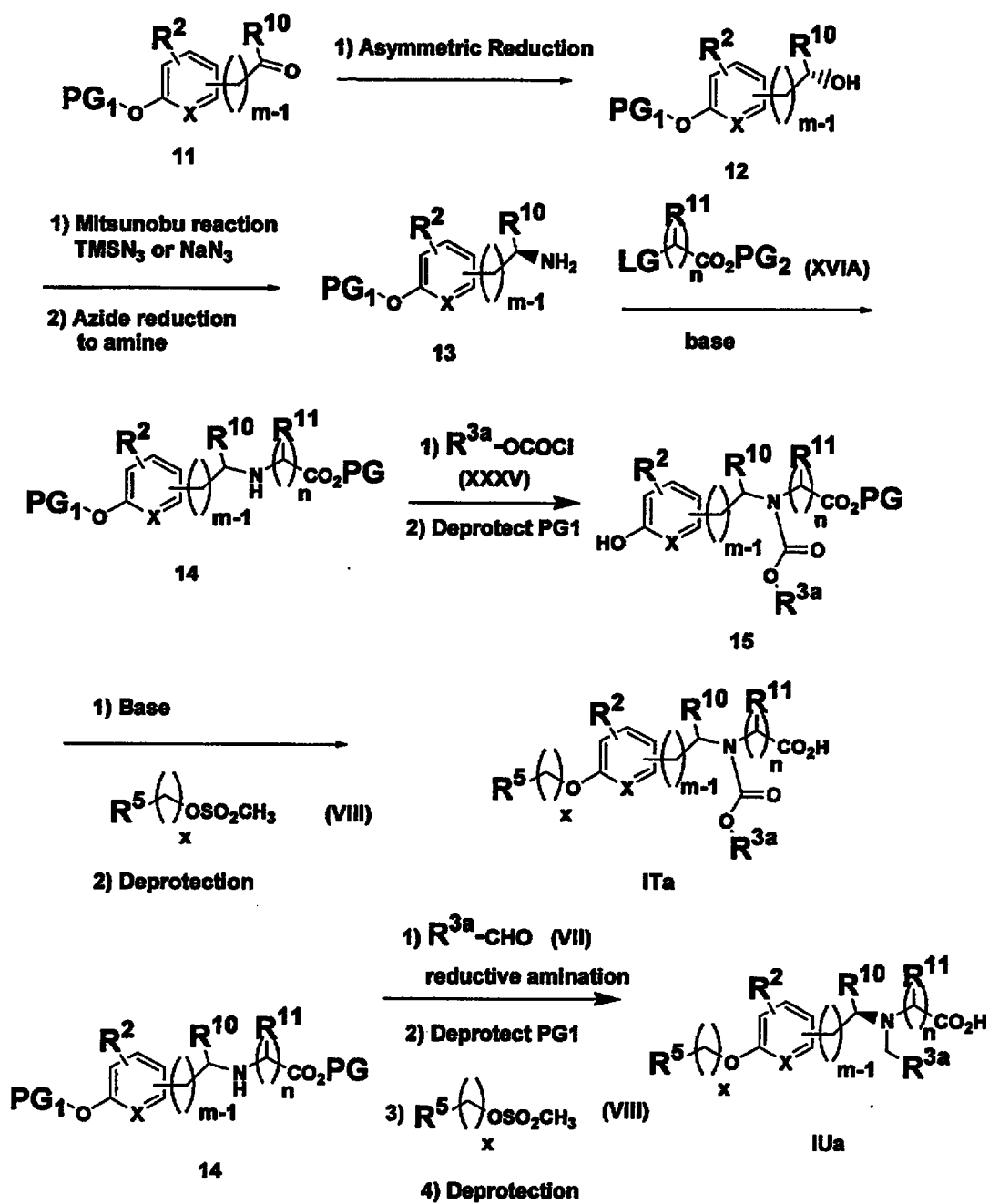
Scheme 22
