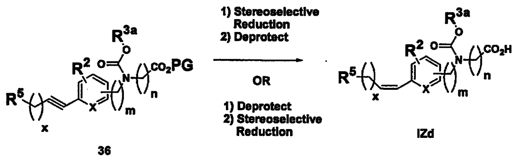
Scheme 28
