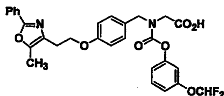
Example 307
