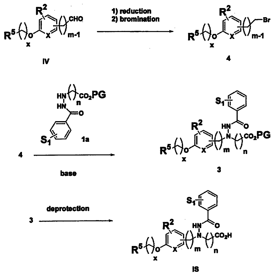
Scheme 19
