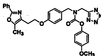
Example 463
