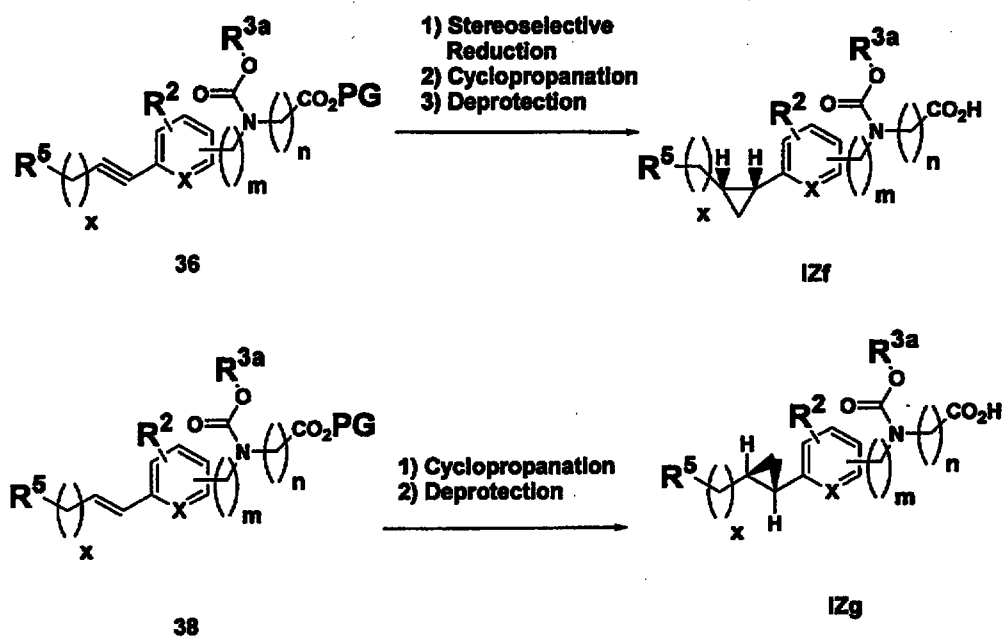
Scheme 30
