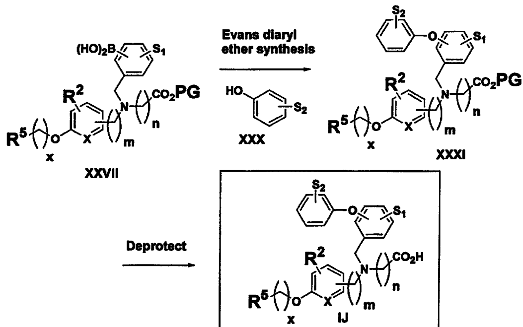
Scheme 9
