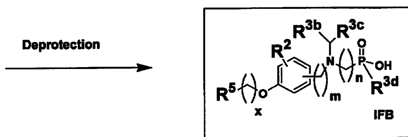
Scheme 5b
