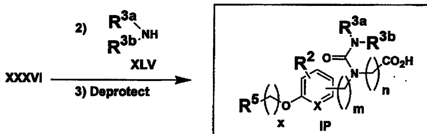
Scheme 15
