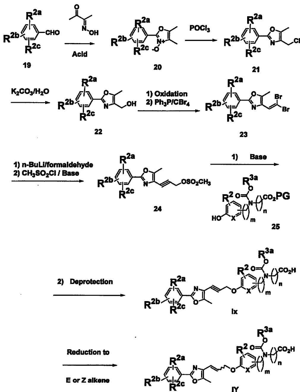
Scheme 24
