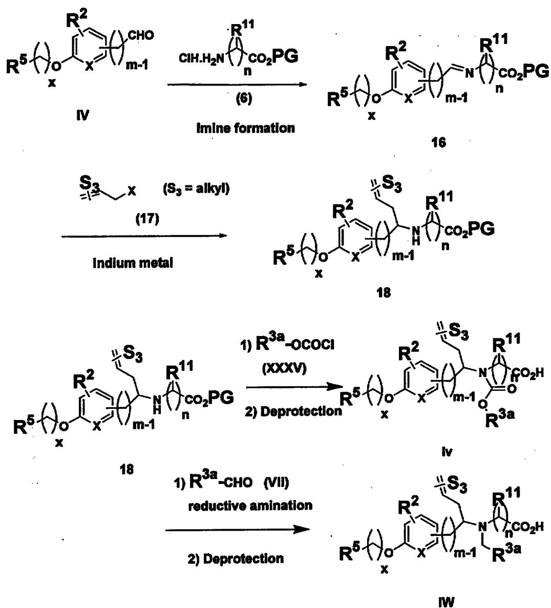
Scheme 23
