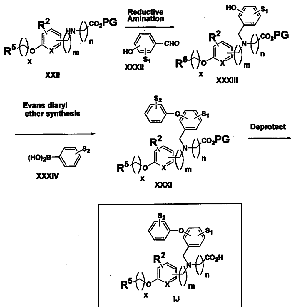
Scheme 10
