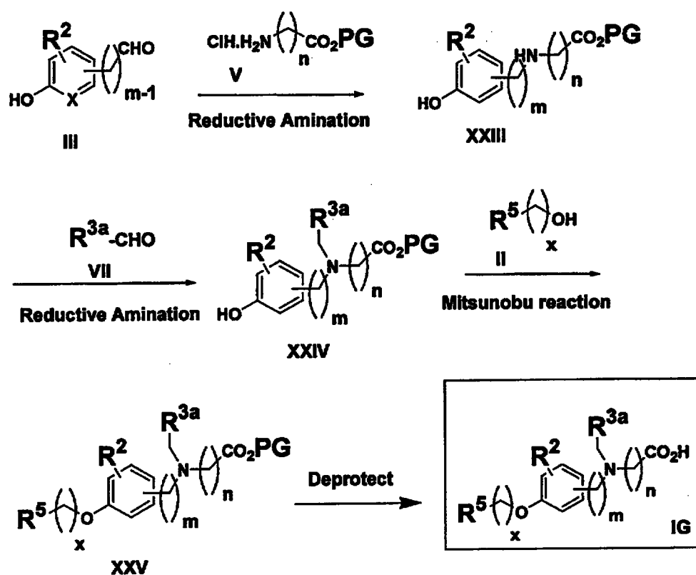
Scheme 7
