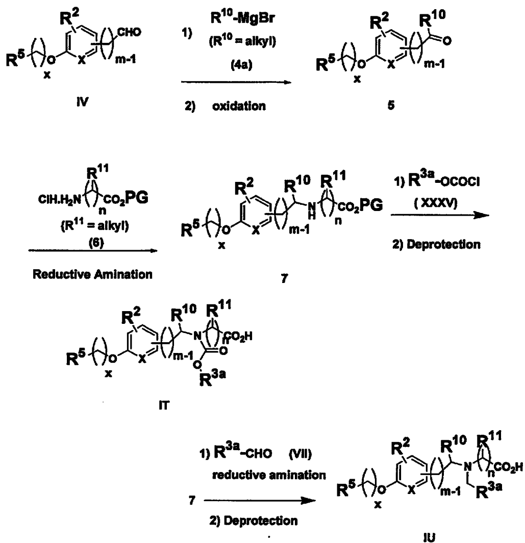
Scheme 20
