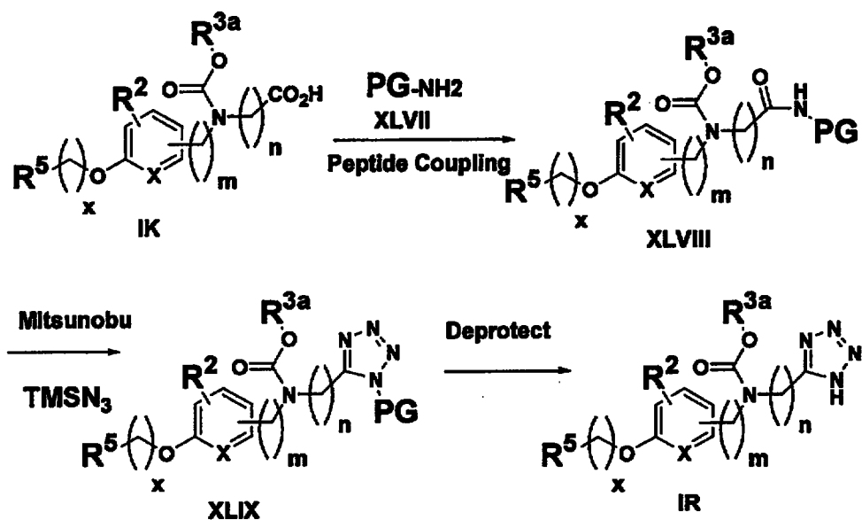
Scheme 17
