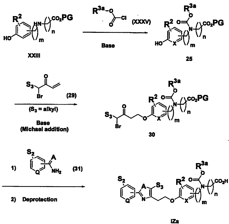
Scheme 26
