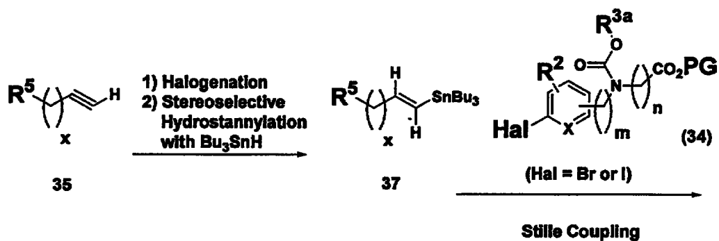
Scheme 28
