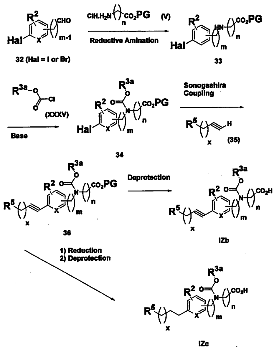
Scheme 27
