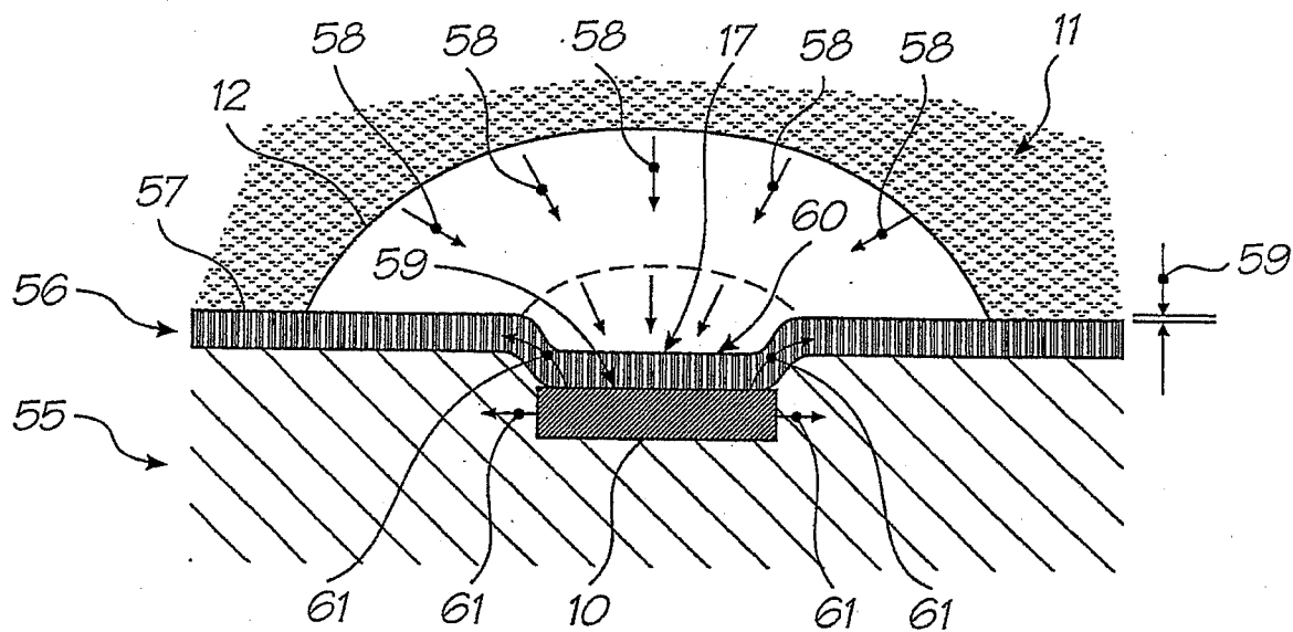
FIG. 47 (PRIOR ART)
