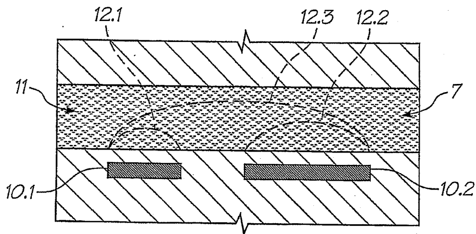
FIG. 52 (PRIOR ART)
