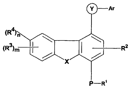
General Structure of formula (1A)
