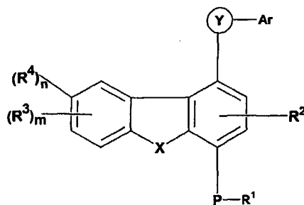
General Structure of formula (1A)
