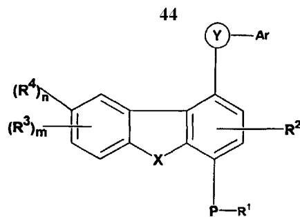
General Structure of formula (1A)
