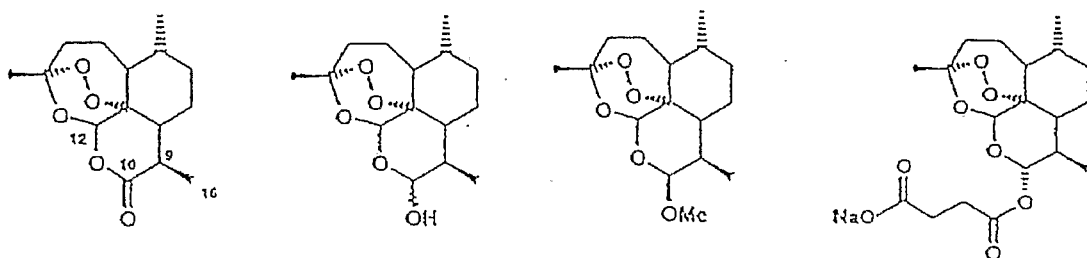
Artemisinin 1 Dihydroartemisinin 2 Artemether 3 Sodium Artesunate 4
