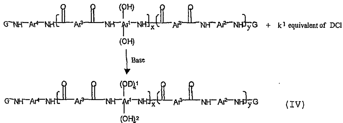
Reaction 2
