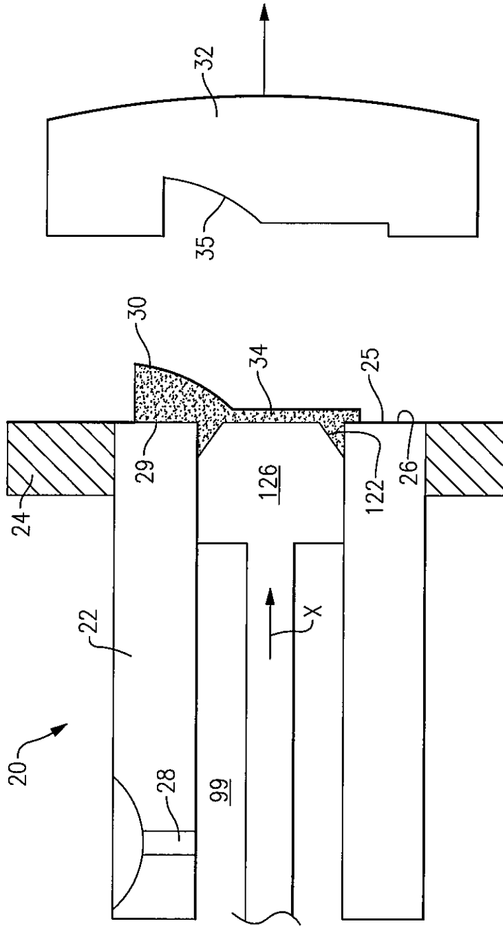
FIG. 1C Prior Art
