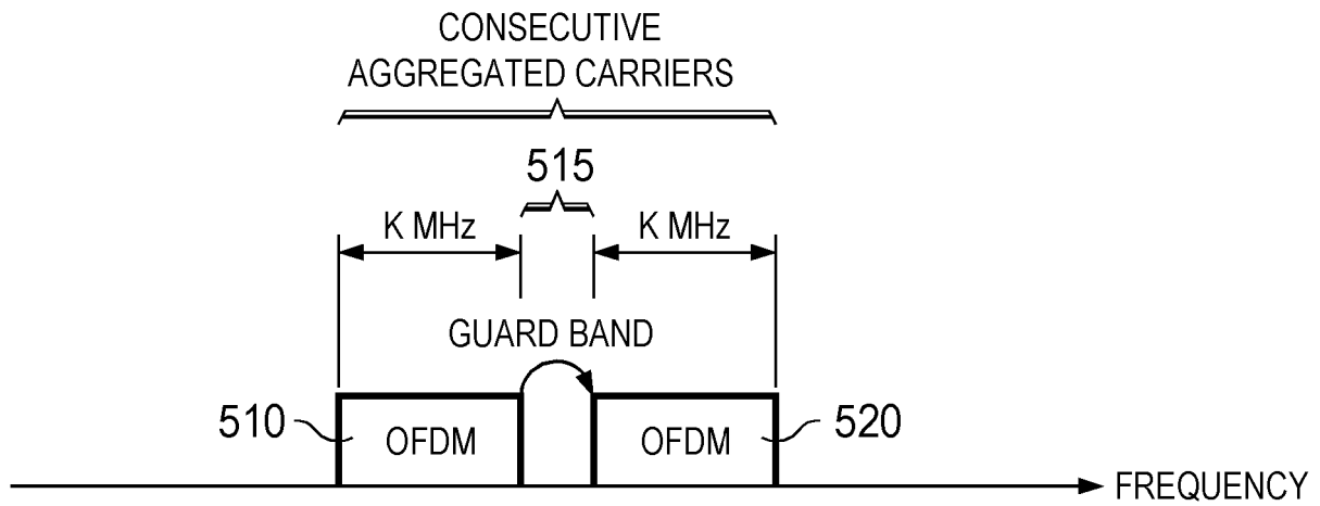
FIG. 5 (PRIOR ART)
