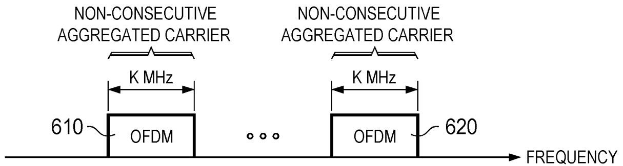
FIG. 6 (PRIOR ART)
