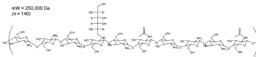
Figure 2. Exemplary structure of viscoelastic glycated chitosan of the present invention, where the deacetylation of the parent chitosan is about 80%, and the glycation of total available deacetylated amino groups is about 12.5%.
