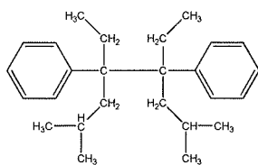
(Structure V); 3,4-dibenzyl-3,4-ditolyl hexane (DBnDTH)
