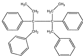
Structure VIII.
