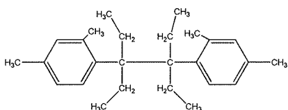
Structure VII; and, 3,4-dibenzyl-3,4-diphenyl hexane
