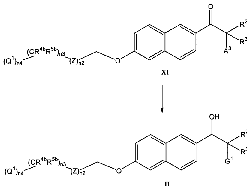
Scheme 13
