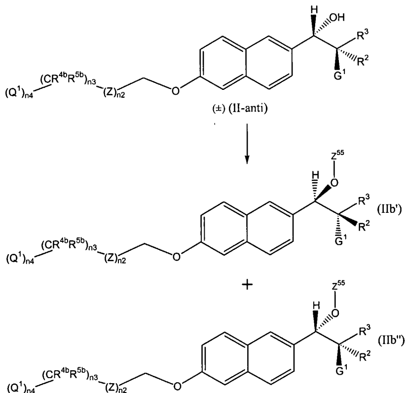
Scheme 29
