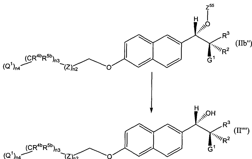
Scheme 27
