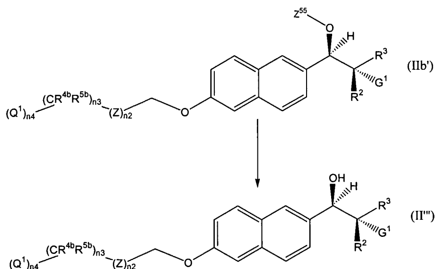
Scheme 26
