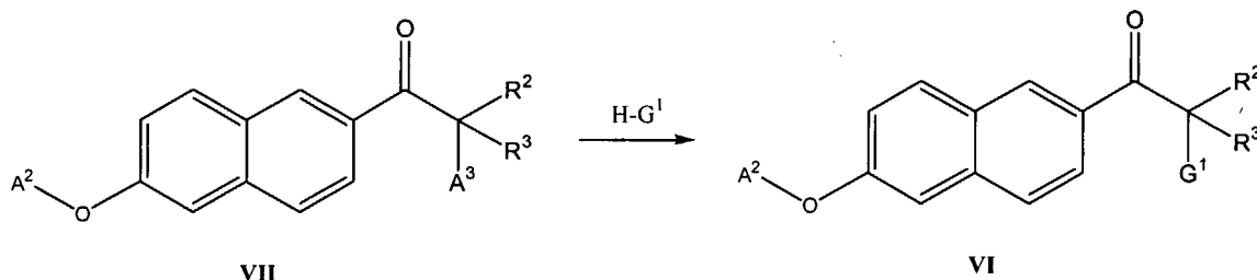
Scheme 5
