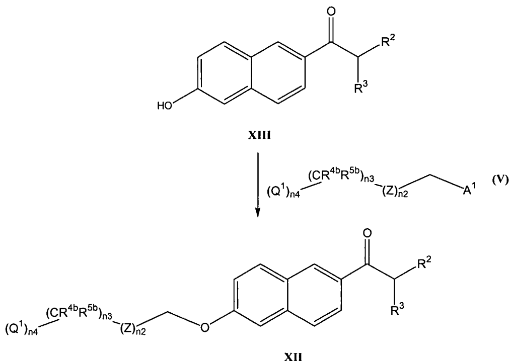
Scheme 9
