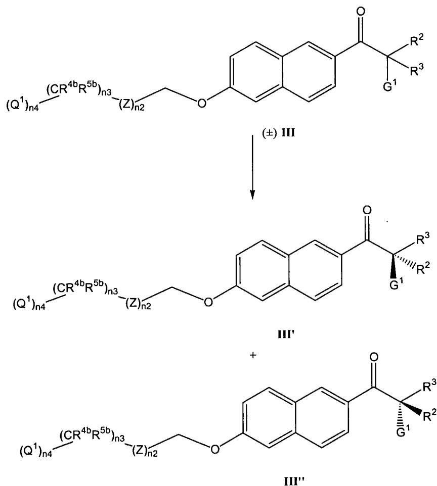
Scheme 21
