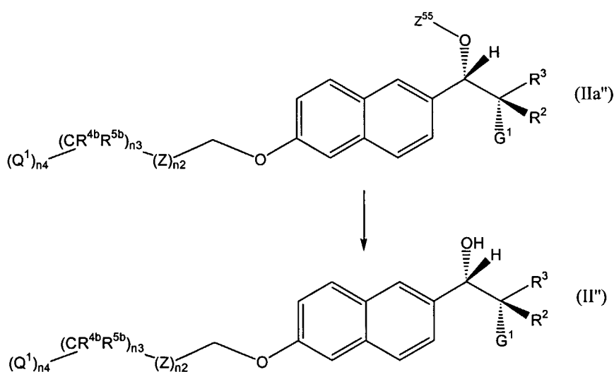
Scheme 25
