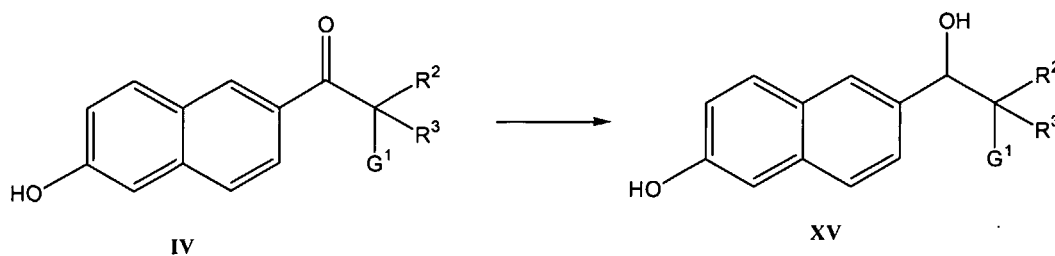
Scheme 16
