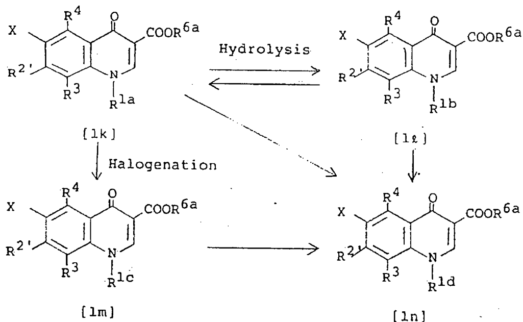
{Reaction scheme-XVI}
