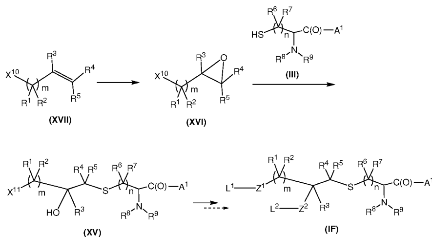
Scheme A1: Preparation of compounds of formula (IF) via conjugation to an epoxide.
