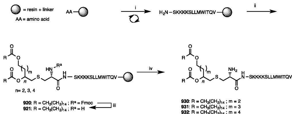
Scheme 2. (i) Iterative Fmoc-SPPS; (ii) ( R )-bis-pamitoylated Fmoc-Cys-OH 806 ( m=2 ) or 811 ( m=3 ) or 820 ( m=4 ), PyBOP, collidine, DMF; (iii) 20% piperidine/DMF; (iv) TFA/EDT/water.
