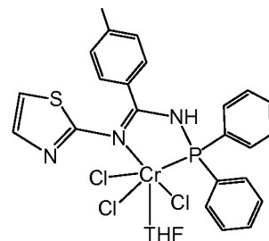
NP Amidine Metal Salt Complex D8
