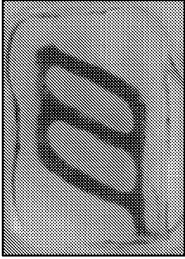
Fibrin
