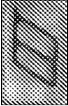
PEG-Diacrylate
