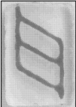
Agarose
