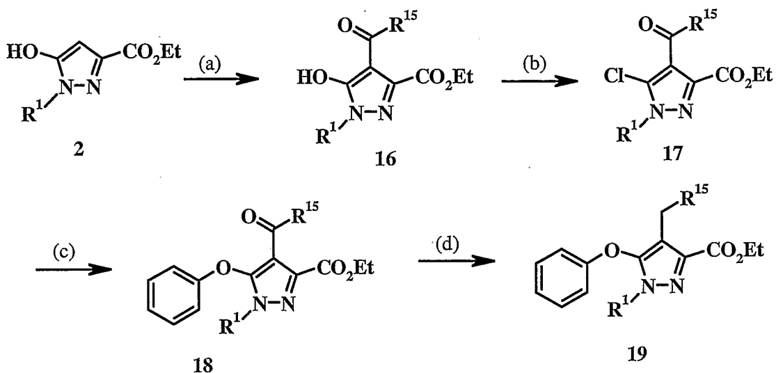
Scheme 4
