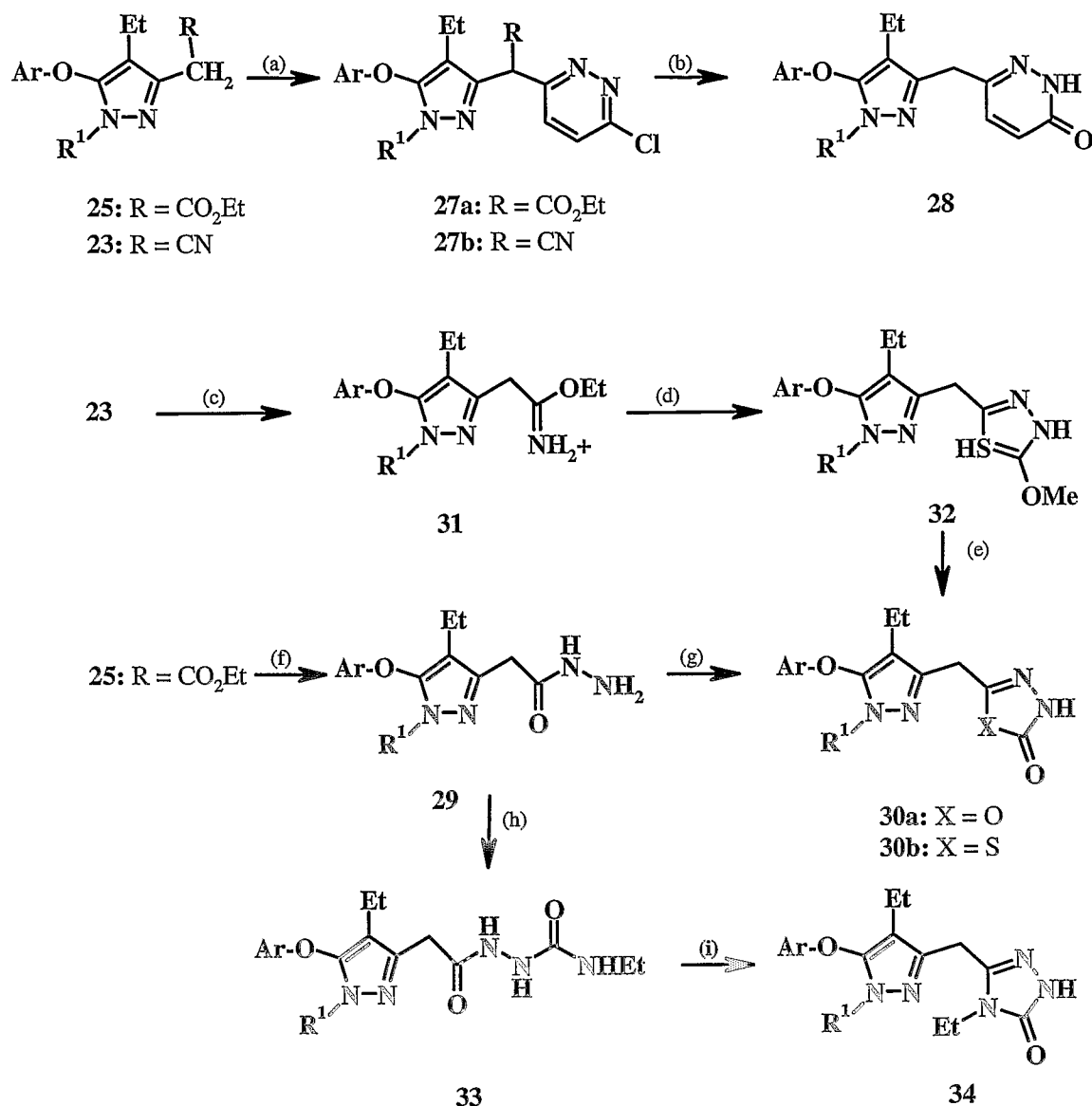
Scheme 6
