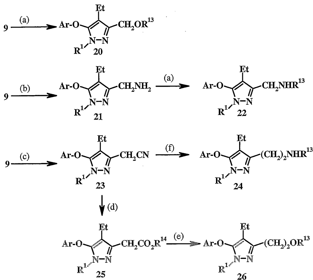
Scheme 6
