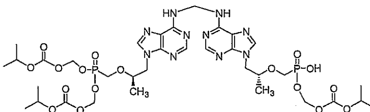
Mixed Dimer
