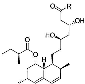
Lovastatin acid, amide or ester
