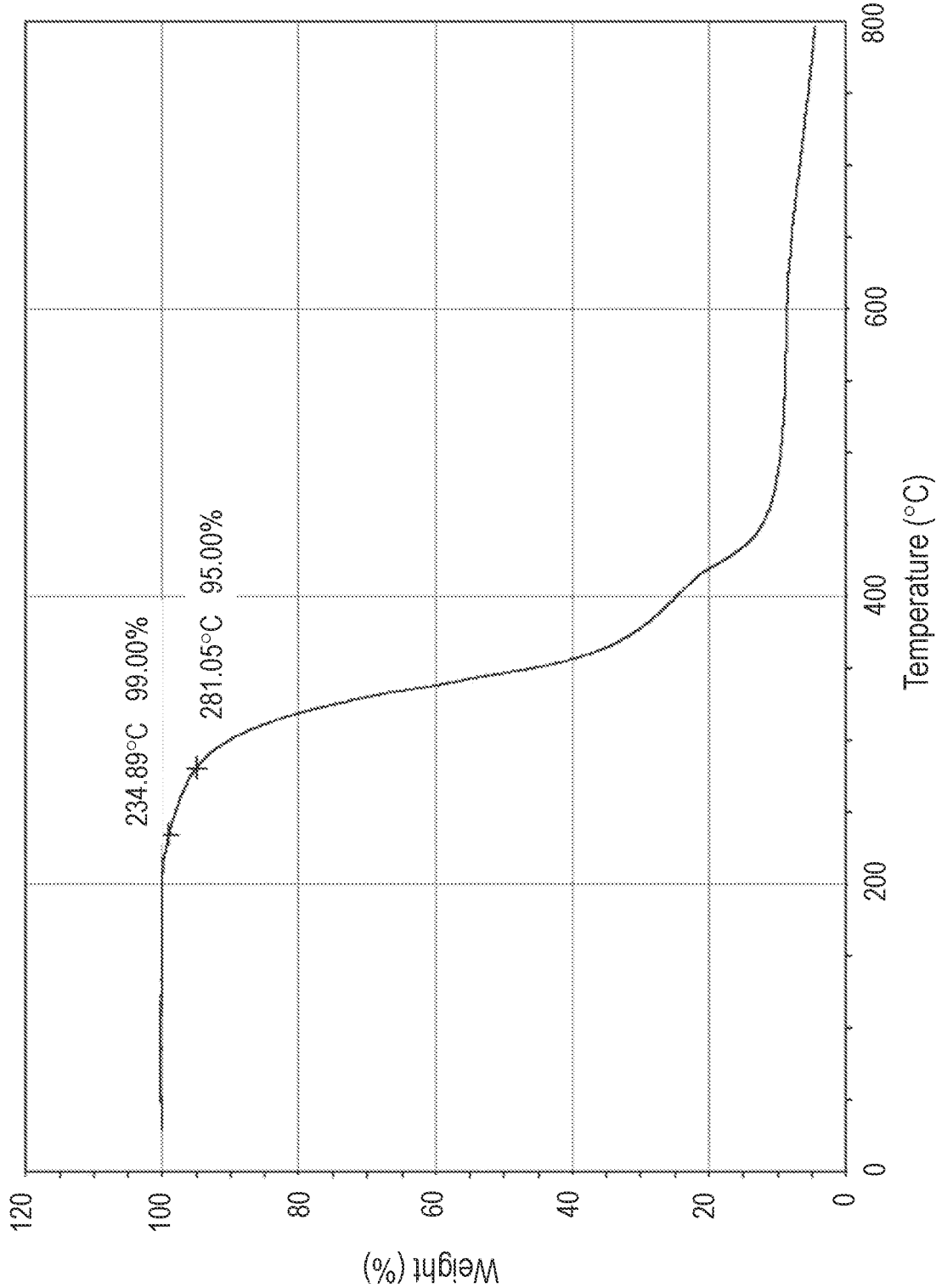
TGA of Example Q-PU-3
