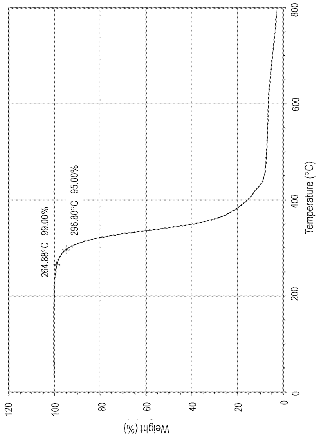
TGA of Example Q-PU-2
