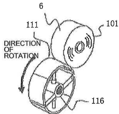
(a) WINDING START STEP
