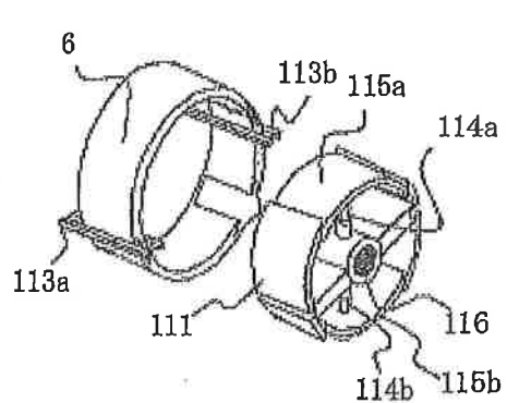
(h) ILLUSTRATION OF FINISHED LAMINATED BODY
