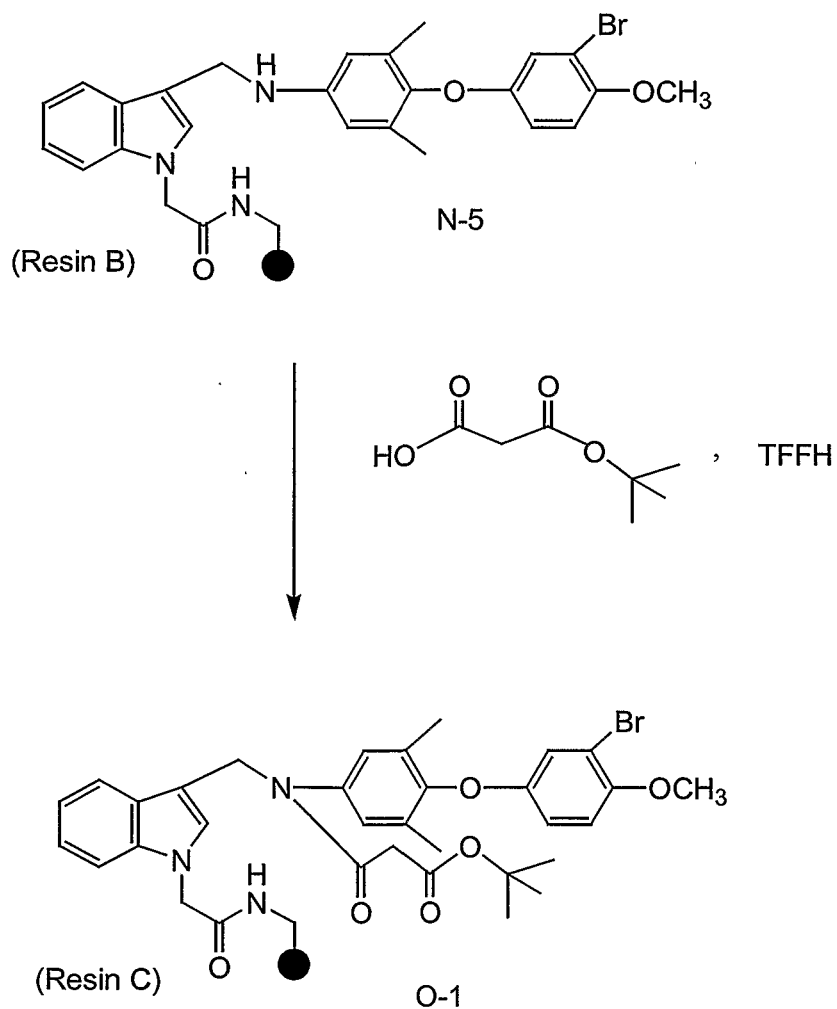
Scheme O
