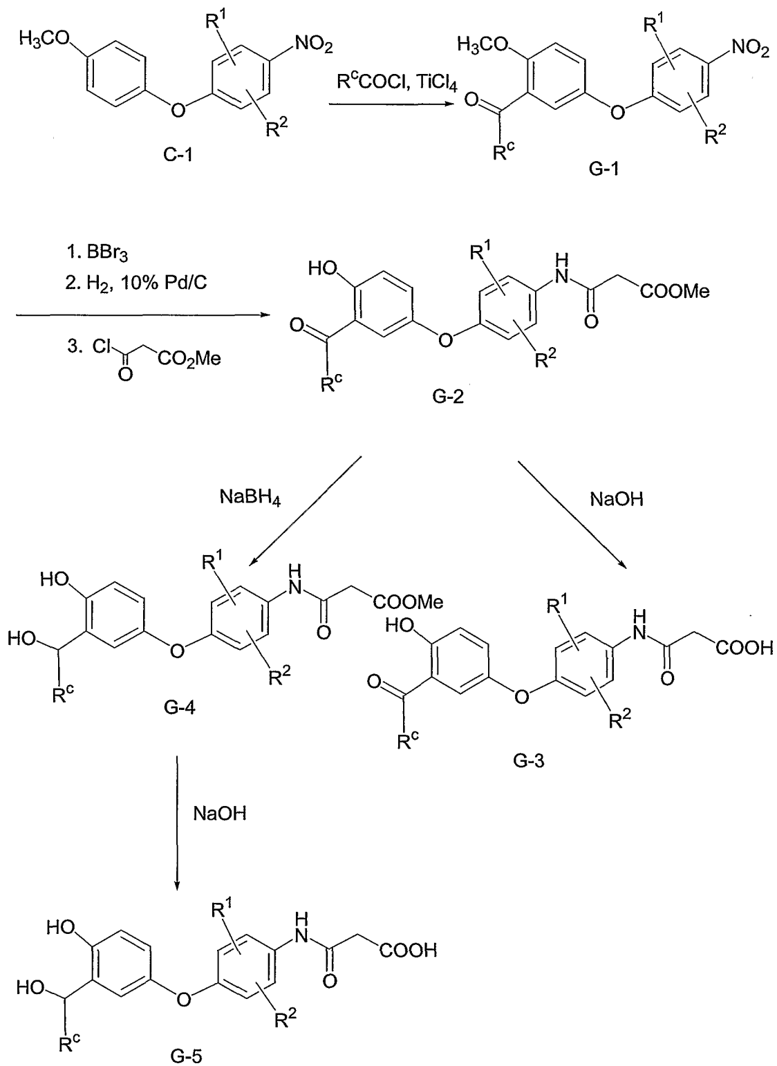
Scheme G
