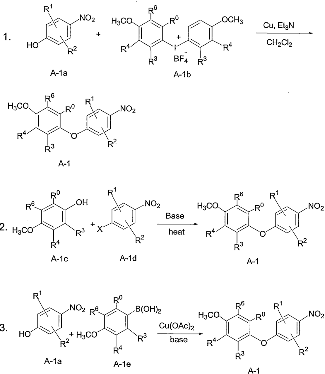
Scheme A
