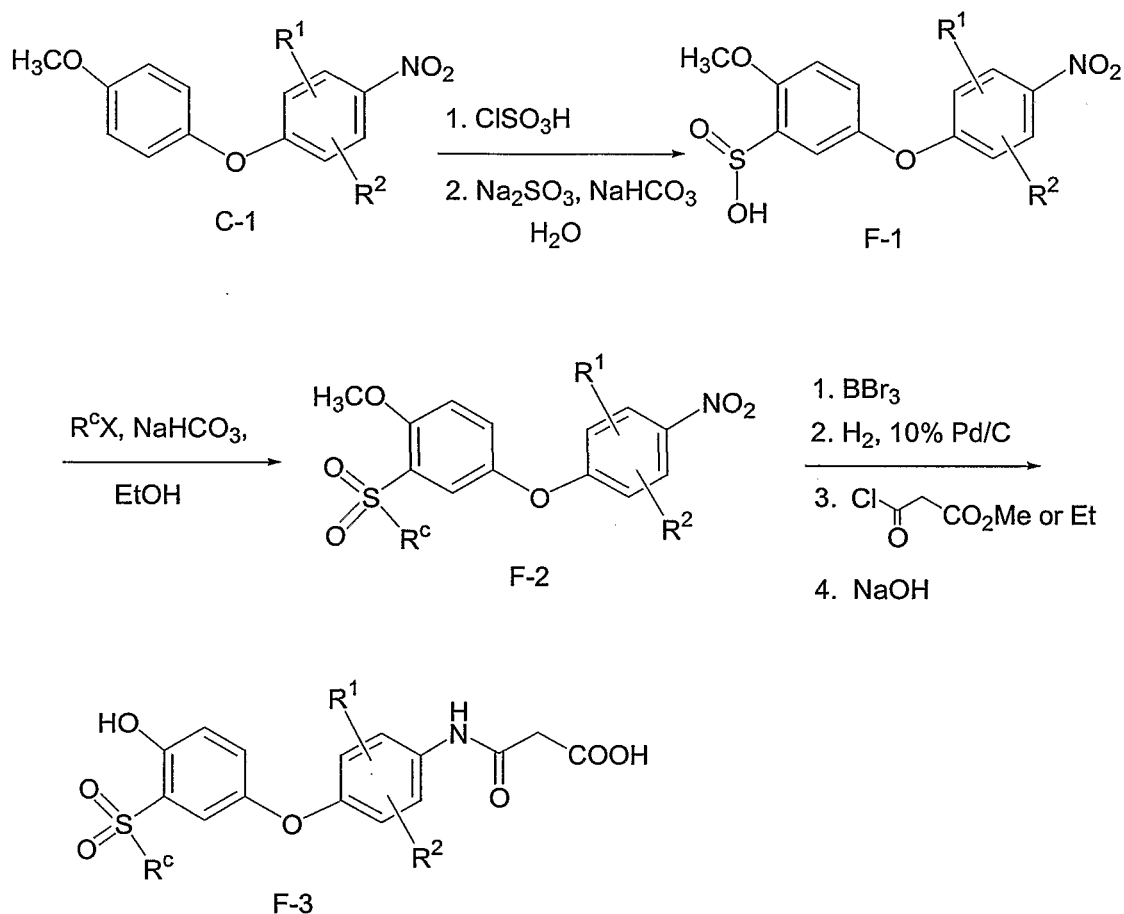
Scheme F
