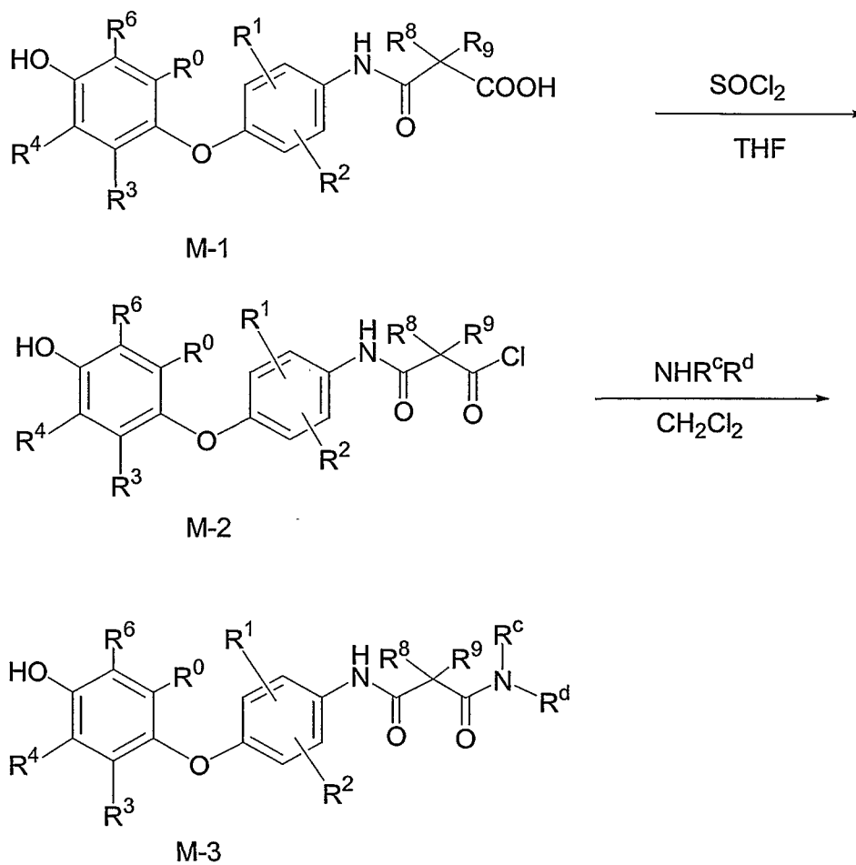
Scheme M
