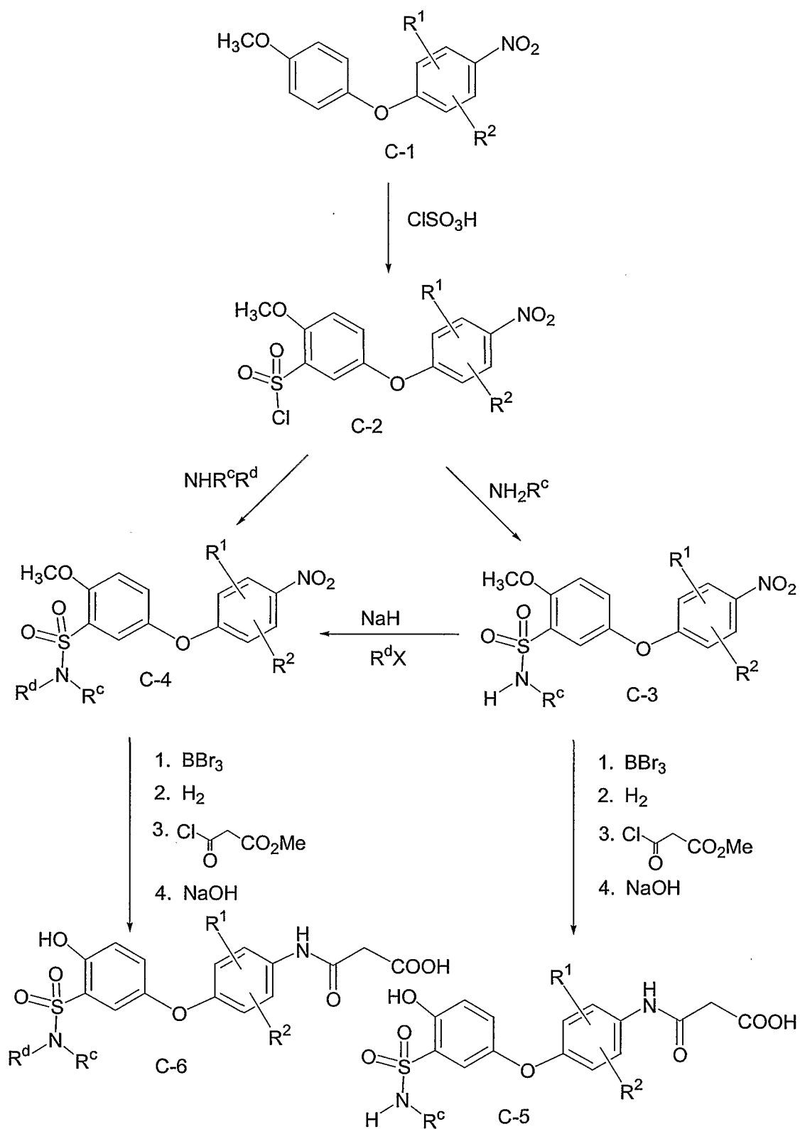
Scheme C
