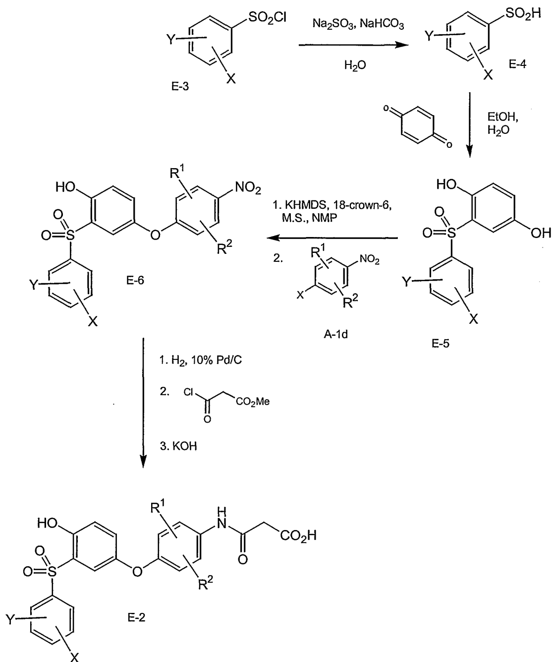
Scheme E
