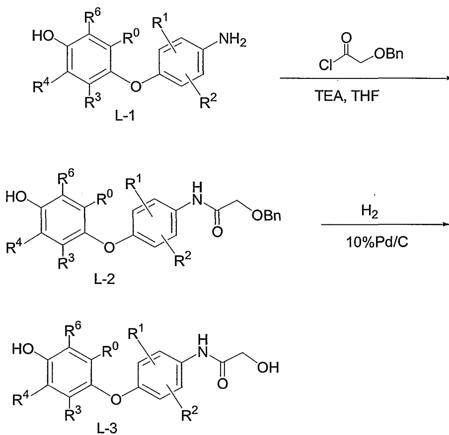
Scheme L
