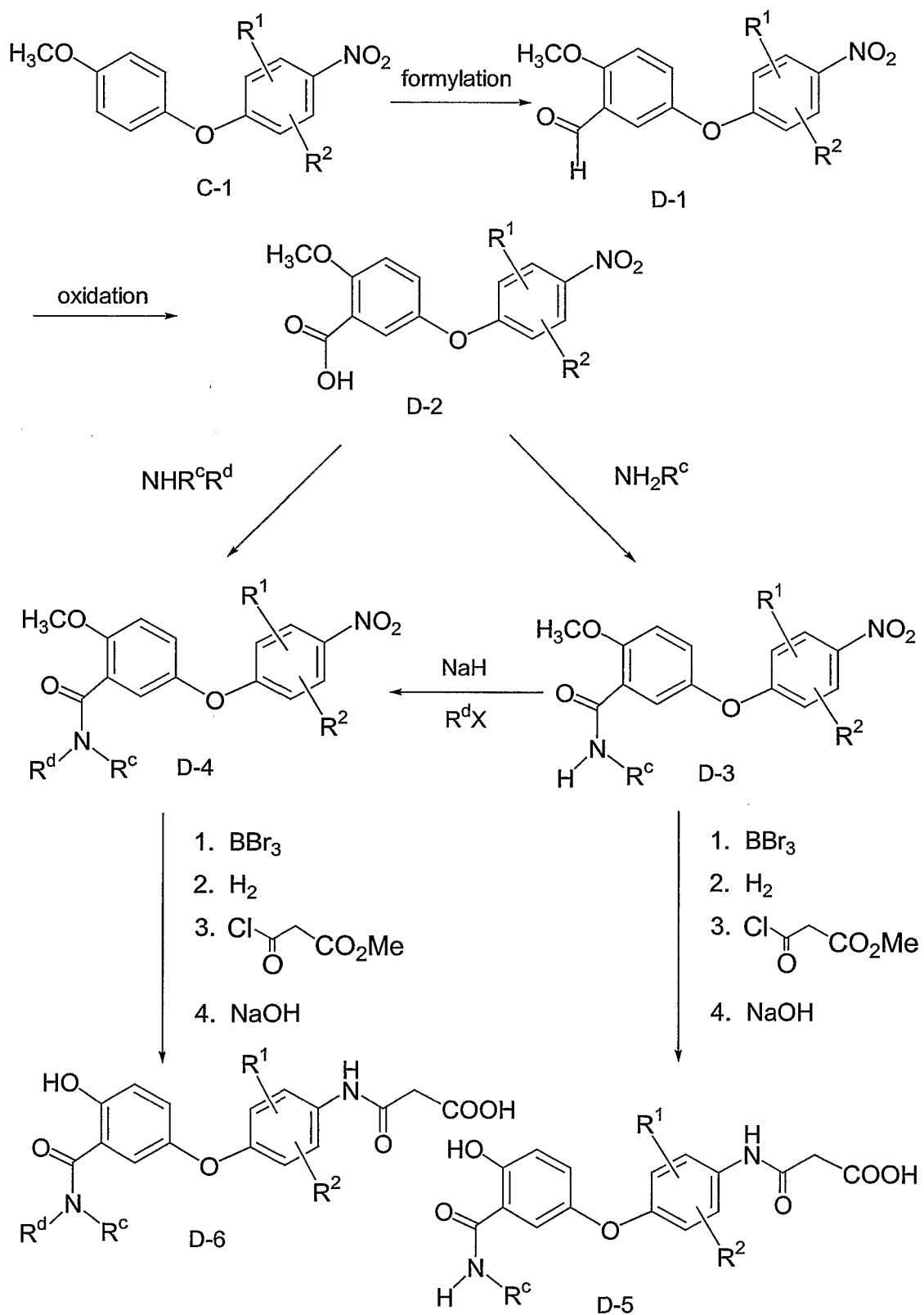
Scheme D
