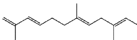
(3E,7E,10E)-2,7,10-trimethyldodeca-1,3,7,10-tetraene
