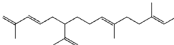
(6E,9E,13E)-2,10,13-trimethyl-6-(prop-1-en-2-yl)pentadeca-1,3,9,13-tetraene
