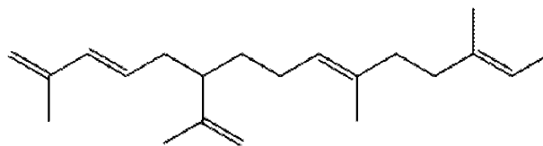
(6E,9E,13E)-2,10,13-trimethyl-6-(prop-1-en-2-yl)pentadeca-1,3,9,13-tetraene
