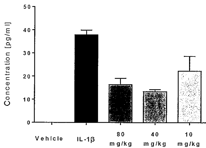
Figure 2: Treatment of an IL-1 \beta -induced inflammation with Exemplary Compound 64 leads to a reduced amount of secreted TNF- \alpha
