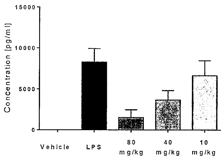
Figure 1: Treatment of LPS-induced inflammation with Exemplary Compound 64 leads to a reduced amount of secreted TNF- \alpha
