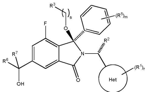
Diastereoisomer 1B
