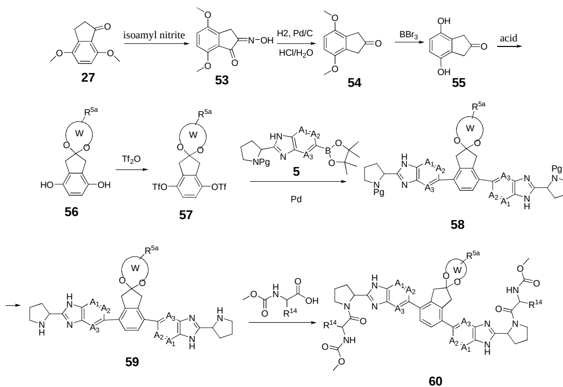
[00266] Scheme 9
