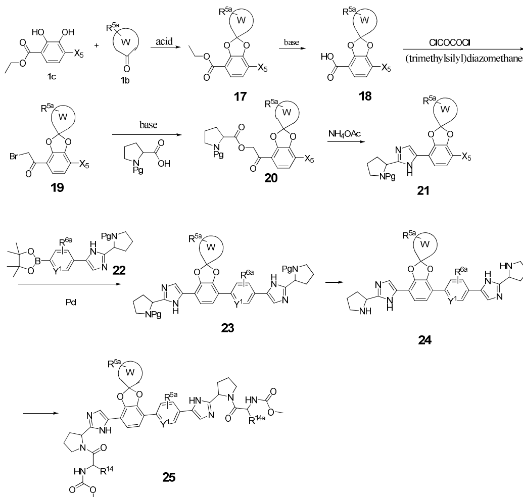
[00256] Scheme 4
