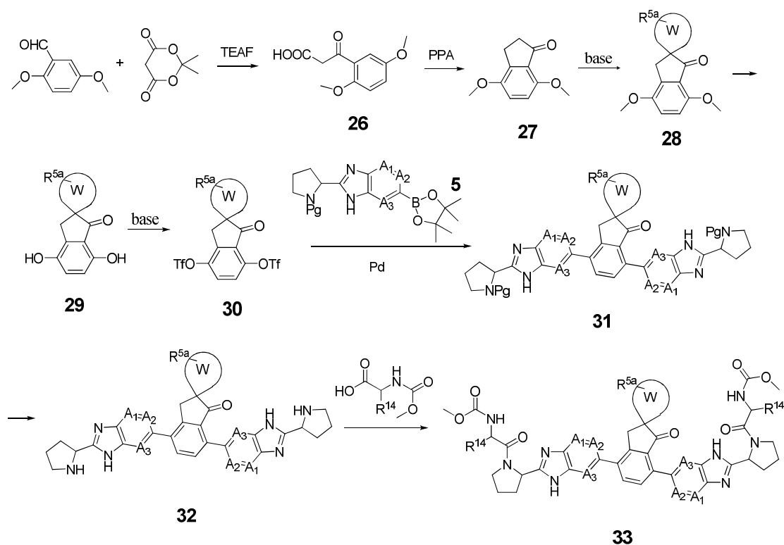
[00258] Scheme 5
