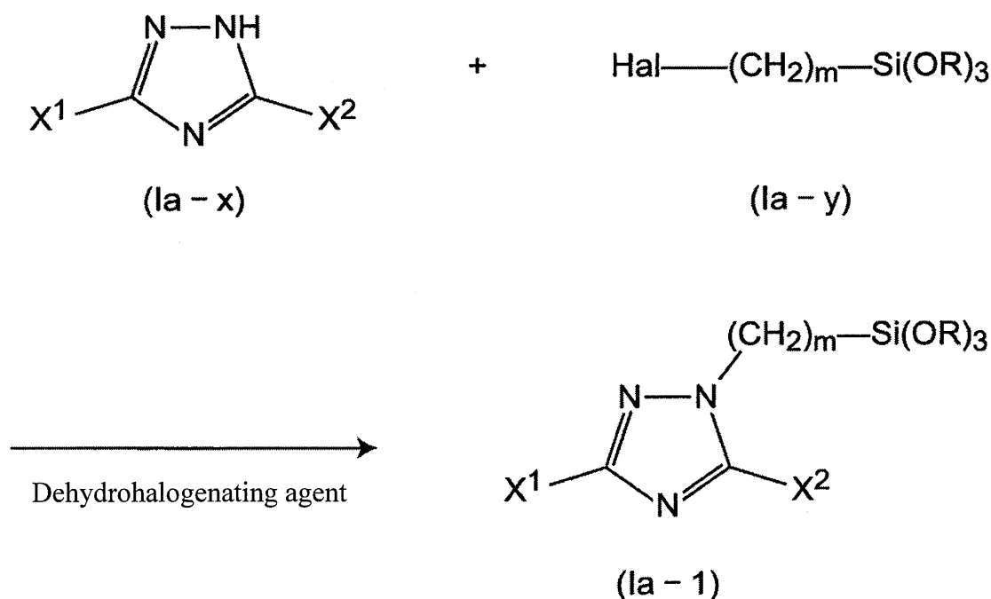
Reaction scheme (E)
