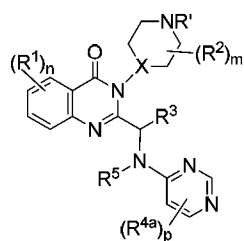
(IIc)
