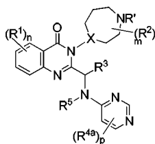
(IIIc)
