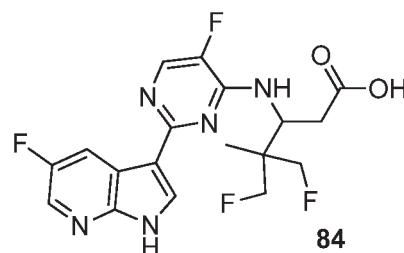
(+/-)-5-Fluoro-3-((5-fluoro-2-(5-fluoro-1H-pyrrolo[2,3-b]pyridin-3-yl)pyrimidin-4-yl)amino)-4-(fluoromethyl)-4-methylpentanoic acid (84)
