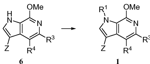
Scheme 2
