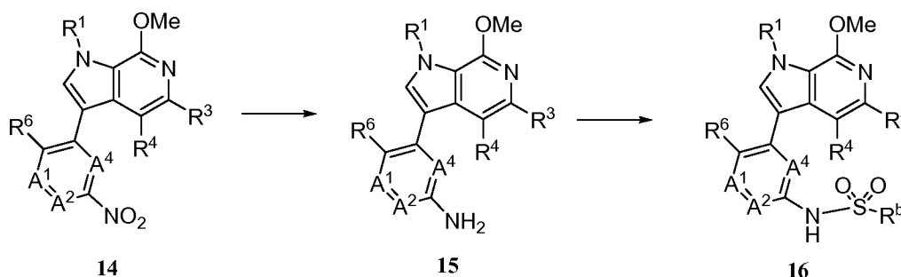
Scheme 5
