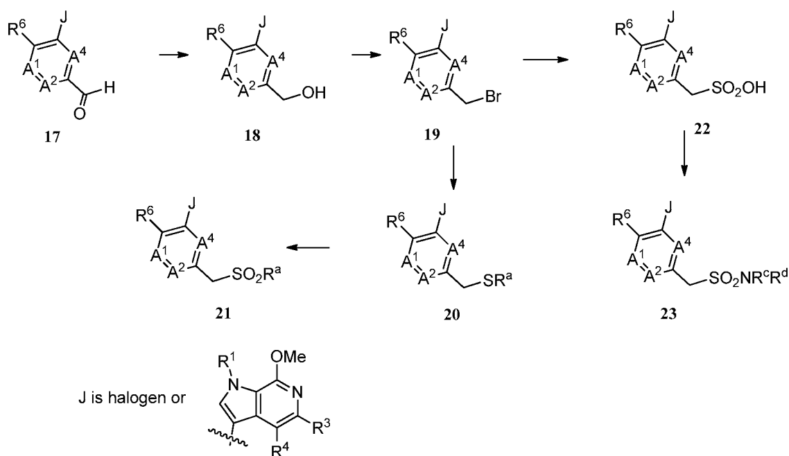
Scheme 6
