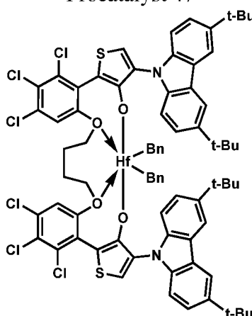
Procatalyst 50
