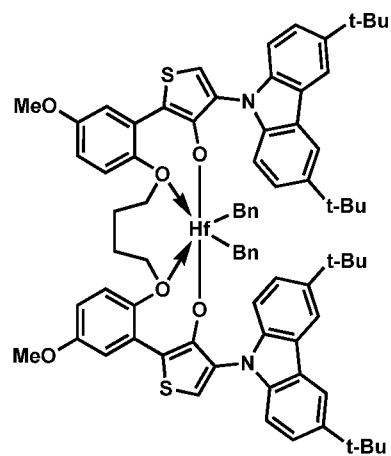
Procatalyst 30
