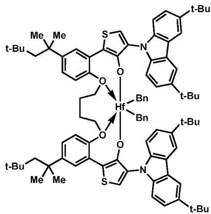
Procatalyst 32
