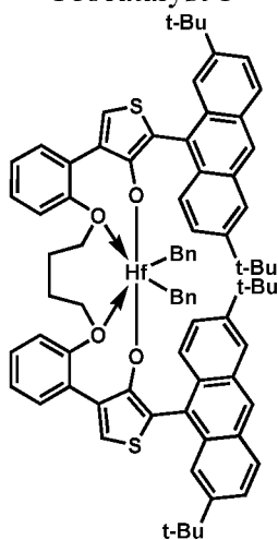
Procatalyst 4
