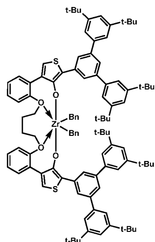
Procatalyst 9
