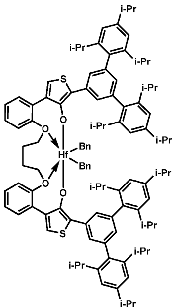
Procatalyst 16
