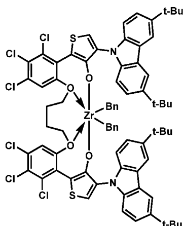
Procatalyst 49
