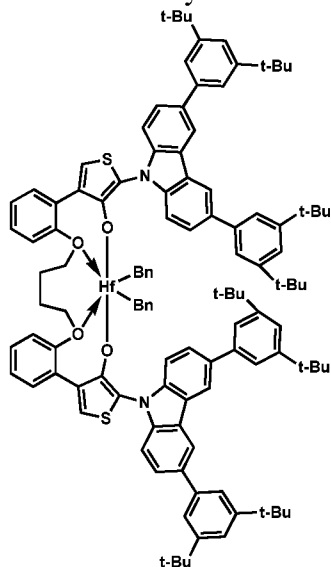
Procatalyst 20
