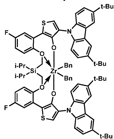
Procatalyst 27
