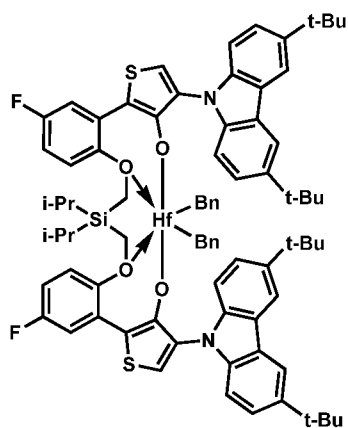
Procatalyst 28
