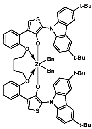
Procatalyst 5
