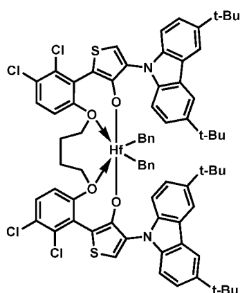
Procatalyst 46
