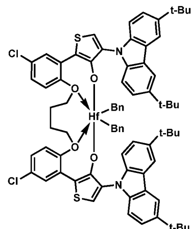
Procatalyst 42
