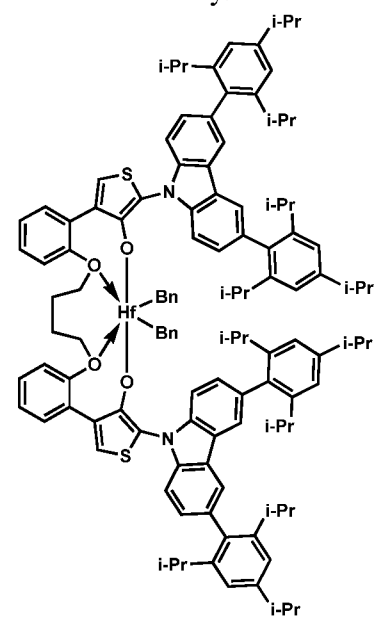
Procatalyst 18
