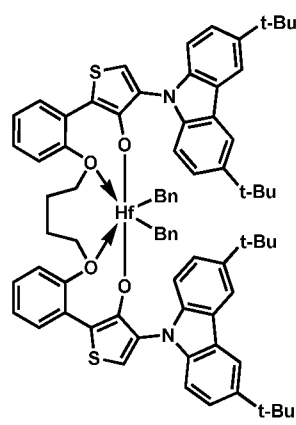
Procatalyst 24
