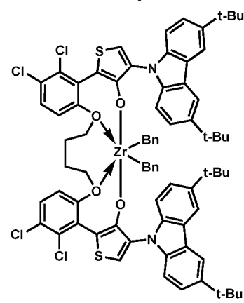
Procatalyst 45
