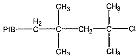
PIB tert-Chloride
