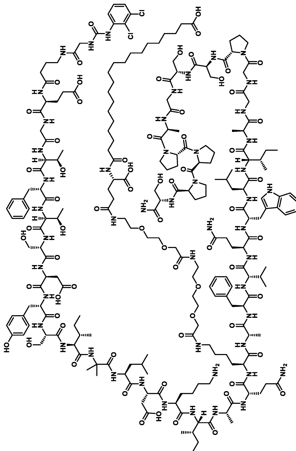
Compound 262
