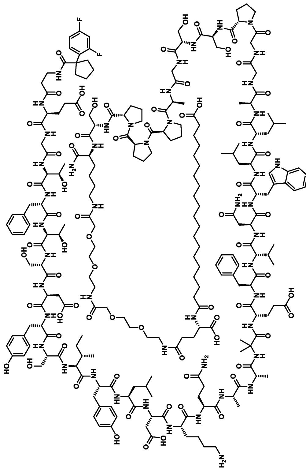
Compound 145
