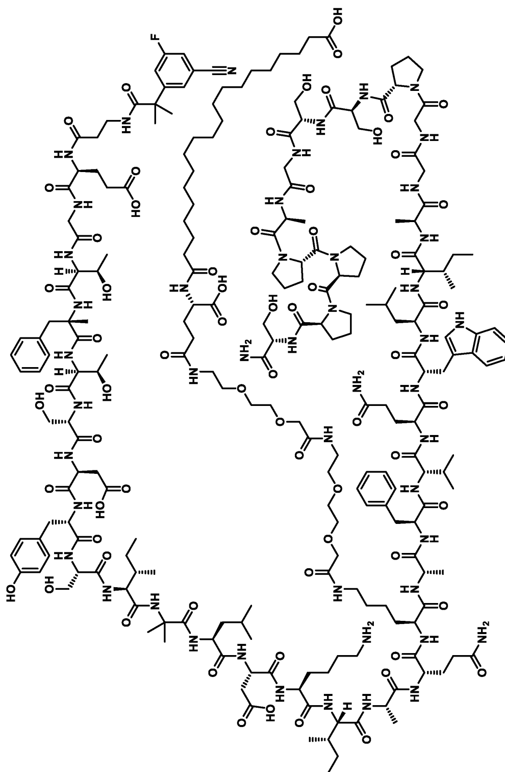
Compound 235
