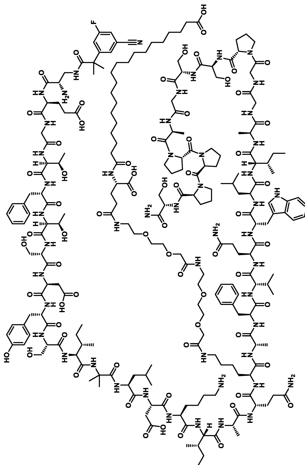
Compound 191
