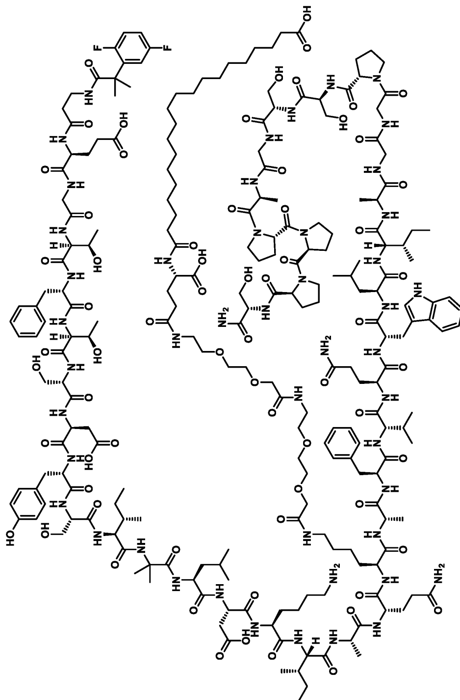
Compound 146
