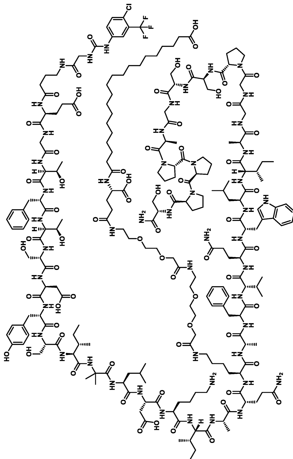
Compound 265
