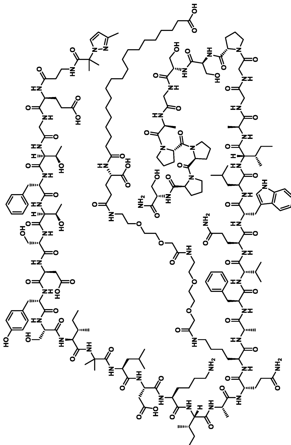
Compound 253
