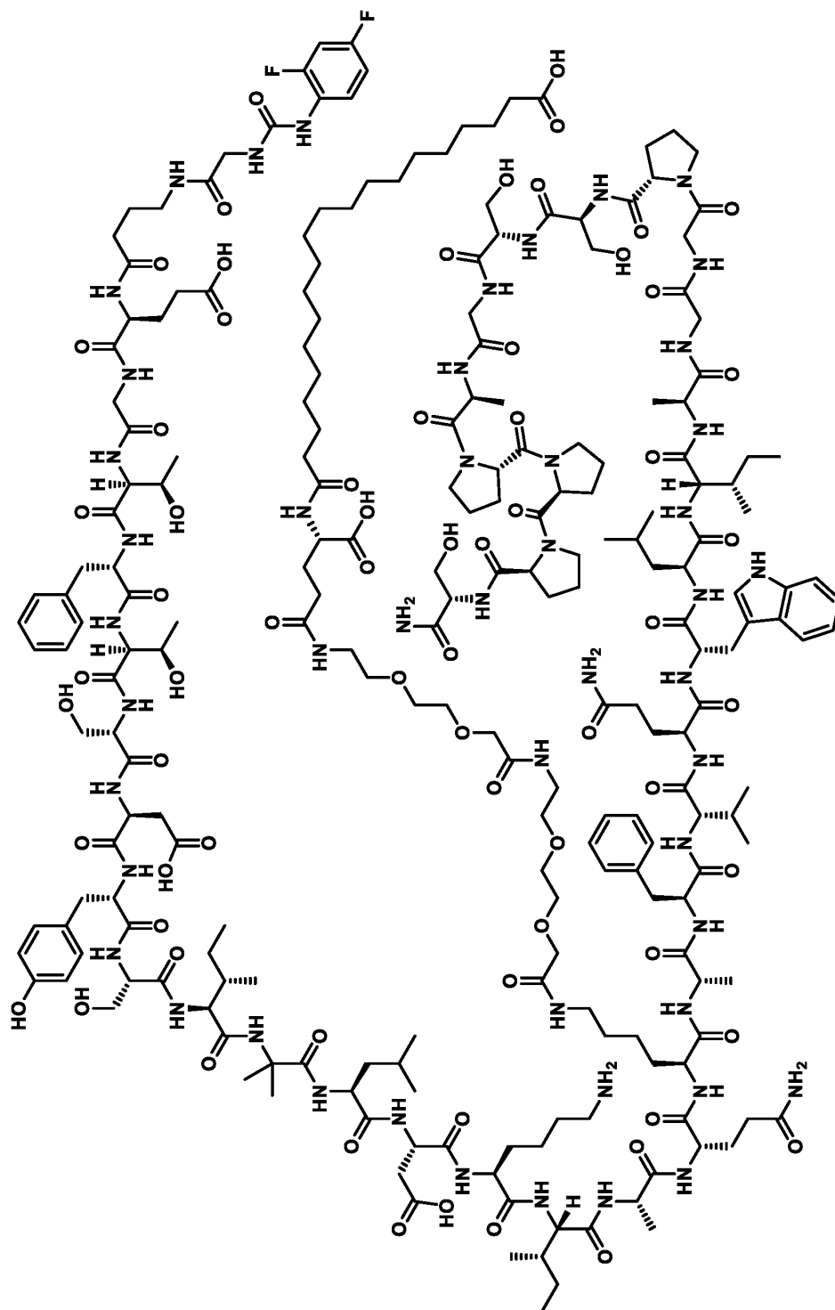
Compound 267
