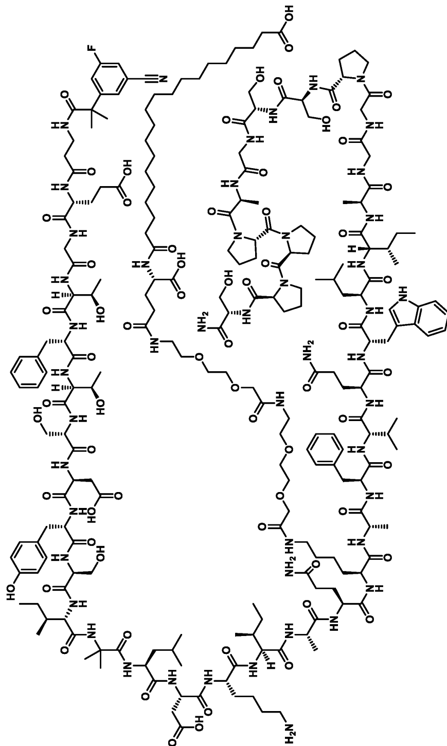
Compound 109
