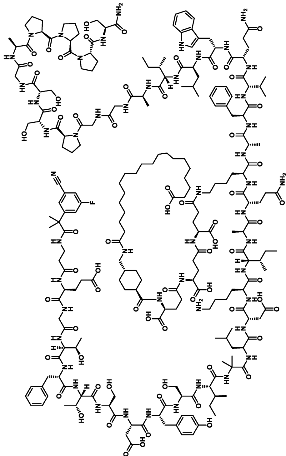
Compound 107
