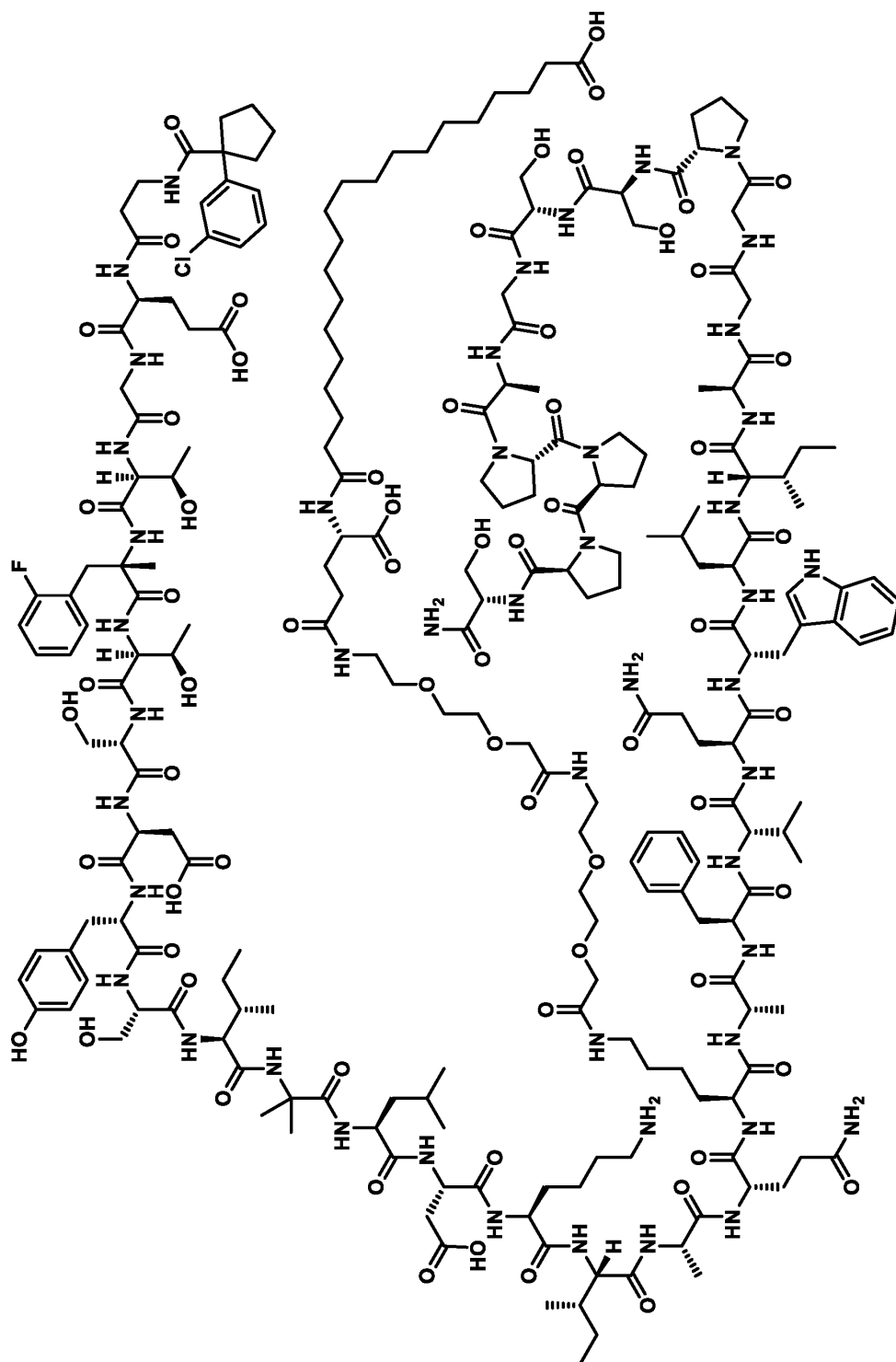
Compound 179
