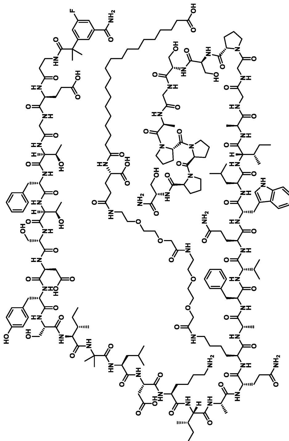
Compound 159
