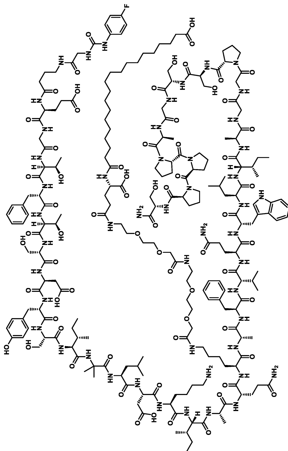
Compound 268
