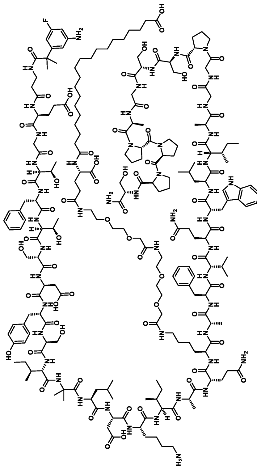
Compound 133
