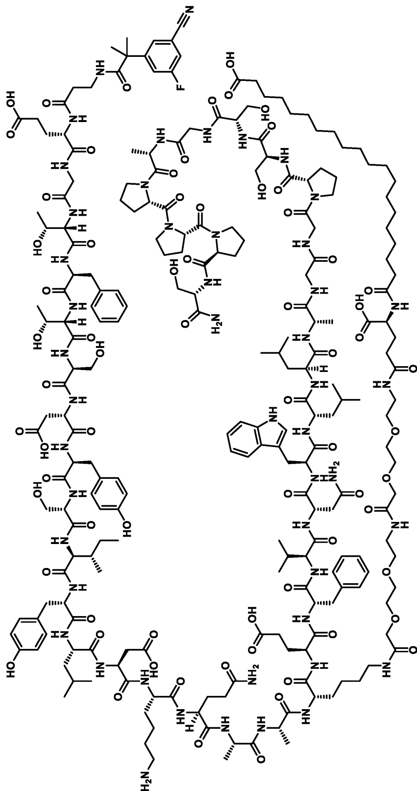
Compound 184
