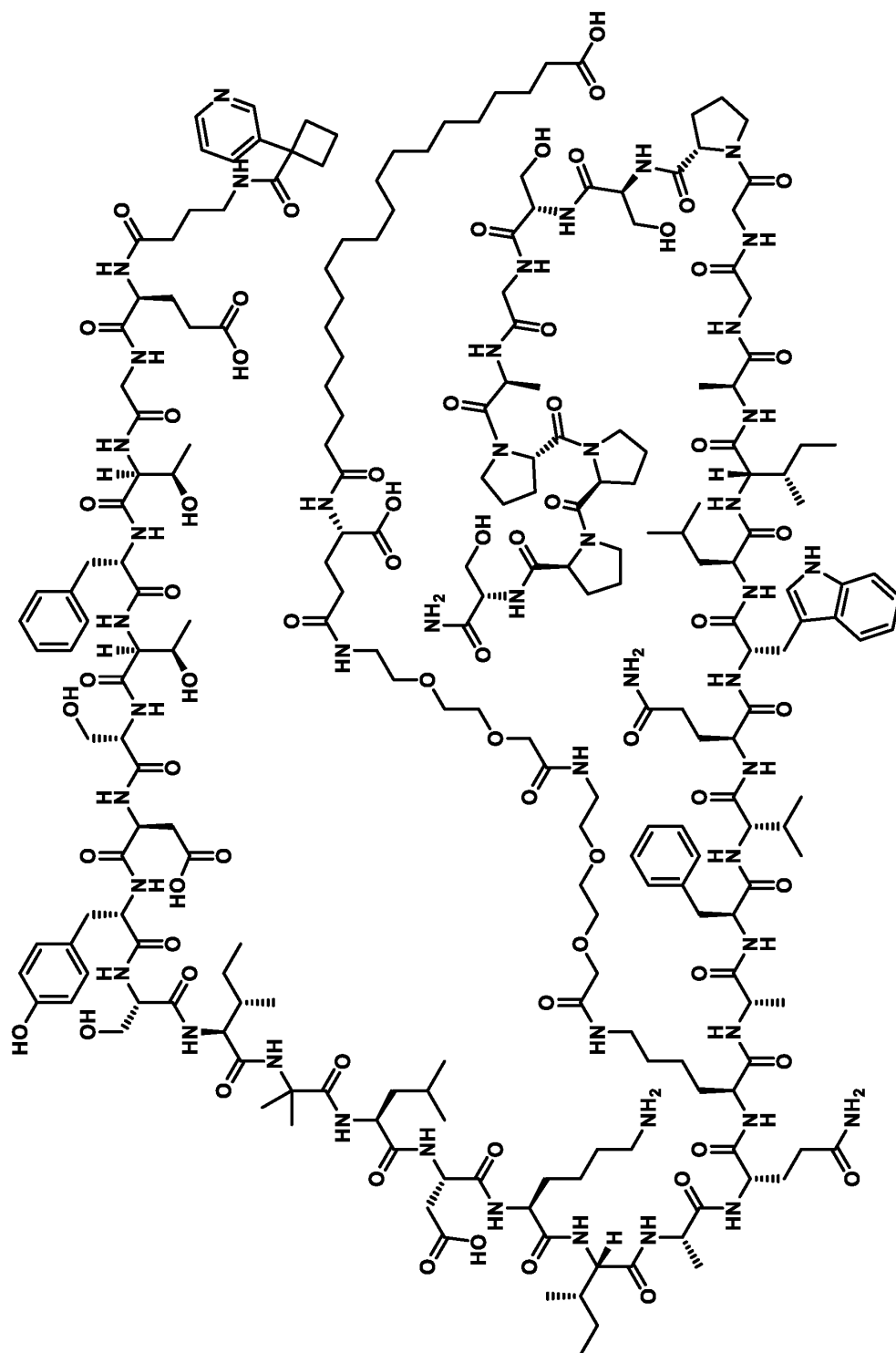
Compound 251
