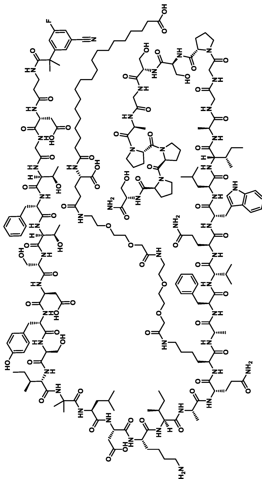
Compound 127
