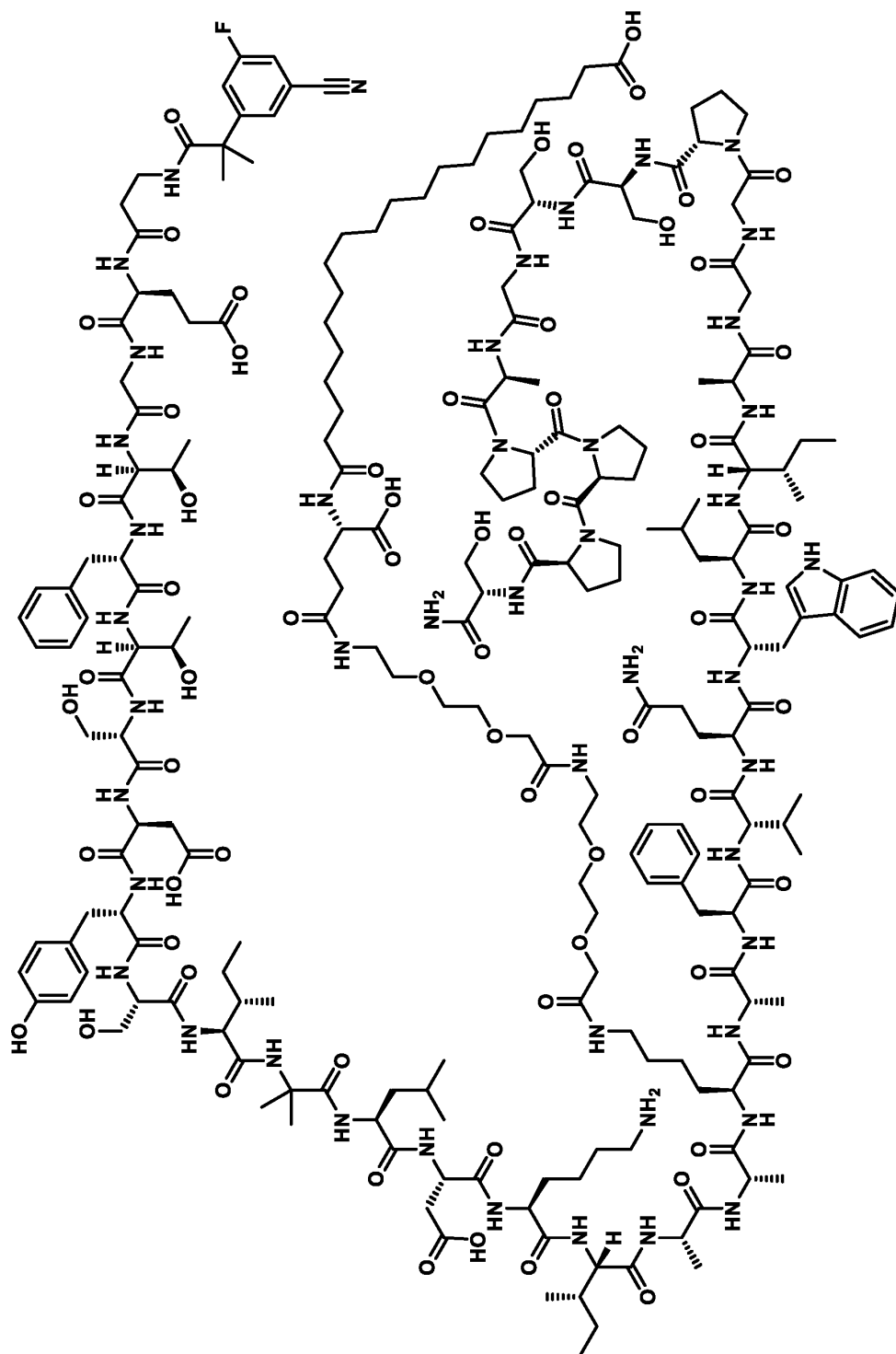
Compound 183
