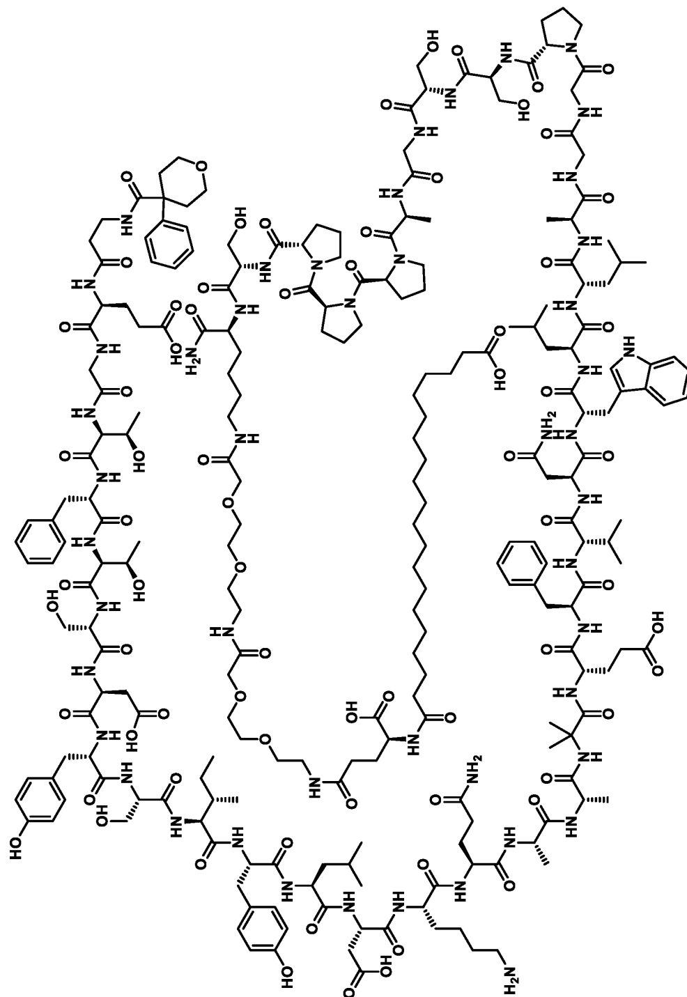
Compound 154
