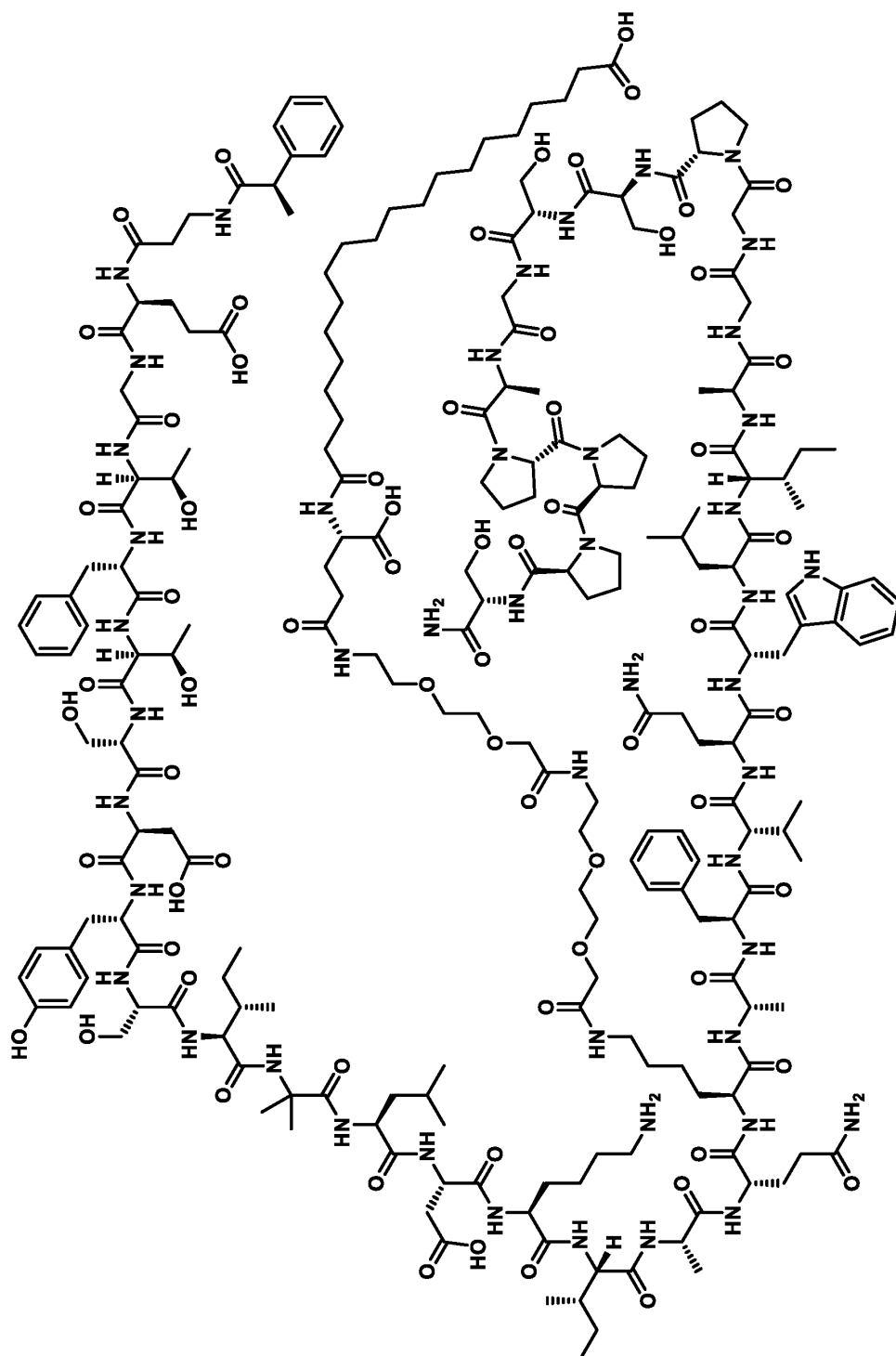
Compound 204
