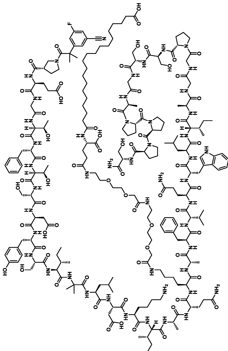
Compound 195
