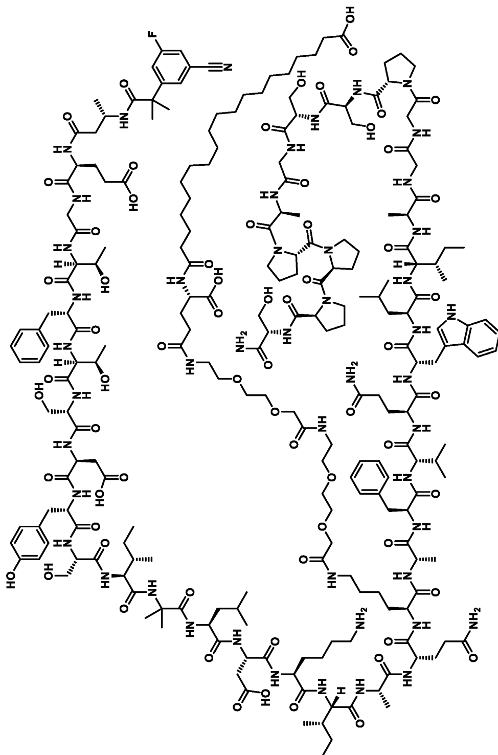
Compound 222
