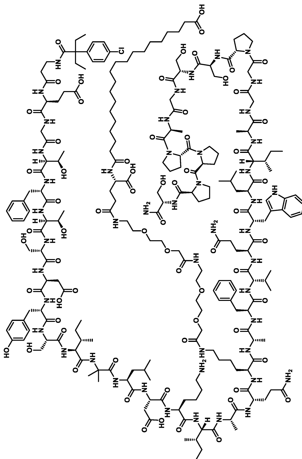
Compound 176
