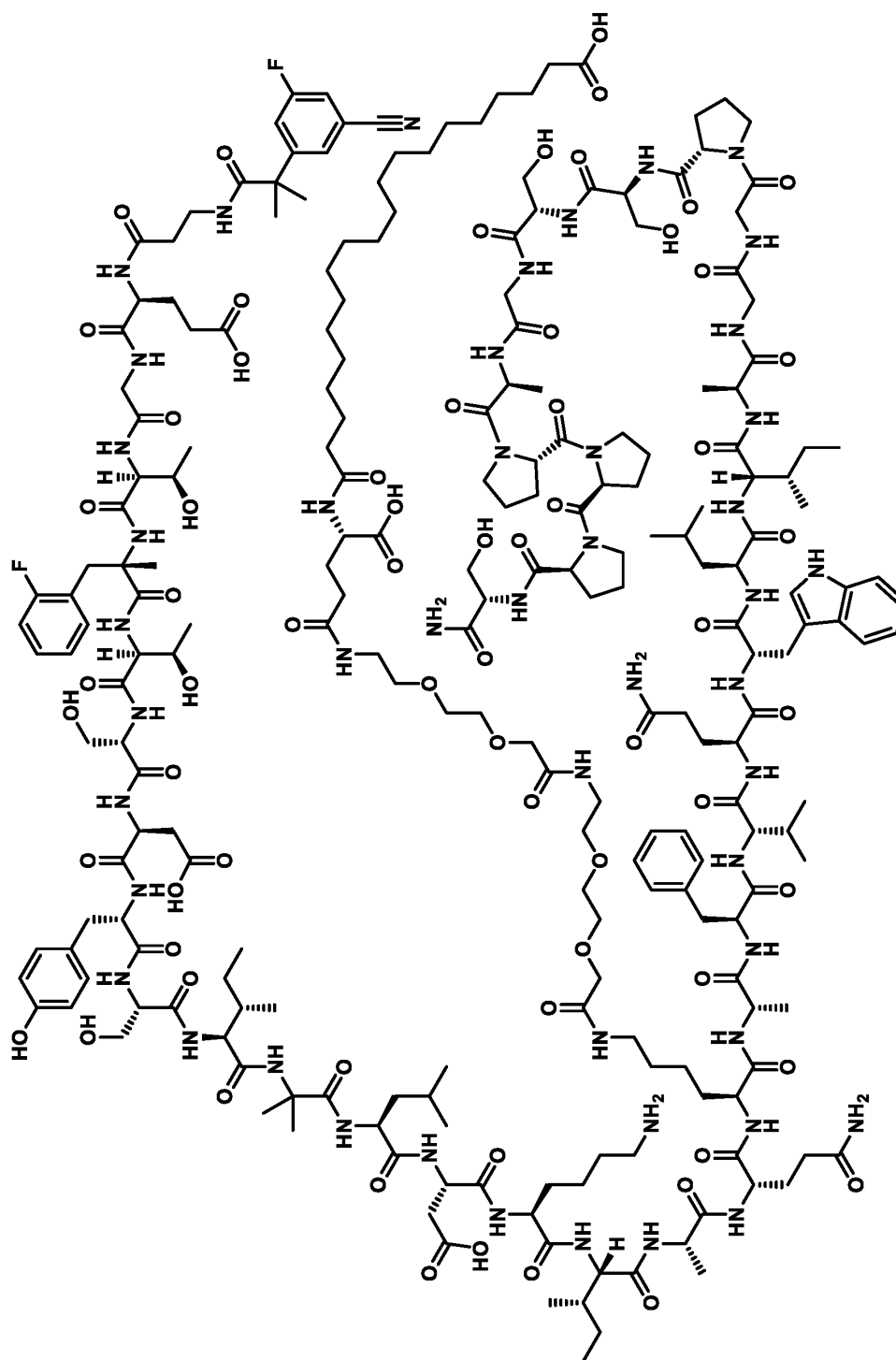
Compound 245
