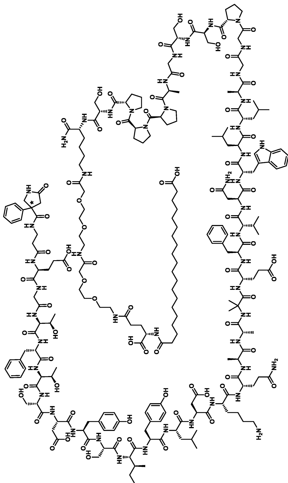
Compound 130
