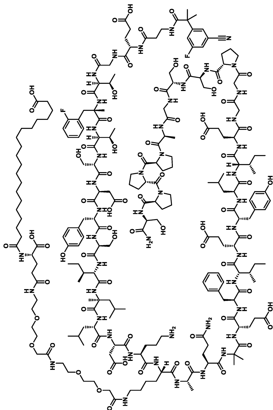
Compound 140
