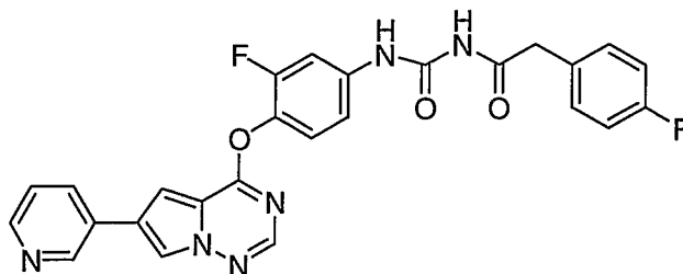
1-(3-Fluoro-4-(6-(pyridin-3-yl)pyrrolo[2,1- f ][1,2,4]triazin-4-yloxy)phenyl)-3-(2-(4-fluorophenyl)acetyl)urea, trifluoroacetic acid salt
