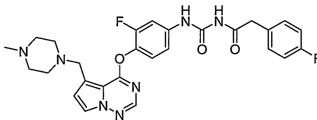
1-(3-Fluoro-4-(5-((4-methylpiperazin-1-yl)methyl)pyrrolo[2,1-f][1,2,4]triazin-4-yloxy)phenyl)-3-(2-(4-fluorophenyl)acetyl)urea
