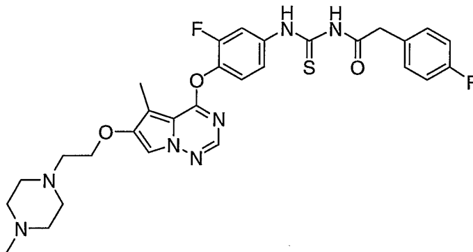
1-(3-Fluoro-4-(5-methyl-6-(2-(4-methylpiperazin-1-yl)ethoxy)pyrrolo[2,1- f ]-[1,2,4]triazin-4-yloxy)phenyl)-3-(2-(4-fluorophenyl)acetyl)thiourea, bis-hydrochloride salt
