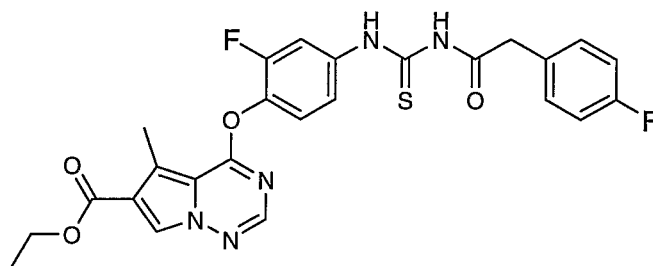
Ethyl 4-(2-fluoro-4-(3-(2-(4-fluorophenyl)acetylthioureido)phenoxy)-5-methylpyrrolo[2,1- f ][1,2,4]triazine-6-carboxylate
