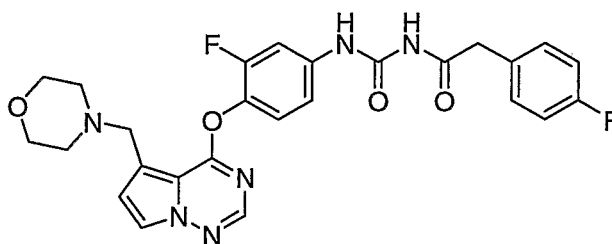
1-(3-Fluoro-4-(5-(morpholinomethyl)pyrrolo[2,1-f][1,2,4]triazin-4-yloxy)phenyl)- 3-(2-(4-fluorophenyl)acetyl)urea
