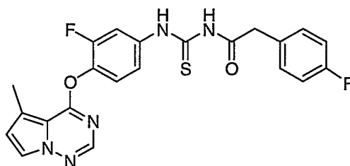
1-(3-Fluoro-4-(5-methylpyrrolo[2,1-f][1,2,4]triazin-4-yloxy)phenyl)-3-(2-(4-fluorophenyl)acetyl)thiourea
