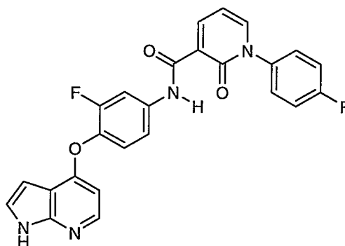
N -(4-(1 H -Pyrrolo[2,3- b ]pyridin-4-yloxy)-3-fluorophenyl)-1-(4-fluorophenyl)-2-oxo-1,2-dihydropyridine-3-carboxamide, trifluoroacetic acid salt
