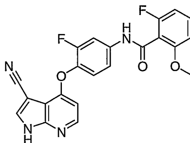
N -(4-(3-Cyano-1 H -pyrrolo[2,3- b ]pyridin-4-yloxy)-3-fluorophenyl)-2-fluoro-6-methoxybenzamide, hydrochloride salt
