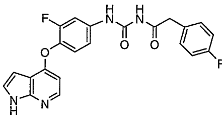
1-(4-(1H-Pyrrolo[2,3-b]pyridin-4-yloxy)-3-fluorophenyl)-3-(2-(4-fluorophenyl)acetyl)urea, hydrochloride salt
