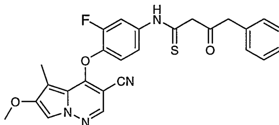
N -(4-(3-Cyano-6-methoxy-5-methyl H -pyrrolo[1,2- b ]pyridazin-4-yloxy)-3-fluorophenyl)-3-oxo-4-phenylbutanethioamide
