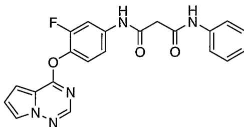
N 1 -(3-Fluoro-4-(pyrrolo[2,1-f][1,2,4]triazin-4-yloxy)phenyl)-N 3 -phenylmalonamide
