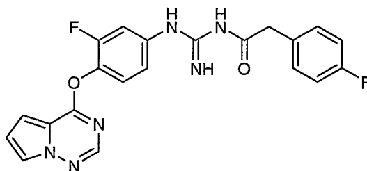
1-(3-Fluoro-4-(pyrrolo[2,1-f][1,2,4]triazin-4-yloxy)phenyl)-3-(2-(4-fluorophenyl)acetyl)guanidine
