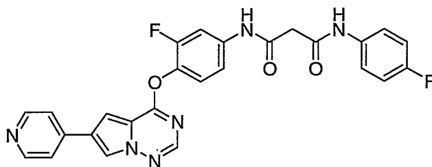
N 1 -(3-Fluoro-4-(6-(pyridin-4-yl)pyrrolo[2,1- f ][1,2,4]triazin-4-yloxy)phenyl)- N 3 -(4-fluorophenyl)malonamide, trifluoroacetic acid salt
