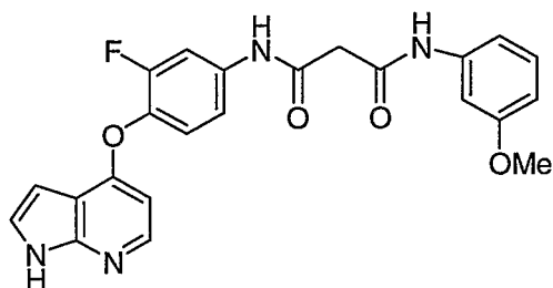
N 1 -(4-(1 H -Pyrrolo[2,3- b ]pyridin-4-yloxy)-3-fluorophenyl)- N 3 -(3-methoxyphenyl)malonamide, trifluoroacetic acid salt
