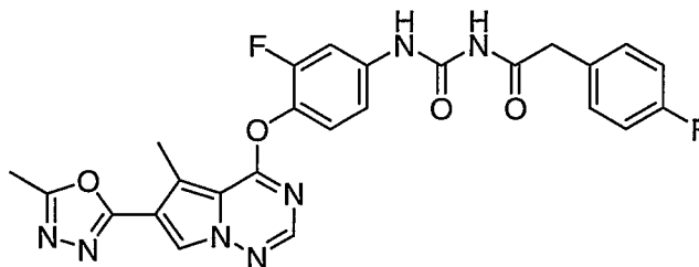
1-(3-Fluoro-4-(5-methyl-6-(5-methyl-1,3,4-oxadiazol-2-yl)pyrrolo[2,1- f][1,2,4]triazin-4-yloxy)phenyl)-3-(2-(4-fluorophenyl)acetyl)urea
