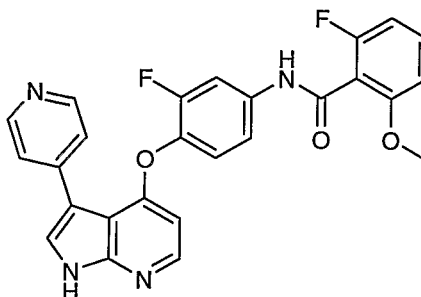
2-Fluoro-N-(3-fluoro-4-(3-(pyridin-4-yl)-1H-pyrrolo[2,3-b]pyridin-4-yloxy)phenyl)-6-methoxybenzamide
