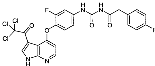
1-(3-Fluoro-4-(3-(2,2,2-trichloroacetyl)-1H-pyrrolo[2,3-b]pyridin-4-yloxy)phenyl)- 3-(2-(4-fluorophenyl)acetyl)urea
