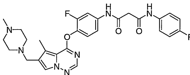
N 1 -(3-Fluoro-4-(5-methyl-6-((4-methylpiperazin-1-yl)methyl)pyrrolo[2,1- f ][1,2,4]triazin-4-yloxy)phenyl)- N 3 -(4-fluorophenyl)malonamide, bis-trifluoroacetic acid salt
