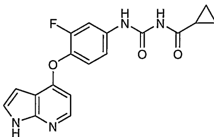
1-(4-(1H-Pyrrolo[2,3-b]pyridin-4-yloxy)-3-fluorophenyl)-3-(cyclopropanecarbonyl)urea
