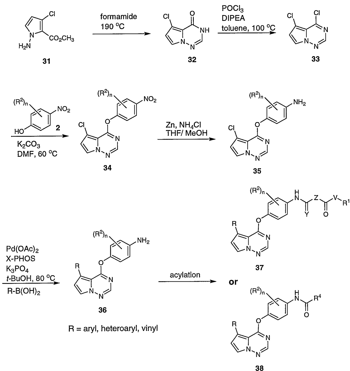
SCHEME 7
