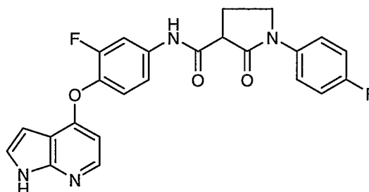
N -(4-(1 H -Pyrrolo[2,3- b ]pyridin-4-yloxy)-3-fluorophenyl)-1-(4-fluorophenyl)-2-oxopyrrolidine-3-carboxamide
