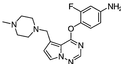
A) 1-(3-Fluoro-4-(5-((4-methylpiperazin-1-yl)methyl)pyrrolo[2,1-f][1,2,4]triazin-4-yloxy)phenyl)-3-(2-(4-fluorophenyl)acetyl)urea
