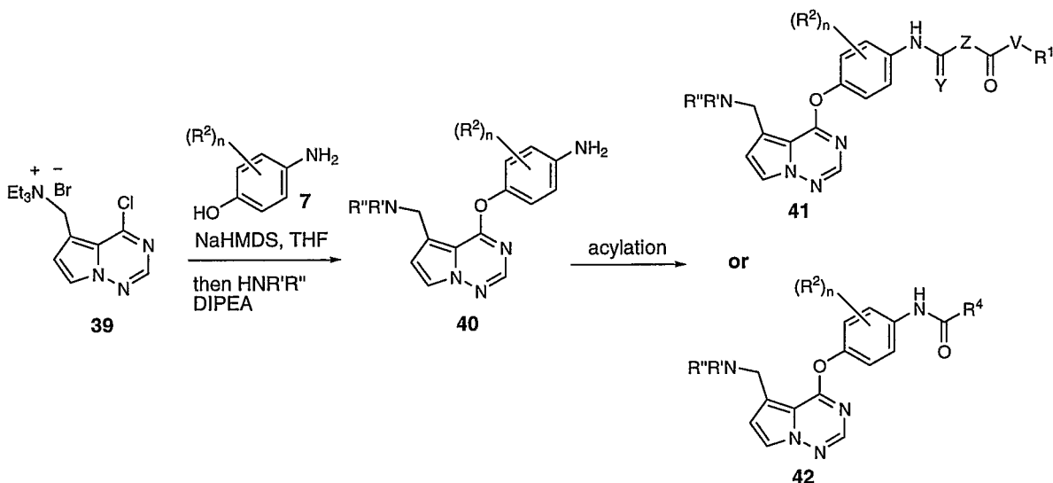
SCHEME 8
