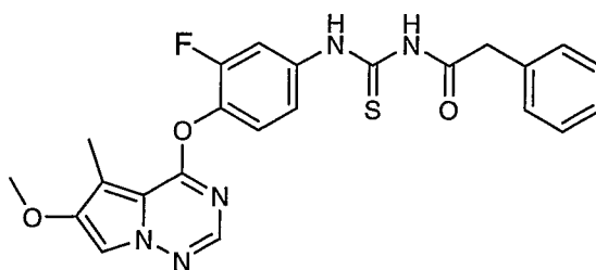
1-(3-Fluoro-4-(6-methoxy-5-methylpyrrolo[2,1-f][1,2,4] triazin-4-yloxy)phenyl)-3-(2-phenylacetyl)thiourea
