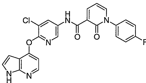
N-(6-(1H-Pyrrolo[2,3- b ]pyridin-4-yloxy)-5-chloropyridin-3-yl)-1-(4-fluorophenyl)-2-oxo-1,2-dihydropyridine-3-carboxamide, trifluoroacetic acid salt
