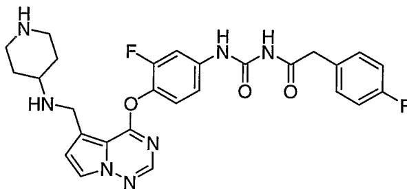
1-(3-Fluoro-4-(5-((piperidin-4-ylamino)methyl)pyrrolo[2,1-f][1,2,4]triazin-4-yloxy)phenyl)-3-(2-(4-fluorophenyl)acetyl)urea
