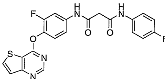
N 1 -(3-Fluoro-4-(thieno[3,2- d ]pyrimidin-4-yloxy)phenyl)- N 3 -(4-fluorophenyl)malonamide
