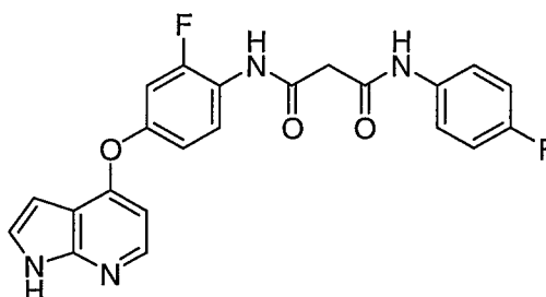
N 1 -(4-(1 H -Pyrrolo[2,3- b ]pyridin-4-yloxy)-2-fluorophenyl)- N 3 -(4-fluorophenyl)malonamide, trifluoroacetic acid salt
