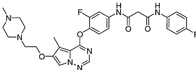
N 1 -(3-Fluoro-4-(5-methyl-6-(2-(4-methylpiperazin-1-yl)ethoxy)pyrrolo[2,1- f ][1,2,4]triazin-4-yloxy)phenyl)- N 3 -(4-fluorophenyl)malonamide, bis-hydrochloride salt
