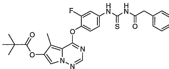
4-(2-Fluoro-4-(3-(2-phenylacetyl)thioureido)phenoxy)-5-methylpyrrolo[2,1-f][1,2,4]triazin-6-yl pivalate
