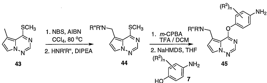
SCHEME 9
