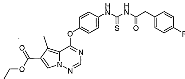
Ethyl 4-(4-(3-(2-(4-fluorophenyl)acetyl)thioureido)phenoxy)-5-methylpyrrolo[2,1-f][1,2,4]triazine-6-carboxylate
