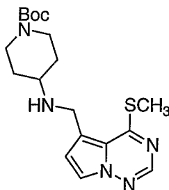
A) tert -Butyl 4-((4-(methylthio)pyrrolo[2,1-f][1,2,4]triazin-5-yl)methylamino)piperidine-1-carboxylate
