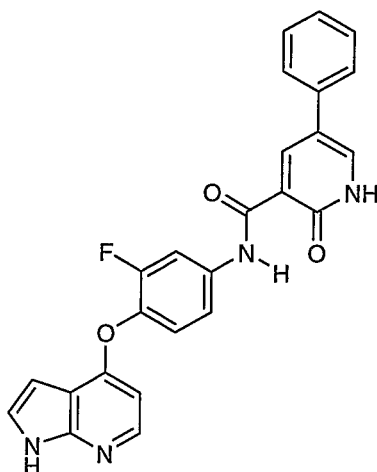
N -(4-(1 H -Pyrrolo[2,3- b ]pyridin-4-yloxy)-3-fluorophenyl)-2-oxo-5-phenyl-1,2-dihydropyridine-3-carboxamide, trifluoroacetic acid salt
