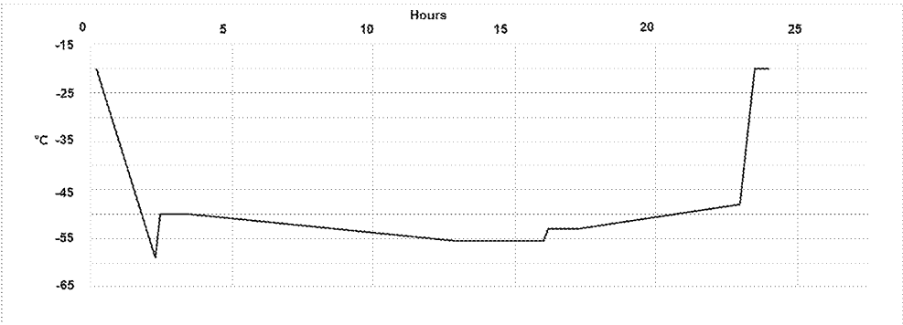
10 Figure 2: Temperature Time Plot for Fractional Crystallisation of example 2
