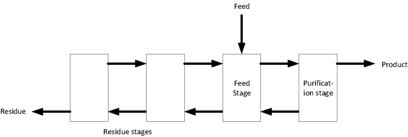
Figure 1: Schematic of Fractional Crystallisation
