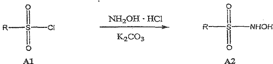
Scheme A. General Synthesis of N -Hydroxysulfonamides.
