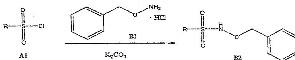
Scheme B. General Synthesis of Intermediate N -Benzyloxysulfonamides.
