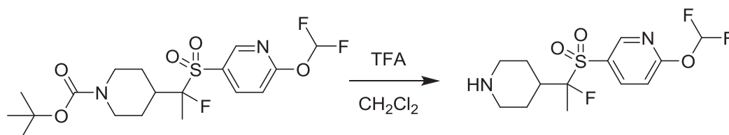
Compound 14.6. 2-(Difluoromethoxy)-5-((1-fluoro-1-(piperidin-4-yl)ethyl)sulfonyl)pyridine
