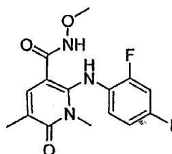
2-(2-fluoro-4-iodophenylamino)-N-methoxy-1,5-dimethyl-6-oxo-1,6-dihydropyridine-3-carboxamide
