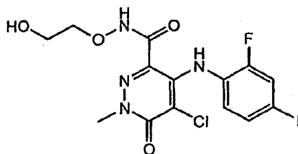
5-Chloro-4-(2-fluoro-4-iodophenylamino)-N-(2-hydroxyethoxy)-1-methyl-6-oxo-1,6-dihydropyridazine-3-carboxamide
