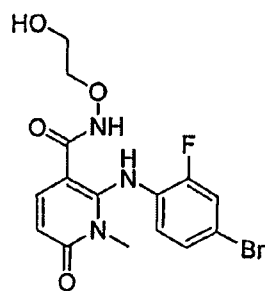
2-(4-bromo-2-fluorophenylamino)-N-(2-hydroxyethoxy)-1-methyl-6-oxo-1,6-dihydropyridine-3-carboxamide
