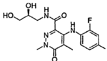
(S)-N-(2,3-Dihydroxypropyl)-4-(2-fluoro-4-iodophenylamino)-1,5-dimethyl-6-oxo-1,6-dihydropyridazine-3-carboxamide
