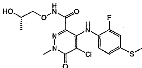
(S)-5-Chloro-4-(2-fluoro-4-(methylthio)phenylamino)-N-(2-hydroxypropoxy)-1-methyl-6-oxo-1,6-dihydropyridazine-3-carboxamide
