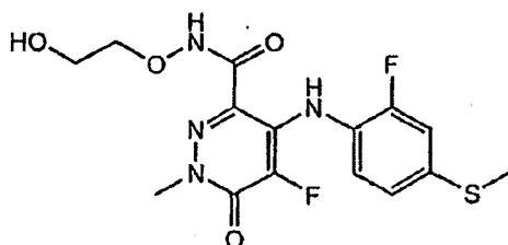
5-Fluoro-4-(2-fluoro-4-methylthio)phenylamino)-N-(2-hydroxyethoxy)-1-methyl-6-oxo-1,6-dihydropyridazine-3-carboxamide
