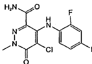
5-Chloro-4-(2-fluoro-4-iodophenylamino)-1-methyl-6-oxo-1,6-dihydropyridazine-3-carboxamide
