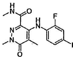
4-(2-Fluoro-4-iodophenylamino)-N,1,5-trimethyl-6-oxo-1,6-dihydropyridazine-3-carboxamide
