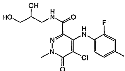
5-Chloro-N-(2,3-dihydroxypropyl)-4-(2-fluoro-4-iodophenylamino)-1-methyl-6-oxo-1,6-dihydropyridazine-3-carboxamide
