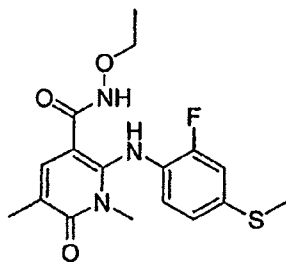
N-ethoxy-2-(2-fluoro-4-(methylthio)phenylamino)-1,5-dimethyl-6-oxo-1,6-dihydropyridine-3-carboxamide
