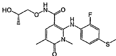
(S)-2-(2-fluoro-4-(methylthio)phenylamino)-N-(2-hydroxypropoxy)-1,5-dimethyl-6-oxo-1,6-dihydropyridine-3-carboxamide
