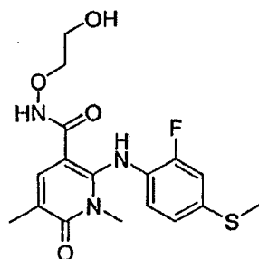
2-(2-fluoro-4-(methylthio)phenylamino)-N-(2-hydroxyethoxy)-1,5-dimethyl-6-oxo-1,6-dihydropyridine-3-carboxamide
