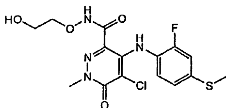
5-Chloro-4-(2-fluoro-4-(methylthio)phenylamino)-N-(2-hydroxyethoxy)-1-methyl-6-oxo-1,6-dihydropyridazine-3-carboxamide
