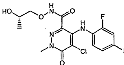
(S)-5-Chloro-4-(2-fluoro-4-iodophenylamino)-N-(2-hydroxypropoxy)-1-methyl-6-oxo-1,6-dihydropyridazine-3-carboxamide
