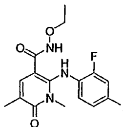
N-ethoxy-2-(2-fluoro-4-iodophenylamino)-1,5-dimethyl-6-oxo-1,6-dihydropyridine-3-carboxamide
