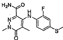
4-(2-Fluoro-4-(methylthio)phenylamino)-1,5-dimethyl-6-oxo-1,6-dihydropyrazine-3-carboxamide
