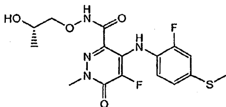
(S)-5-Fluoro-4-(2-fluoro-4-(methylthio)phenylamino)-N-(2-hydroxypropoxy)-1-methyl-6-oxo-1,6-dihydropyridazine-3-carboxamide
