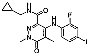
N-(Cyclopropylmethyl)-4-(2-fluoro-4-iodophenylamino)-1,5-dimethyl-6-oxo-1,6-dihydropyridazine-3-carboxamide
