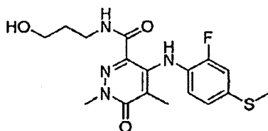
4-(2-Fluoro-4-(methylthio)phenylamino)-N-(3-hydroxypropyl)-1,5-dimethyl-6-oxo-1,6-dihydropyridazine-3-carboxamide
