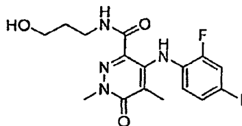
4-(2-Fluoro-4-iodophenylamino)-N-(3-hydroxypropyl)-1,5-dimethyl-6-oxo-1,6-dihydropyridazine-3-carboxamide
