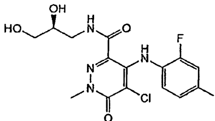
(S)-5-Chloro-N-(2,3-dihydroxypropyl)-4-(2-fluoro-4-iodophenylamino)-1-methyl-6-oxo-1,6-dihydropyridazine-3-carboxamide
