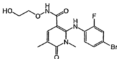
2-(4-Bromo-2-fluorophenylamino)-N-(2-hydroxyethoxy)-1,5-dimethyl-6-oxo-1,6-dihydropyridine-3-carboxamide
