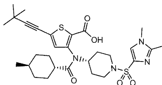
Compound 206
