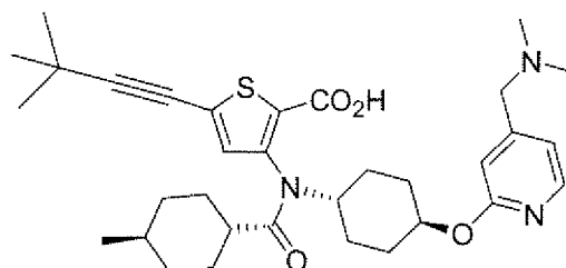
Compound 29
