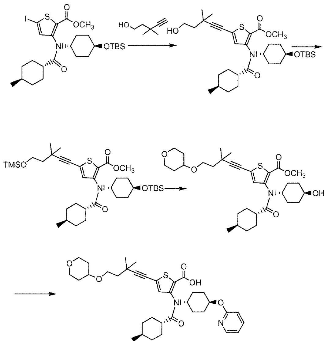
Compound 319
