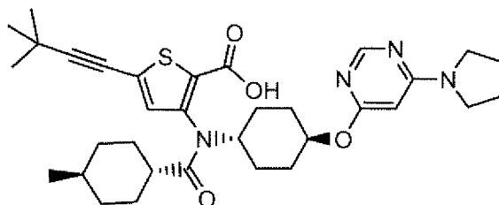
Compound 150
