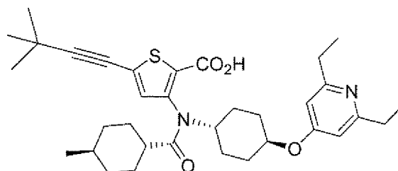
Compound 26
