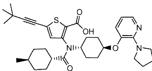
Compound 149
