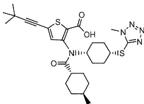
Compound 104
