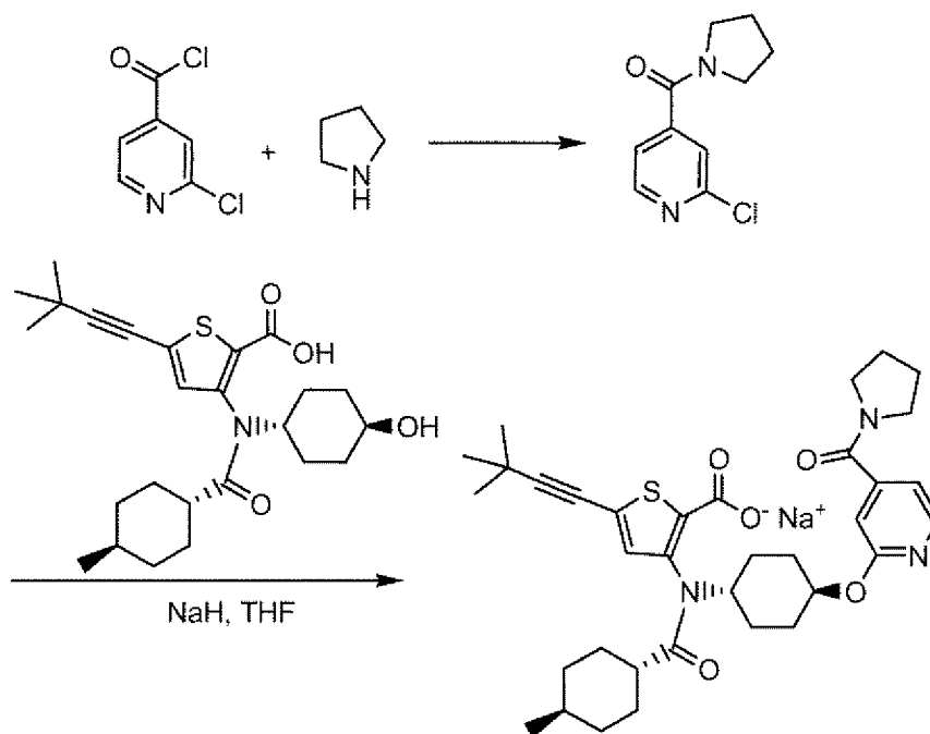
Compound 166
