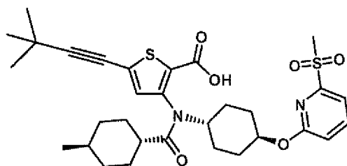
Compound 6
