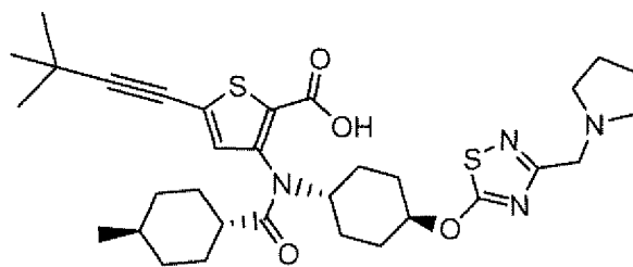
Compound 161
