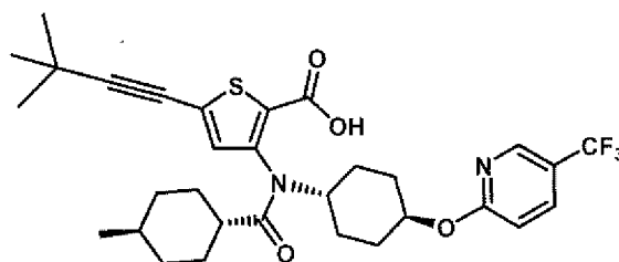
Compound 10
