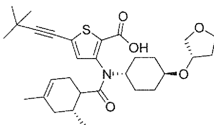
Compound 304
