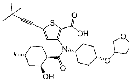
Compound 228
