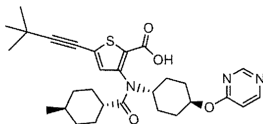
Compound 163
