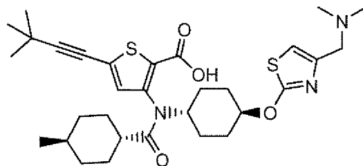
Compound 156
