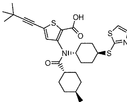
Compound 106
