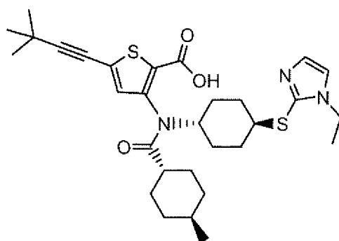
Compound 89
