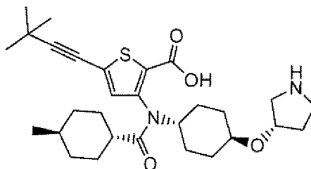
Compound 226
