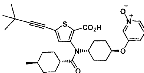
Compound 24
