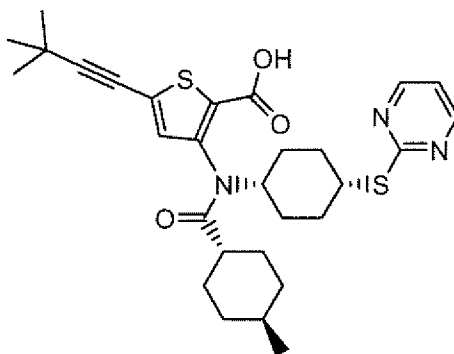
Compound 108
