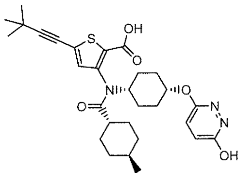
Compound 178
