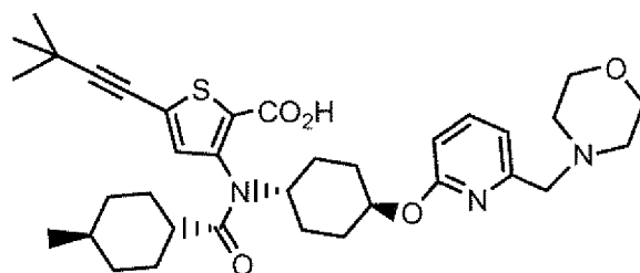
Compound 188
