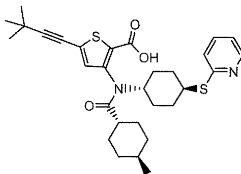
Compound 99
