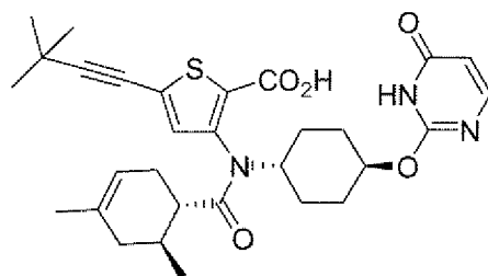
Compound 357
