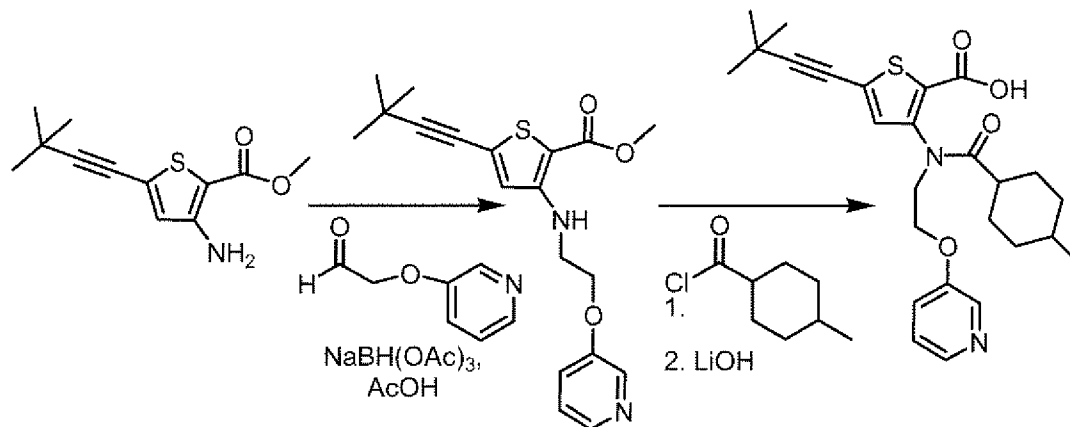
Compound 138
