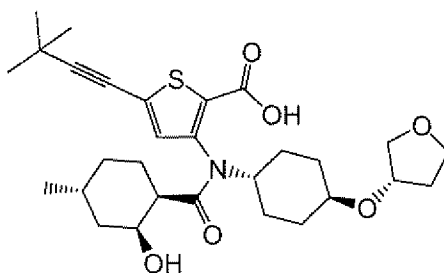
Compound 309
