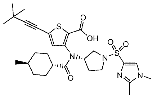
Compound 212
