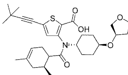
Compound 308
