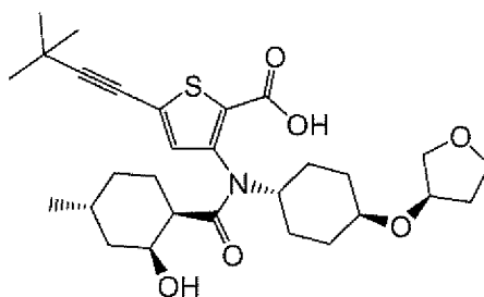
Compound 310
