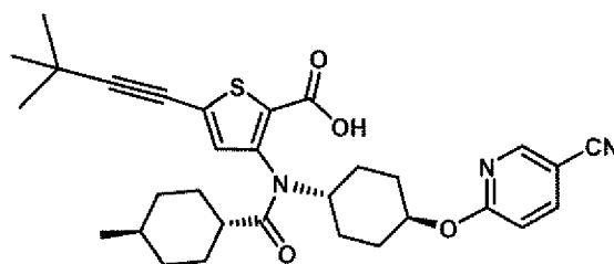
Compound 9
