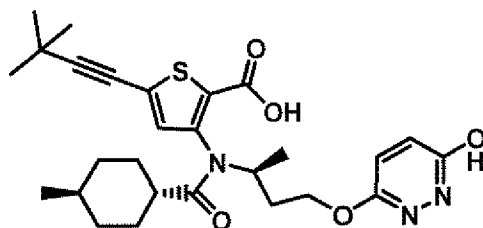
Compound 63
