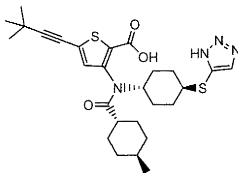
Compound 96
