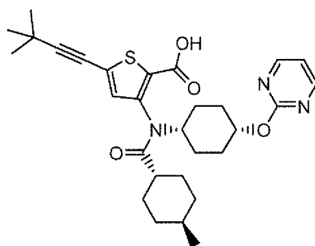
Compound 181
