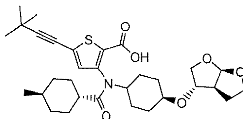
Compound 221
