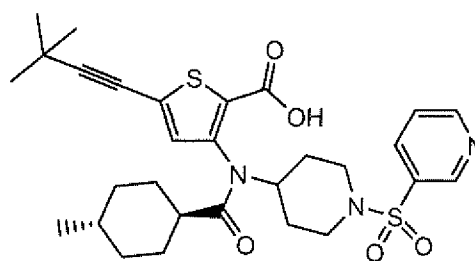
Compound 210
