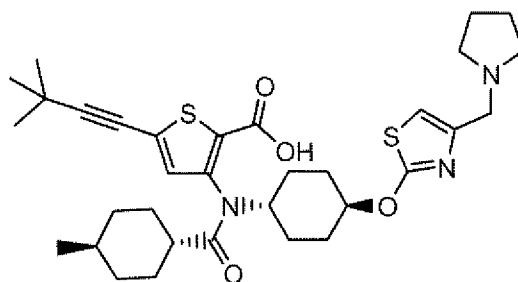
Compound 155
