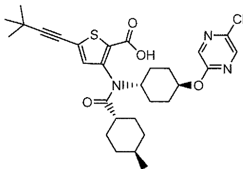
Compound 184
