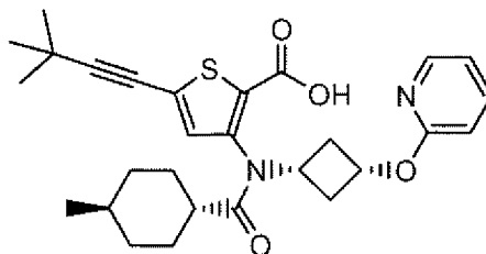
Compound 146
