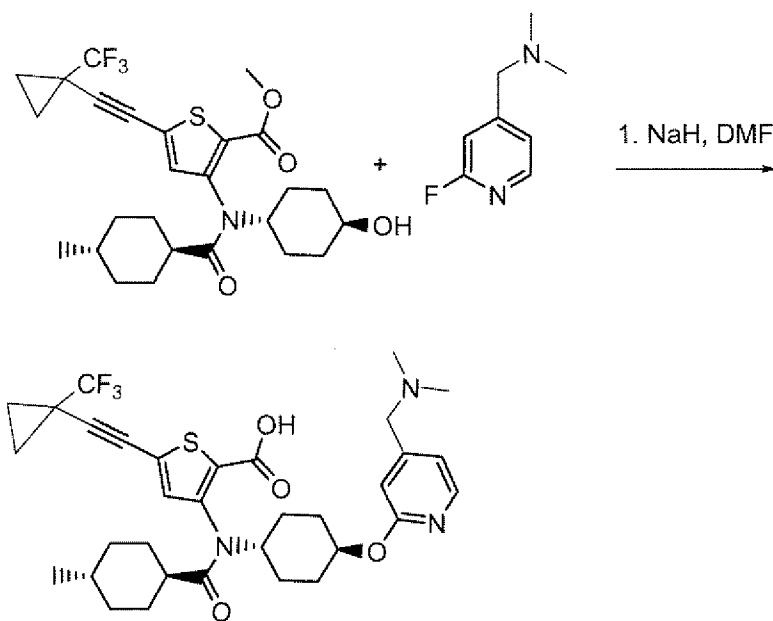
Compound 340
