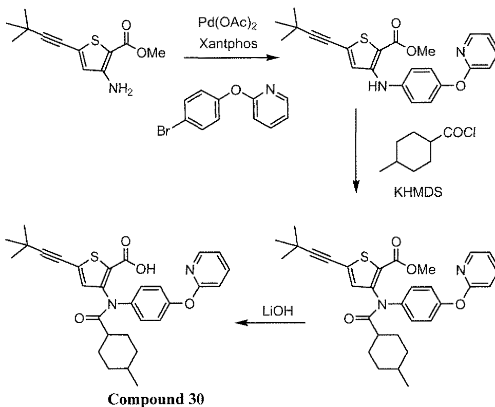
Scheme 5
