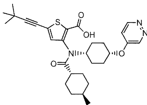
Compound 183
