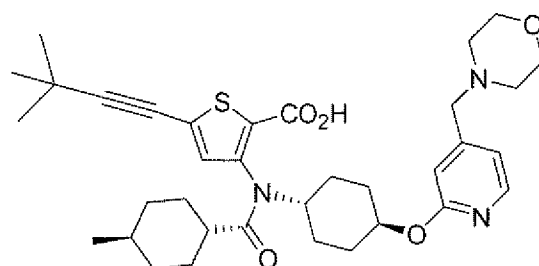
Compound 28
