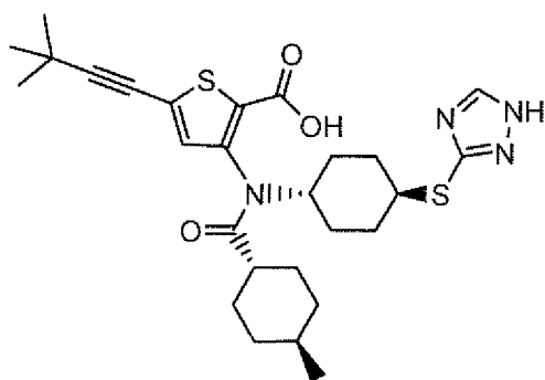
Compound 97
