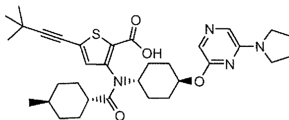
Compound 153
