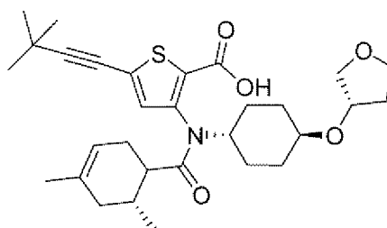
Compound 303
