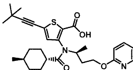
Compound 60
