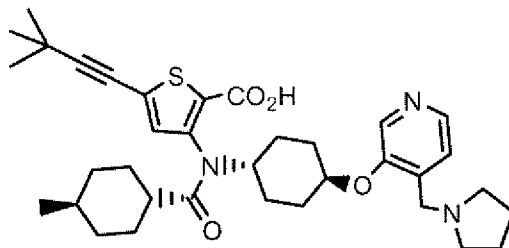
Compound 196
