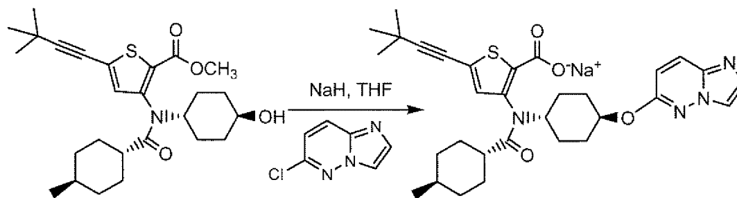
Compound 176
