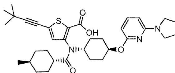
Compound 152
