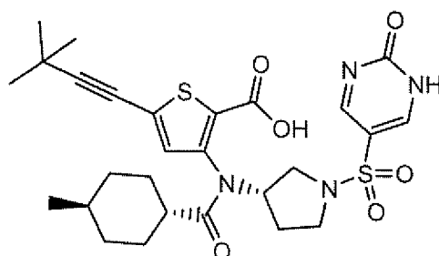
Compound 214
