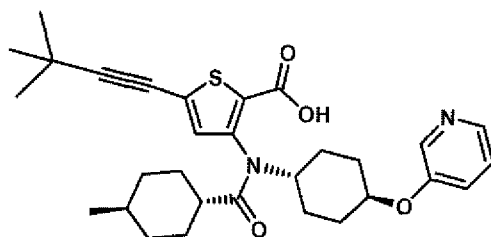
Compound 5
