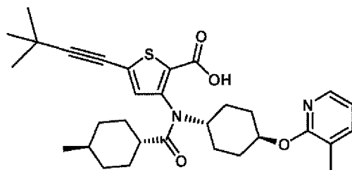
Compound 12
