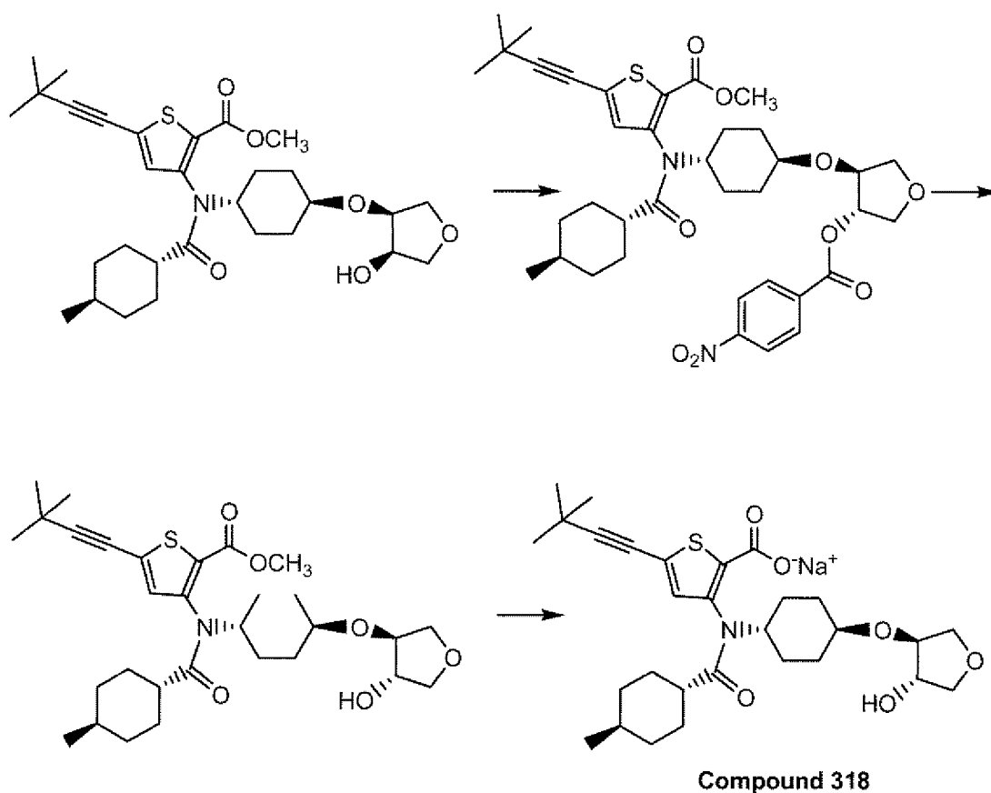
Scheme 9
