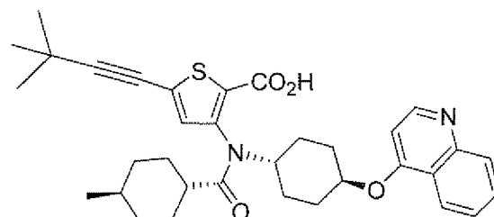
Compound 25
