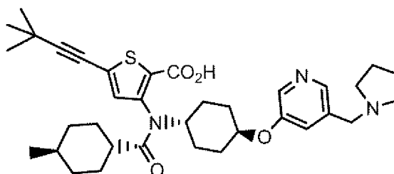
Compound 193
