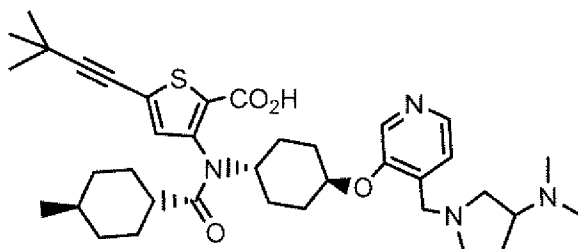
Compound 195
