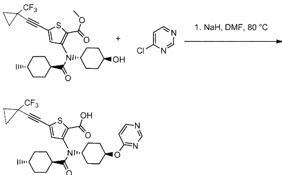
Compound 344
