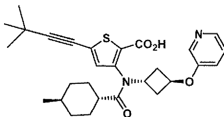
Compound 21
