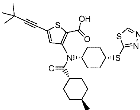
Compound 105
