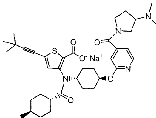
Compound 169
