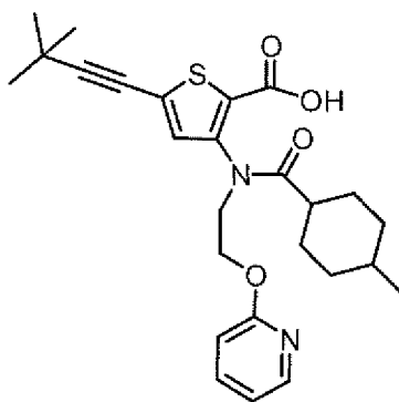
Compound 139
