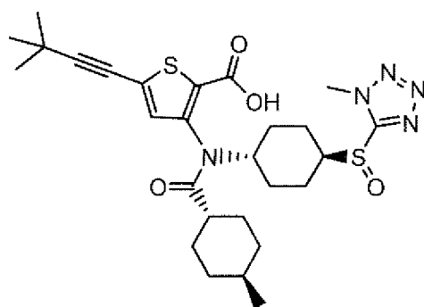
Compound 111
