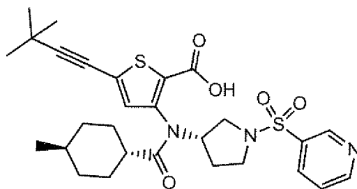
Compound 216
