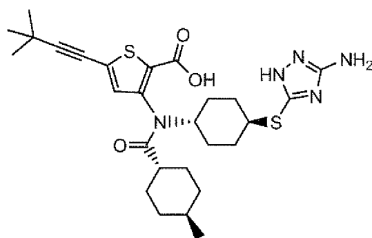
Compound 95
