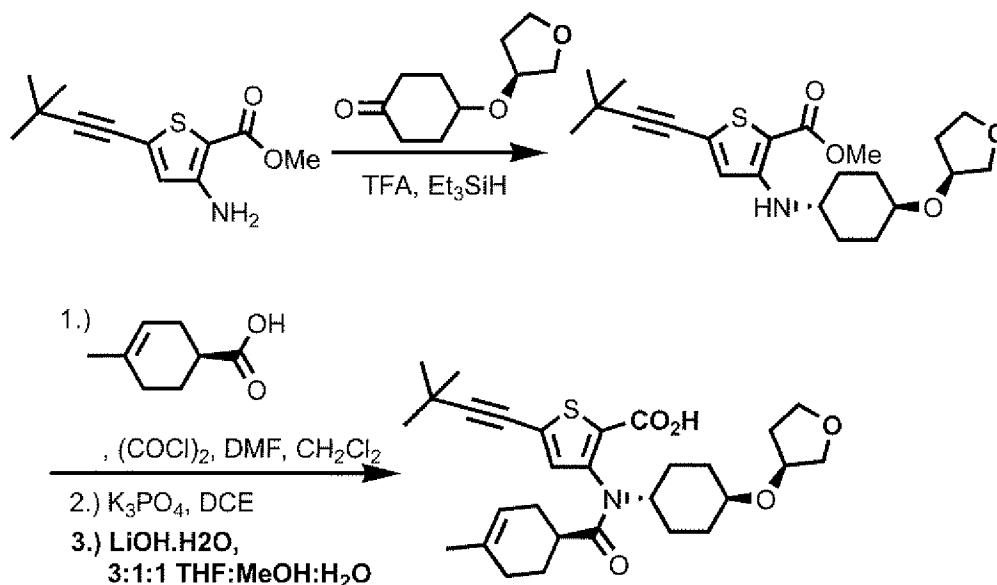
Scheme 18
