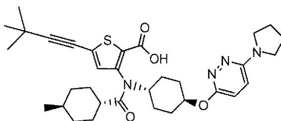
Compound 159
