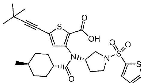
Compound 213
