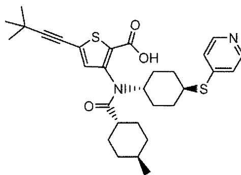
Compound 87
