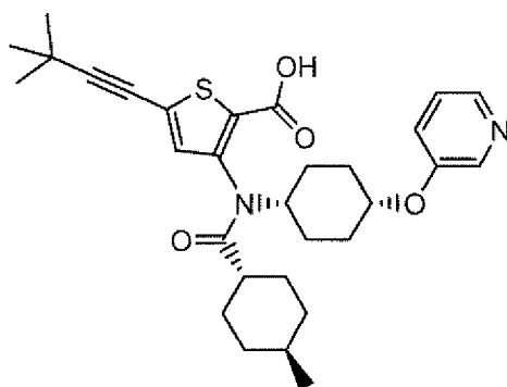
Compound 180
