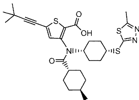
Compound 103
