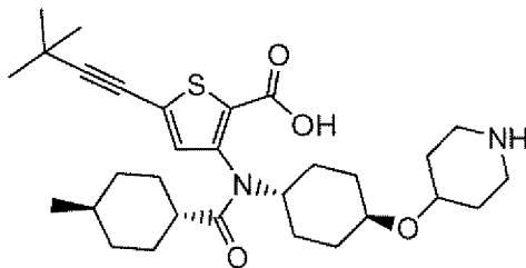
Compound 223
