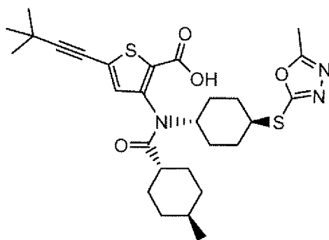
Compound 98
