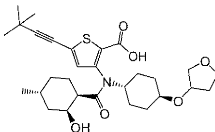
Compound 227
