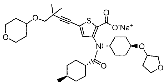
Compound 355
