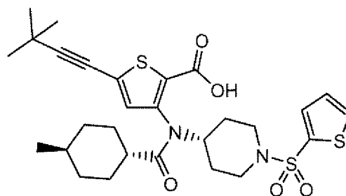
Compound 207
