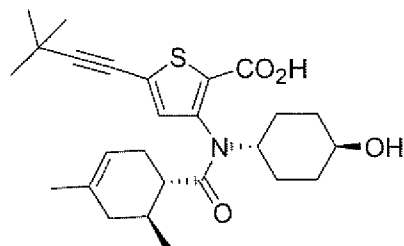
Scheme 1
