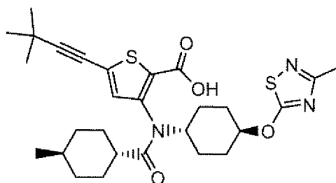
Compound 154
