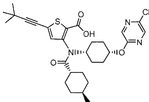
Compound 182
