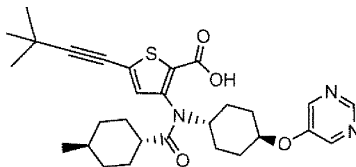
Compound 162
