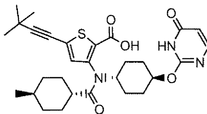
Compound 326
