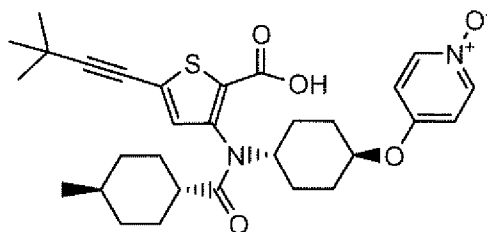
Compound 157
