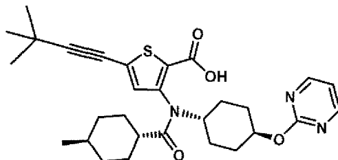
Compound 4
