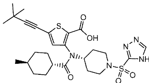
Compound 202
