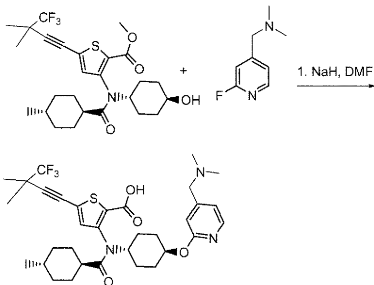
Scheme 23
