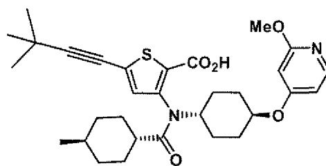
Compound 19
