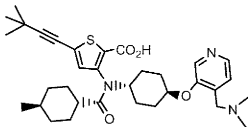
Compound 198
