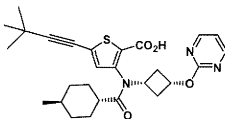
Compound 22
