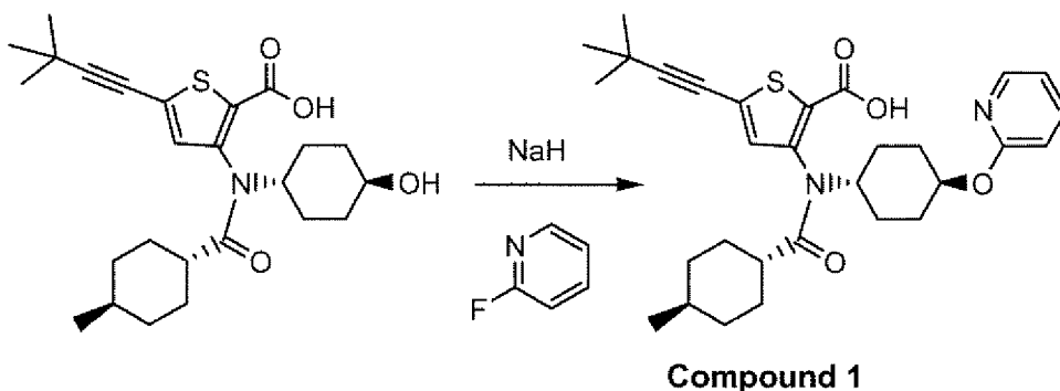
15 Scheme 1
