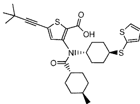
Compound 93
