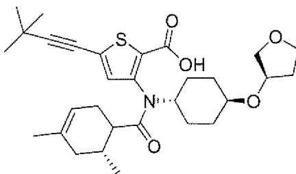
Compound 306
