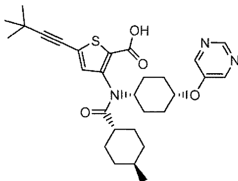
Compound 179
