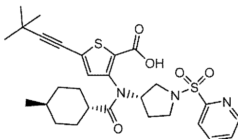
Compound 215
