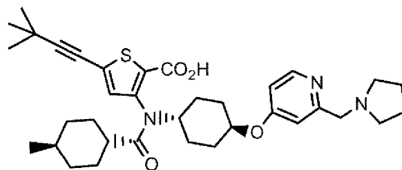
Compound 199
