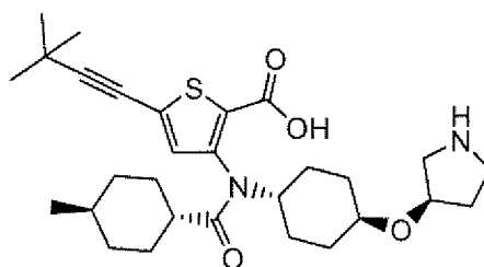
Compound 231
