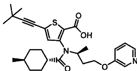
Compound 58
