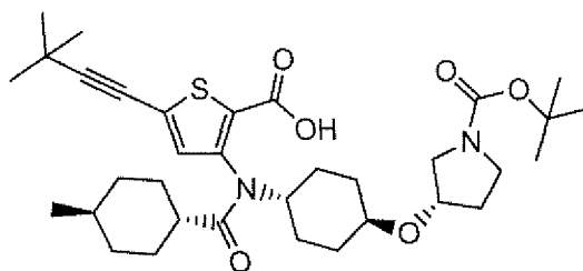
Compound 225
