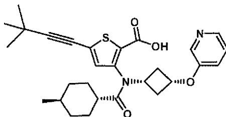
Compound 20
