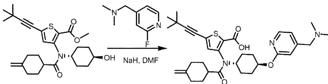
Compound 325
