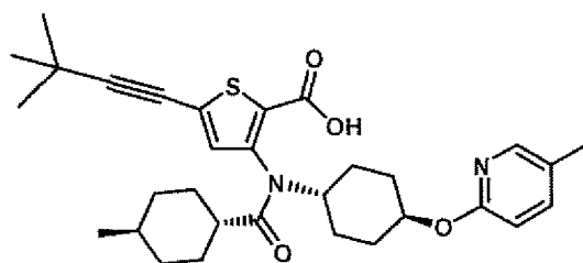
Compound 11
