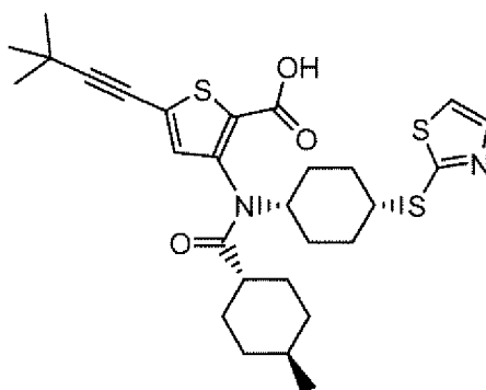
Compound 107
