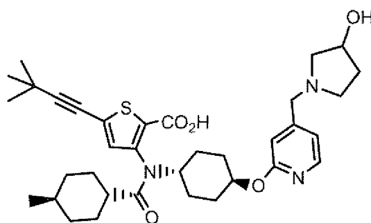
Compound 190
