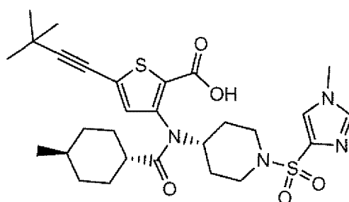
Compound 201
