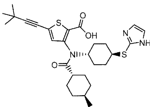
Compound 94
