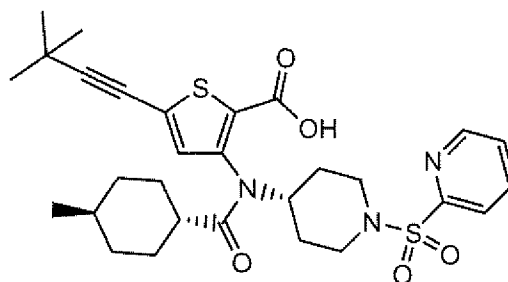
Compound 209
