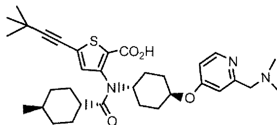
Compound 200
