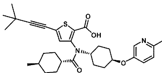
Compound 7
