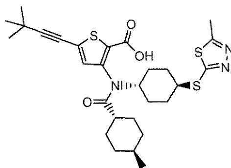
Compound 102
