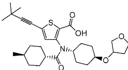
Compound 224
