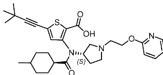
Compound 321
