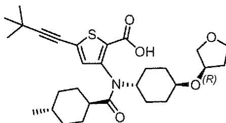
Compound 322
