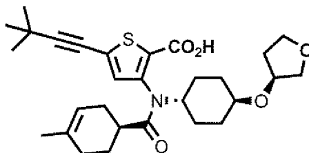
Compound 333
