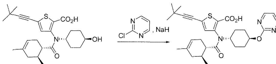
Compound 349
