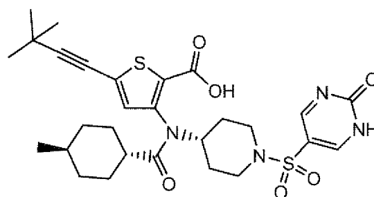
Compound 208
