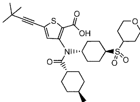
Compound 109
