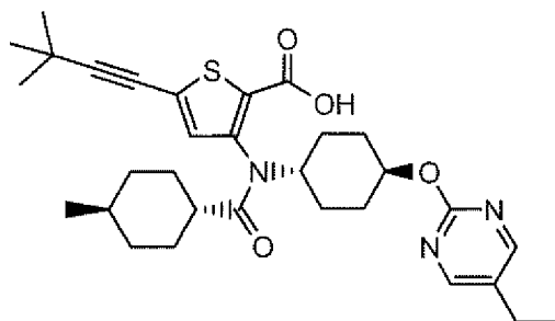
Compound 148
