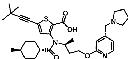
Compound 62
