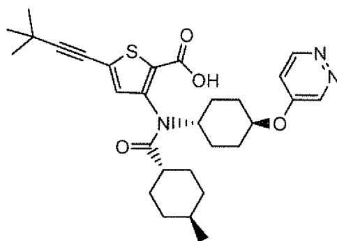
Compound 185
