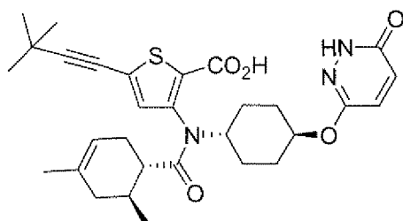
Compound 356
