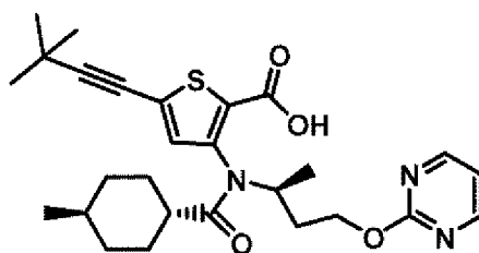
Compound 59
