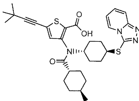
Compound 92
