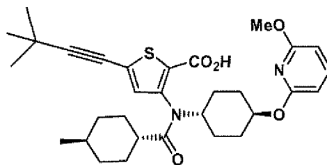
Compound 18
