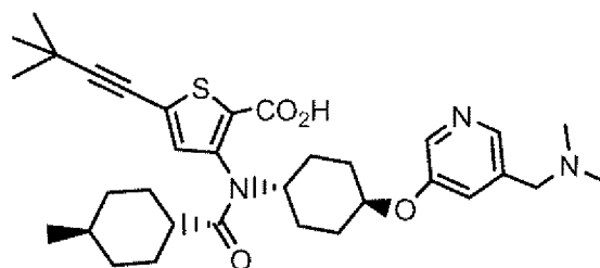
Compound 192
