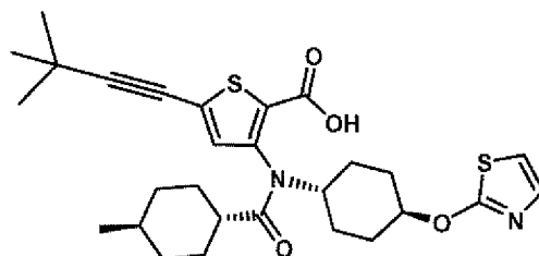
Compound 15
