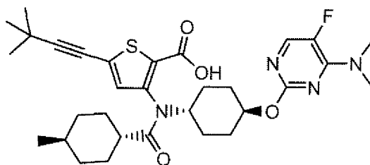
Compound 151
