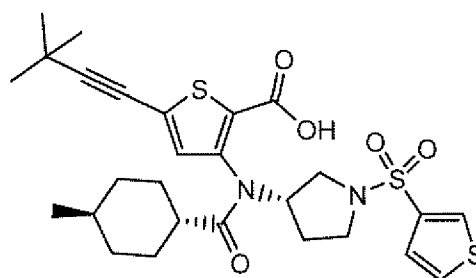
Compound 211
