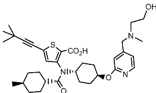
Compound 191
