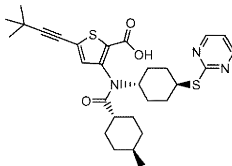
Compound 100
