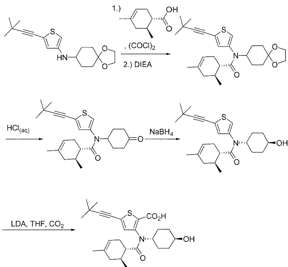
Scheme 1
