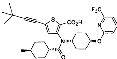
Compound 17
