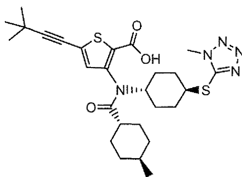
Compound 101
