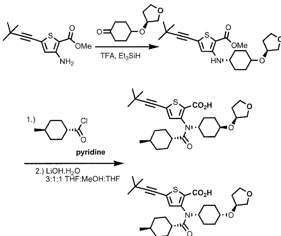
Scheme 17
