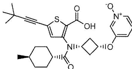
Compound 145
