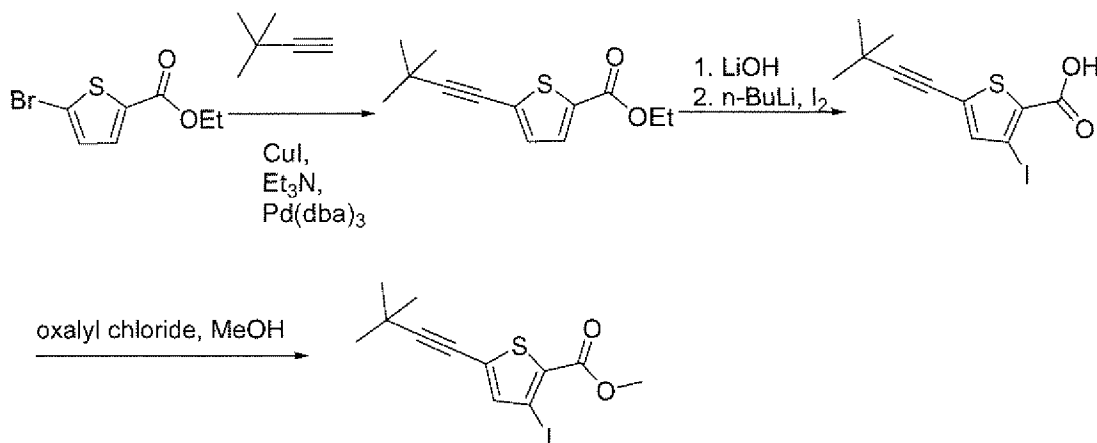
Scheme 8
