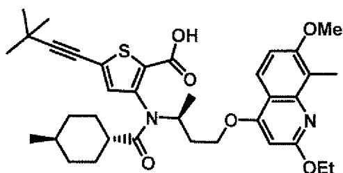
Compound 144
