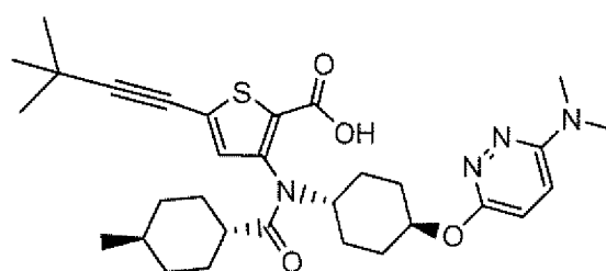
Compound 160
