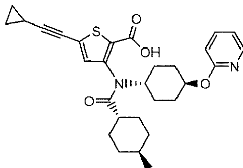
Compound 229
