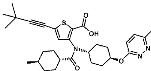
Compound 3
