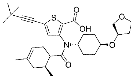
Compound 307
