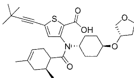
Compound 302
