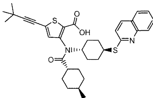
Compound 91
