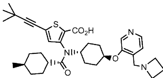
Compound 197
