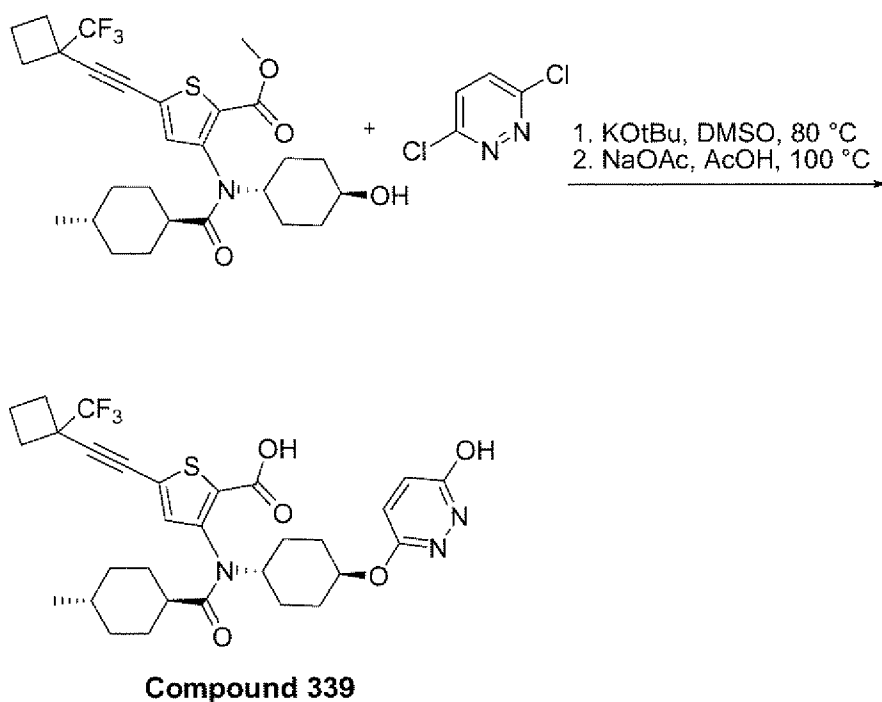
Scheme 21
