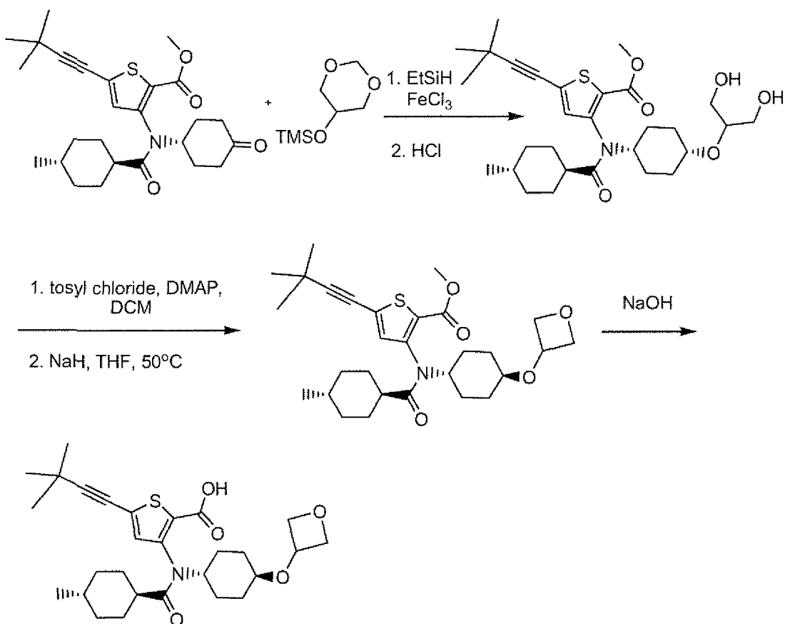
Compound 347
