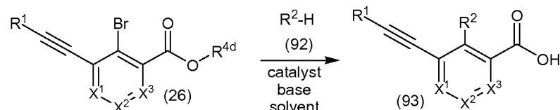
Scheme 21
