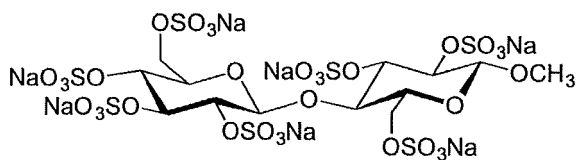
methyl 2,2',3,3',4',6,6'-hepta-O-sulfo- \beta -cellobioside (methyl \beta -cellobioside per-O-sulfate, mCBS,
