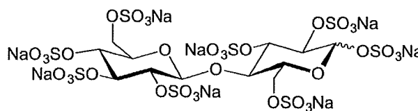
1,2,2',3,3',4',6,6'-octa-O-sulfo- \alpha,\beta -cellobiose, (cellobiose per-O-sulfate, CBS)
