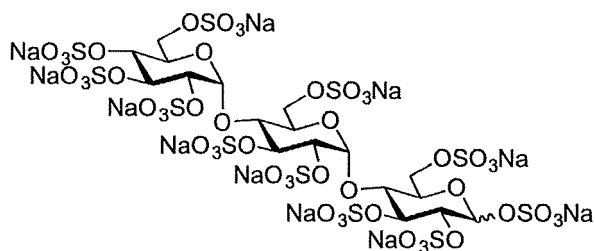
1,2',2'',3,3',3'',3''',4'',6,6',6'',6'''-undeca-O-sulfo- \alpha,\beta -maltotriose (maltotriose per-O-sulfate, MTS)
