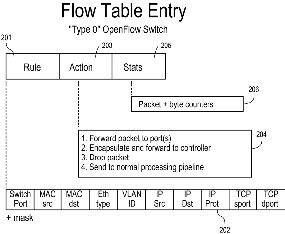
FIG. 2 (PRIOR ART)
