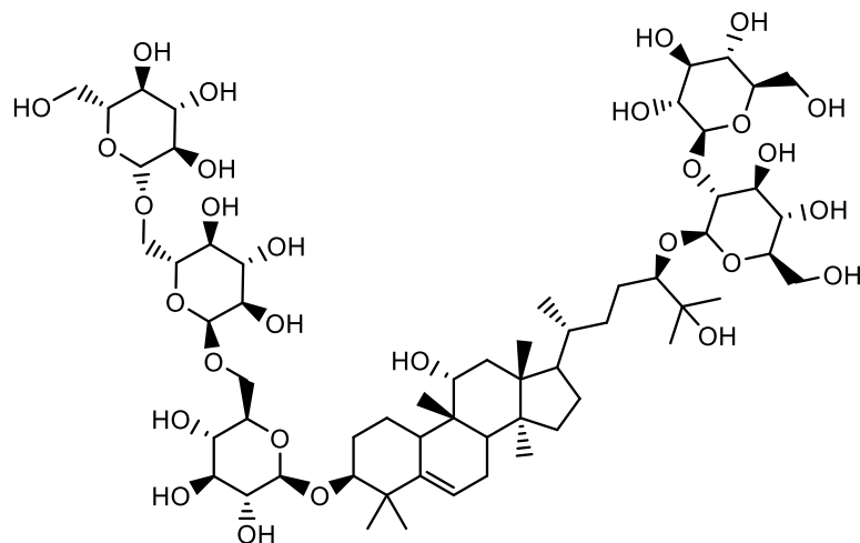
Compound 33
