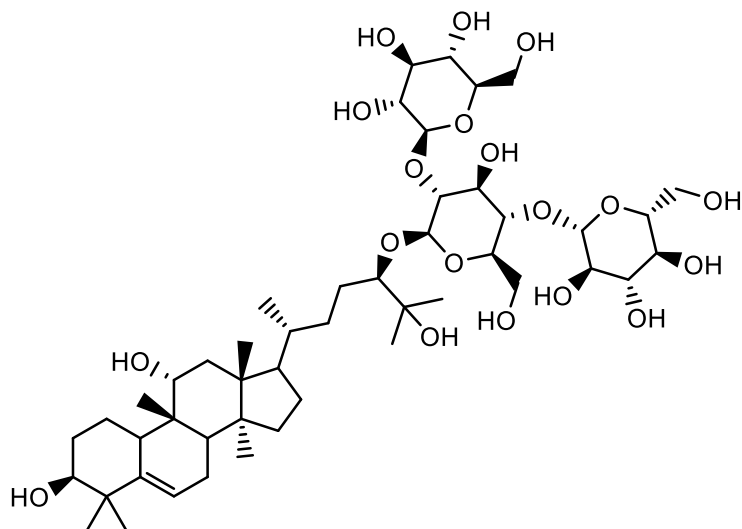
Compound 35
