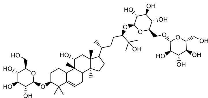
Mogroside III
