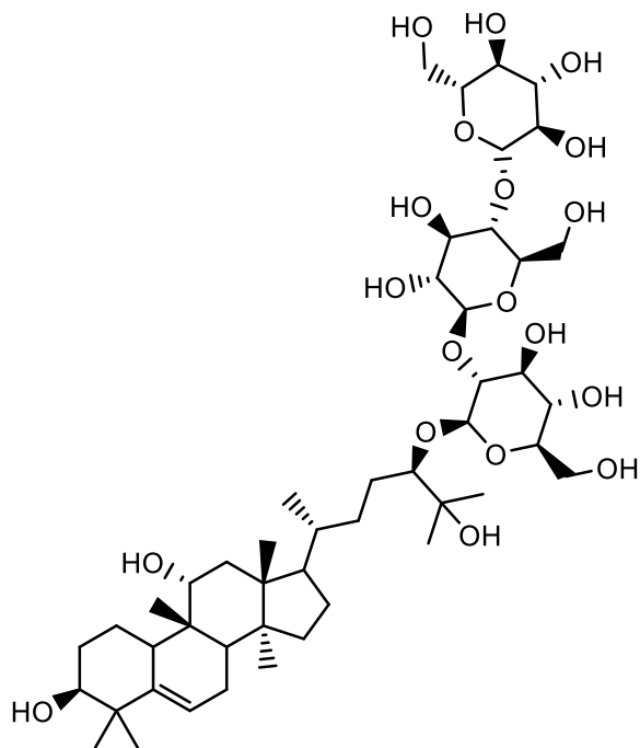
Compound 34
