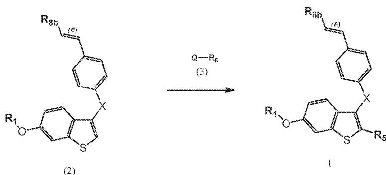
General Reaction Scheme II:
