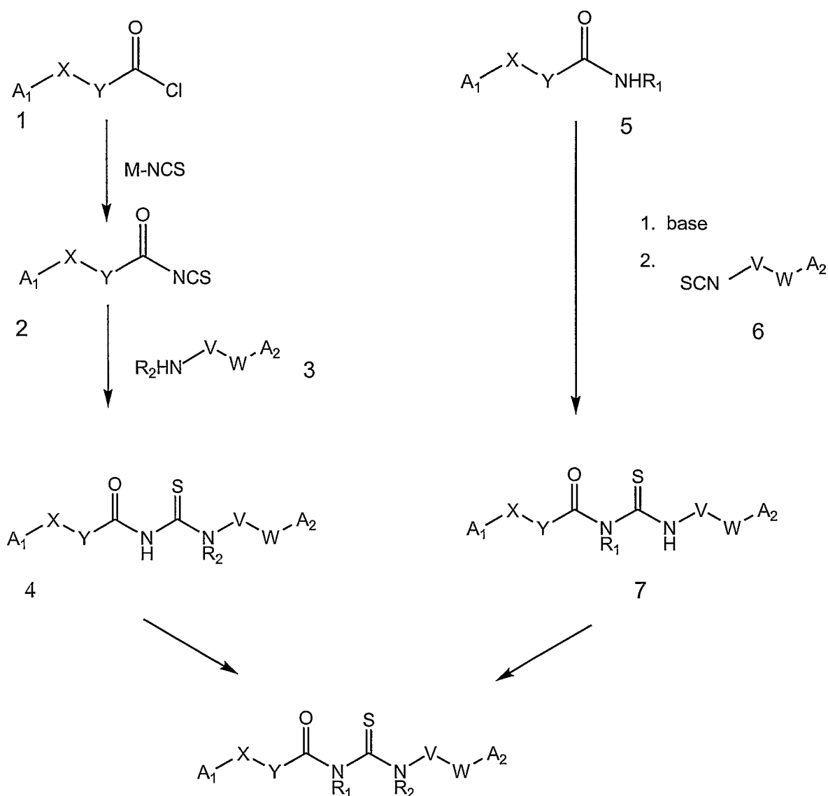
Scheme I
