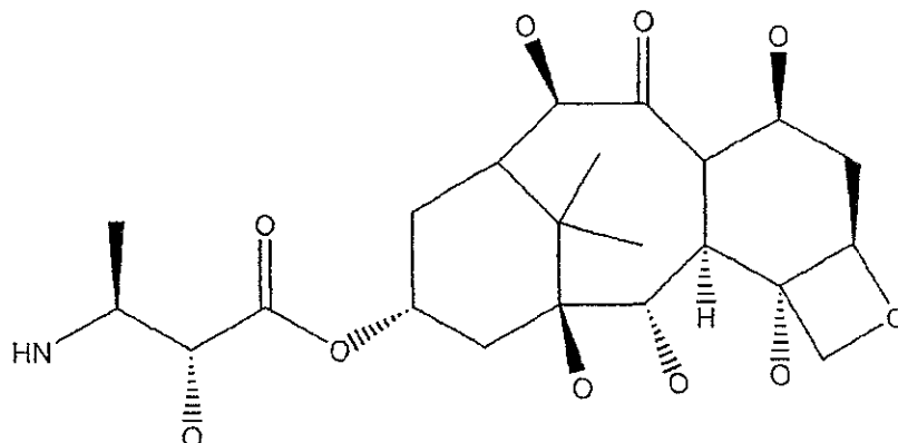
(XXVI).
