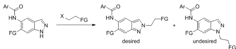
5 Scheme 1: N-alkylation of 1H-indazoles
