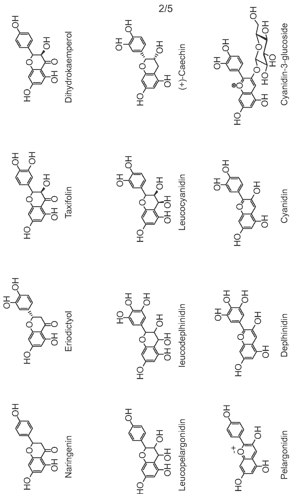
FIG. 2 Structures of the flavonoid and anthocyanin molecules produced
