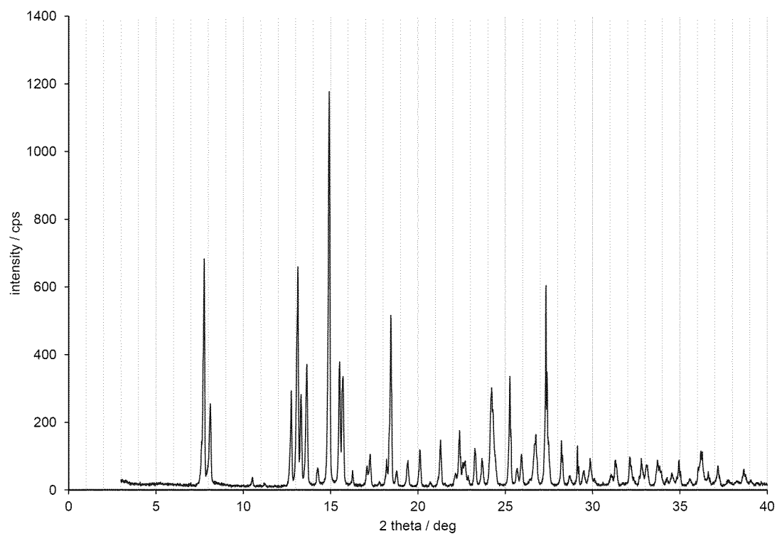
Figure 1: pXRD for Crystalline, Monohydrate (S)-CSA salt of S-Ketamine
