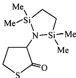
Thiolactone-NSi 2
