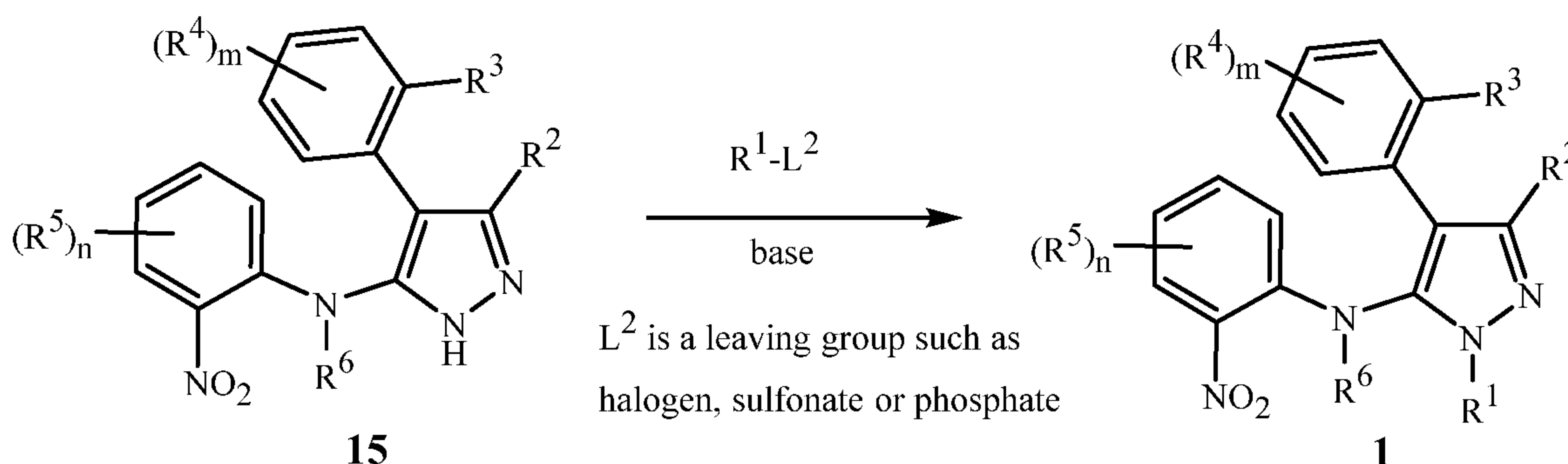
Scheme 7
