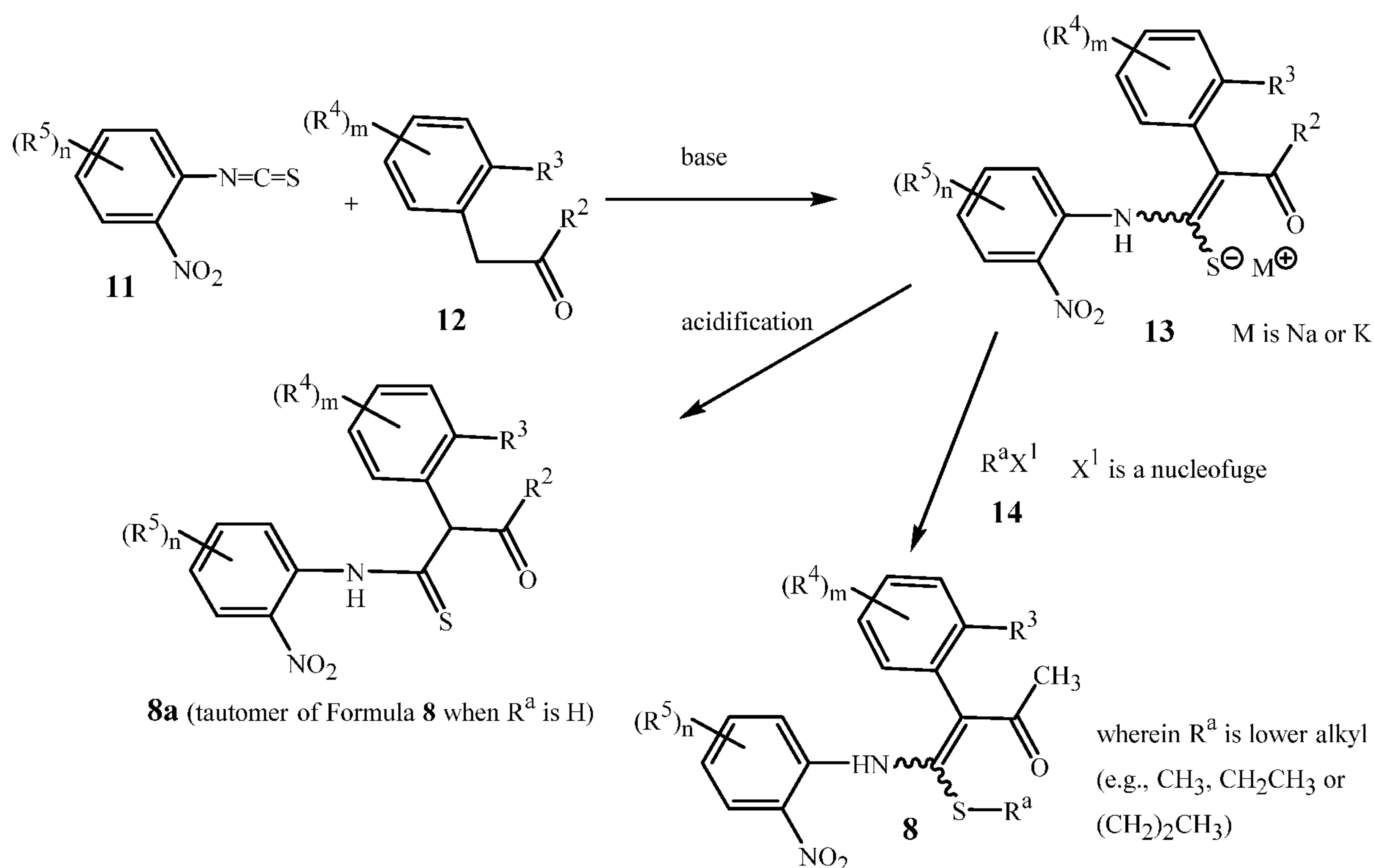
Scheme 6
