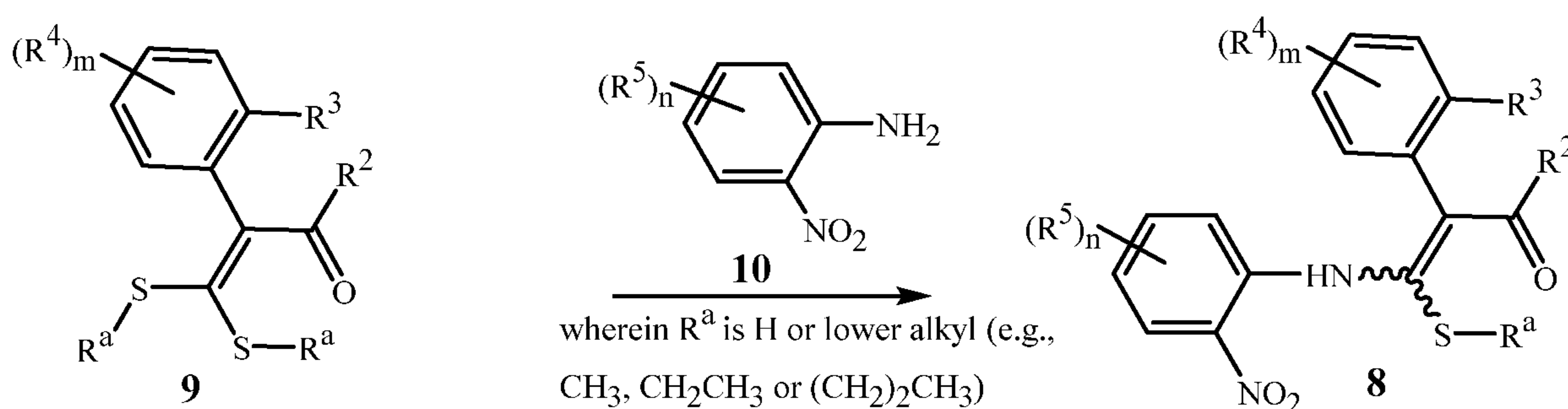
Scheme 5
