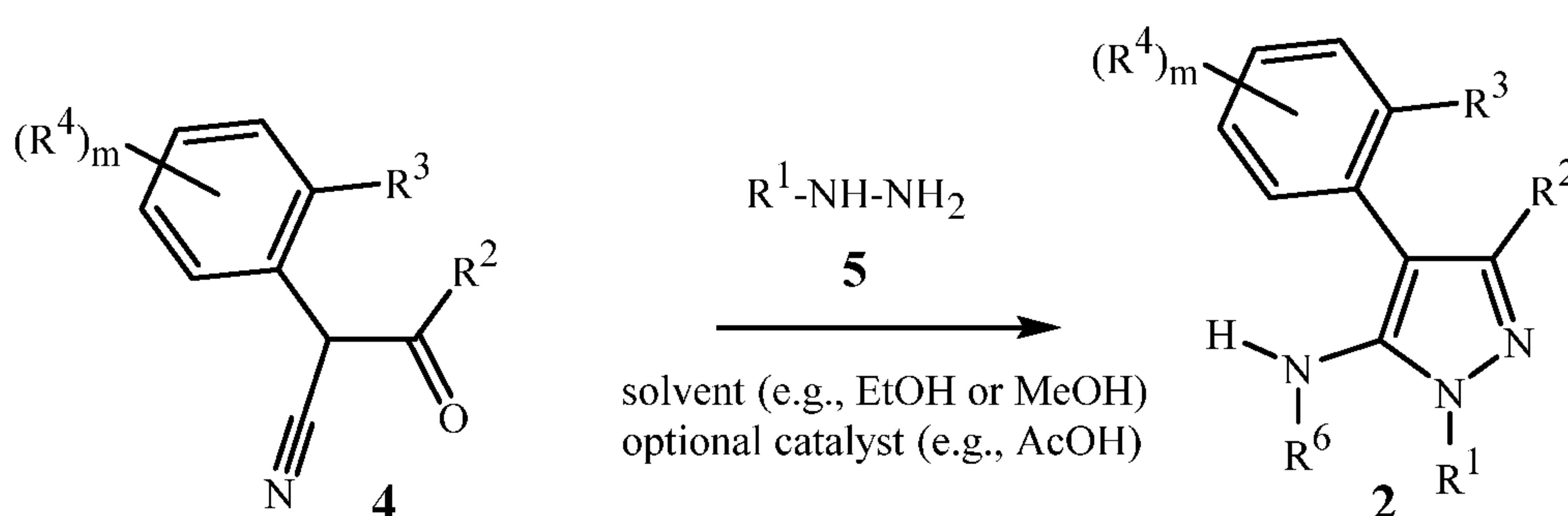
Scheme 2
