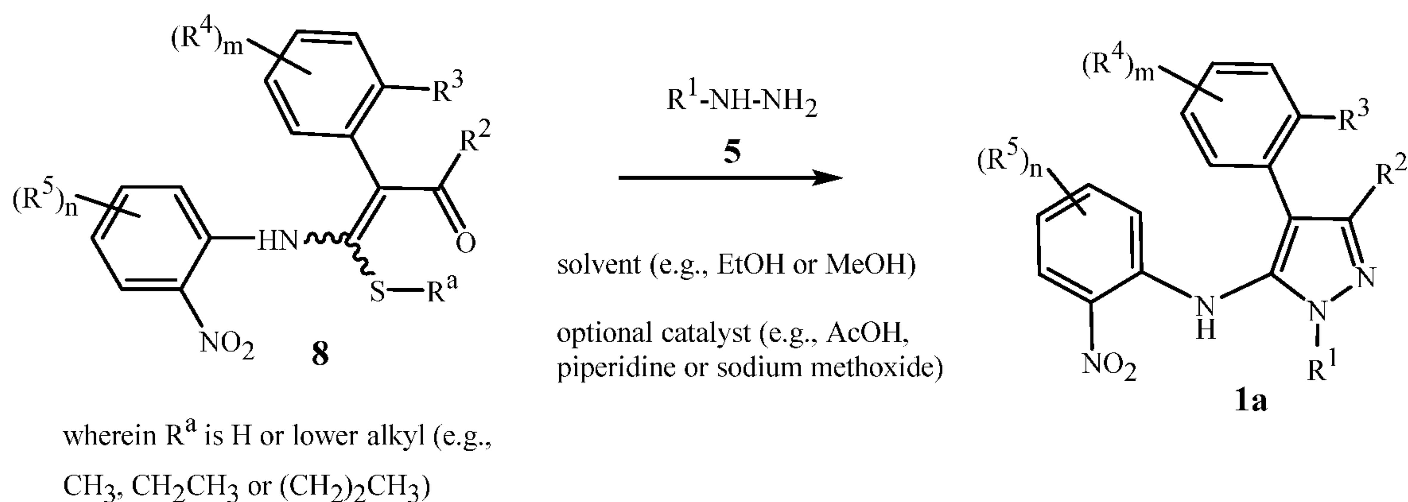
Scheme 4
