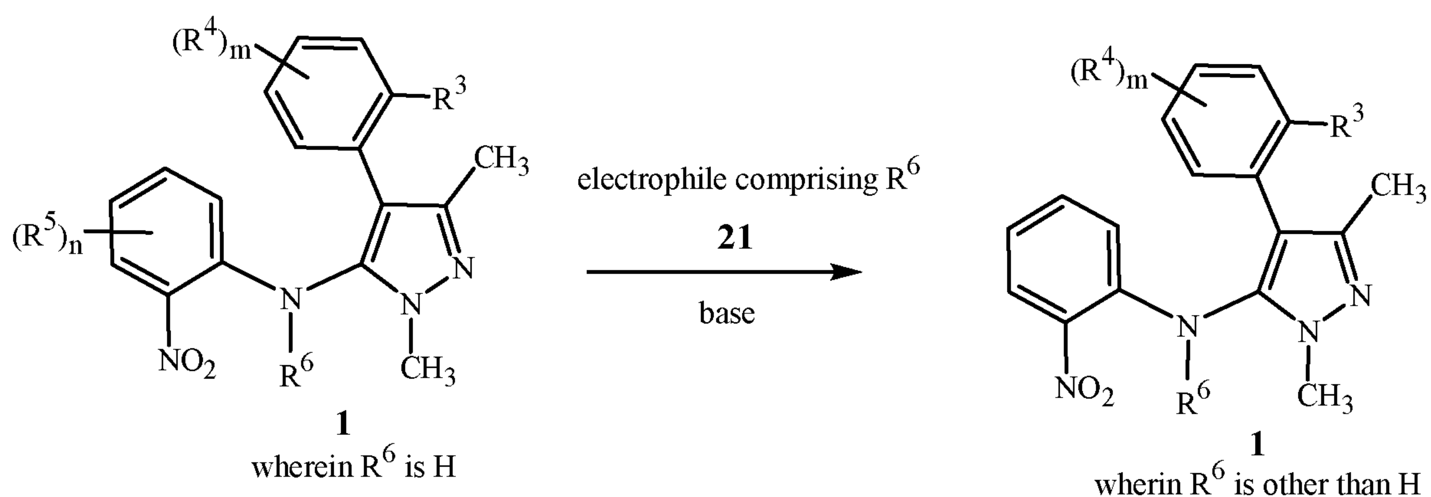
Scheme 12
