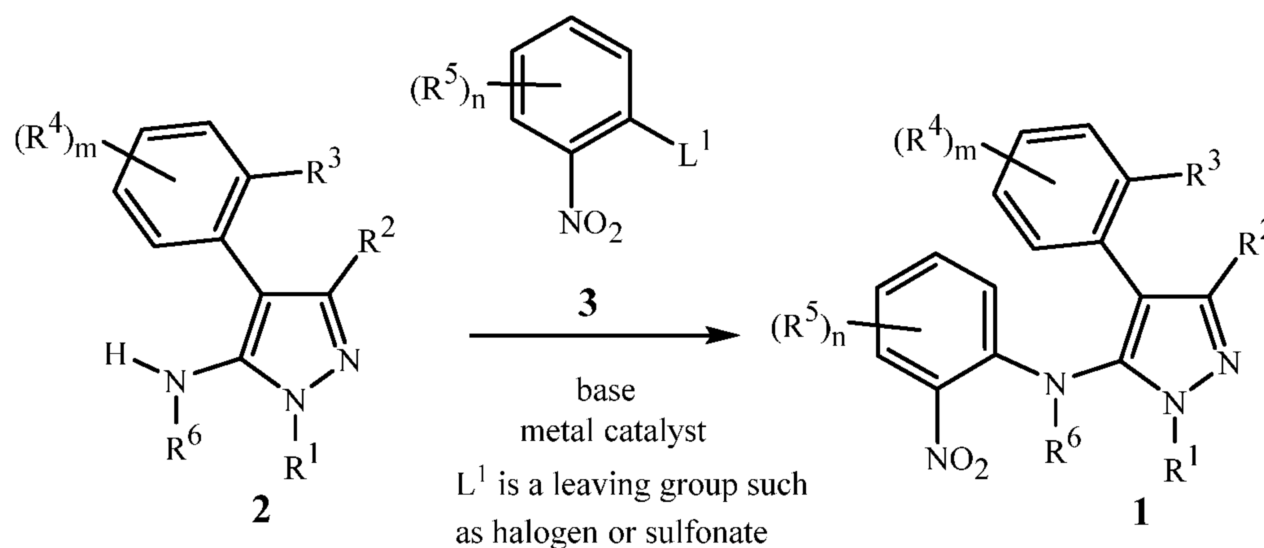
Scheme 1
