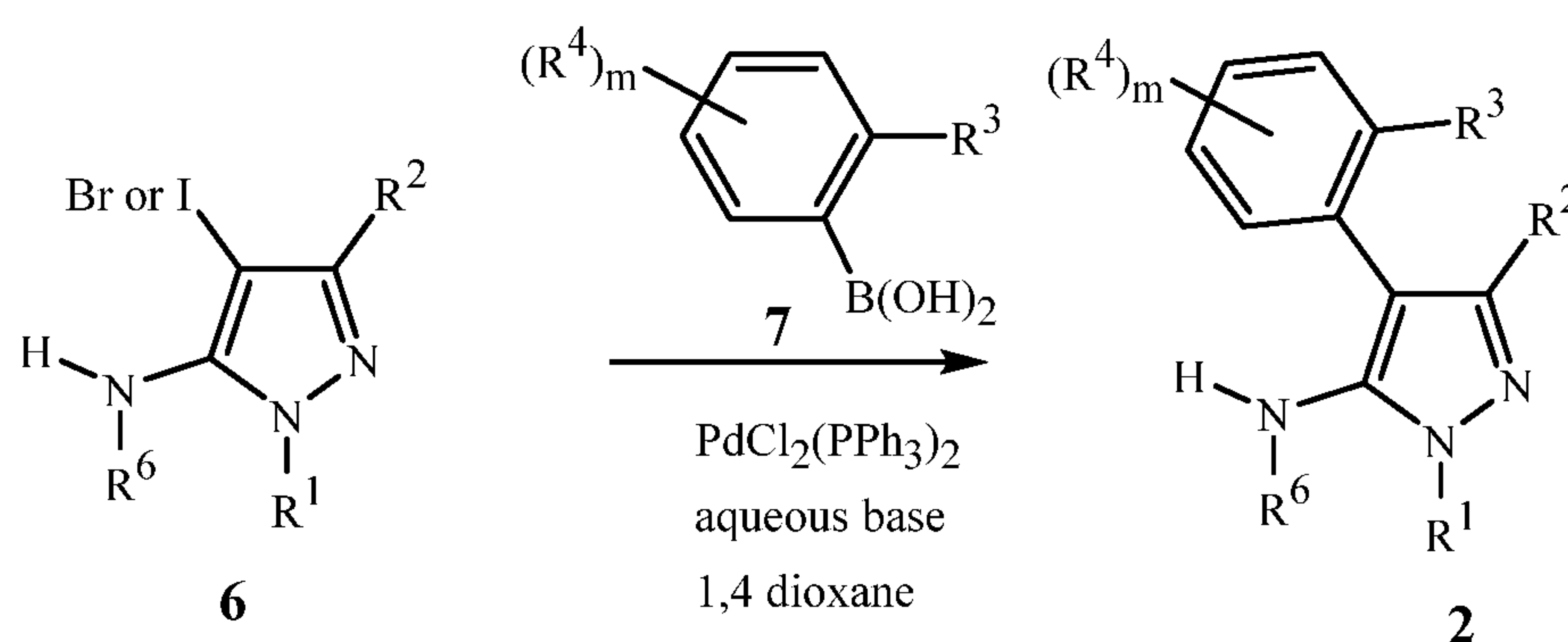
Scheme 3
