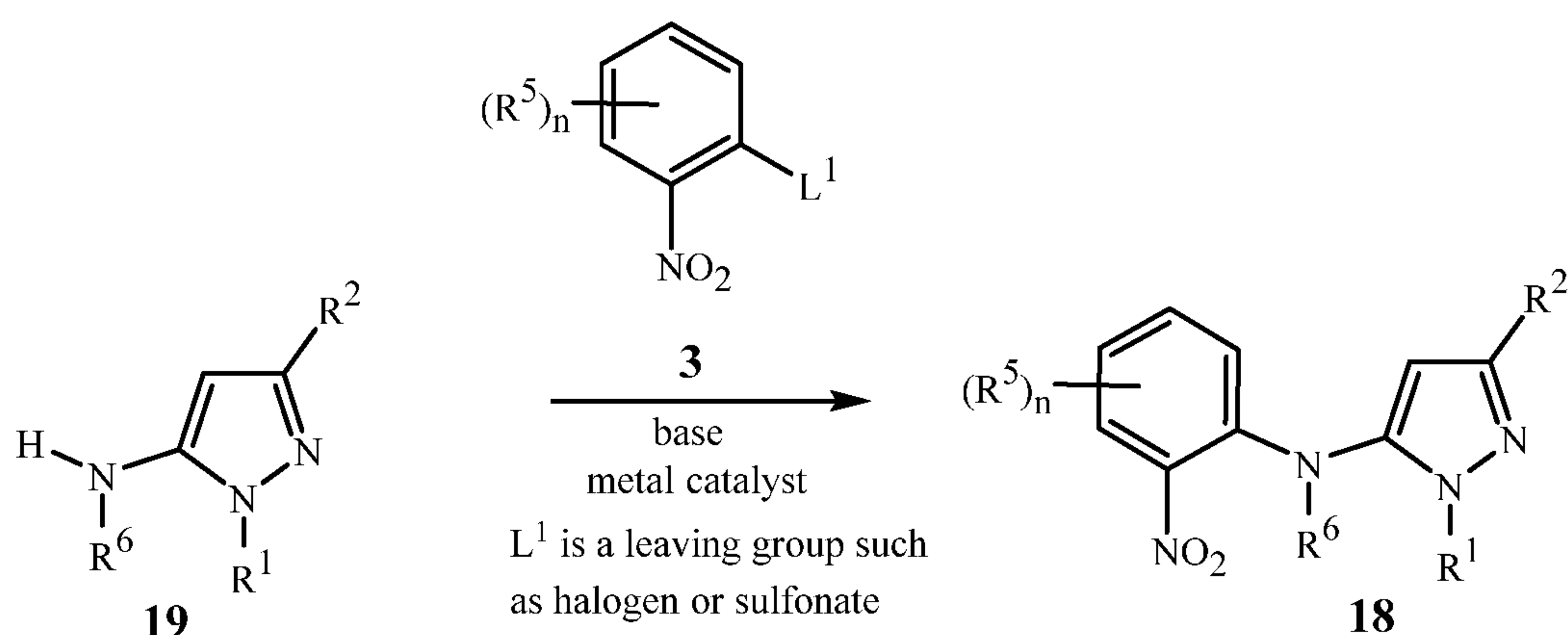
Scheme 10
