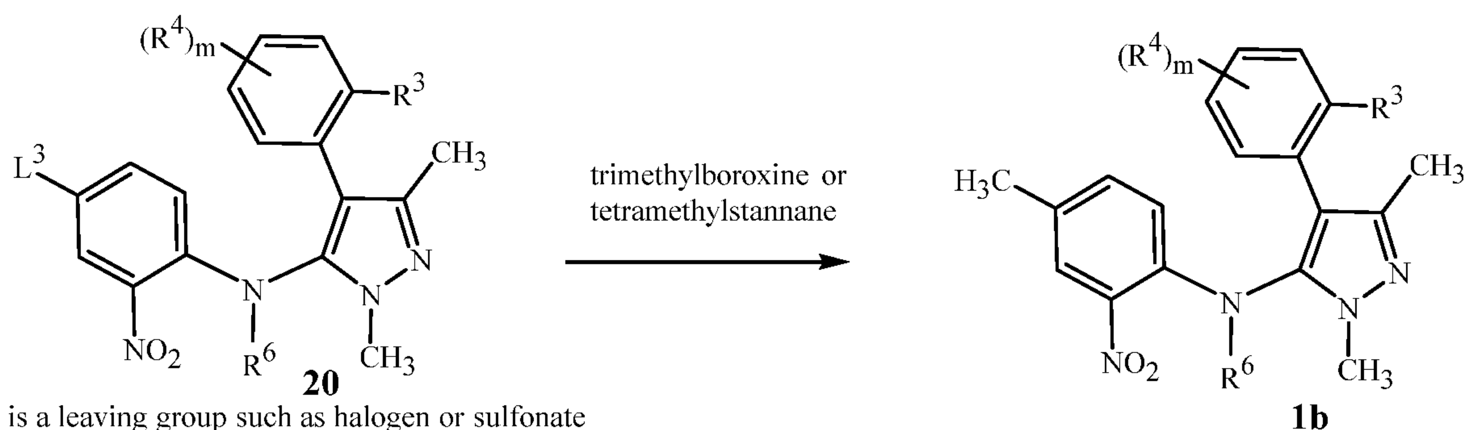
Scheme 11
